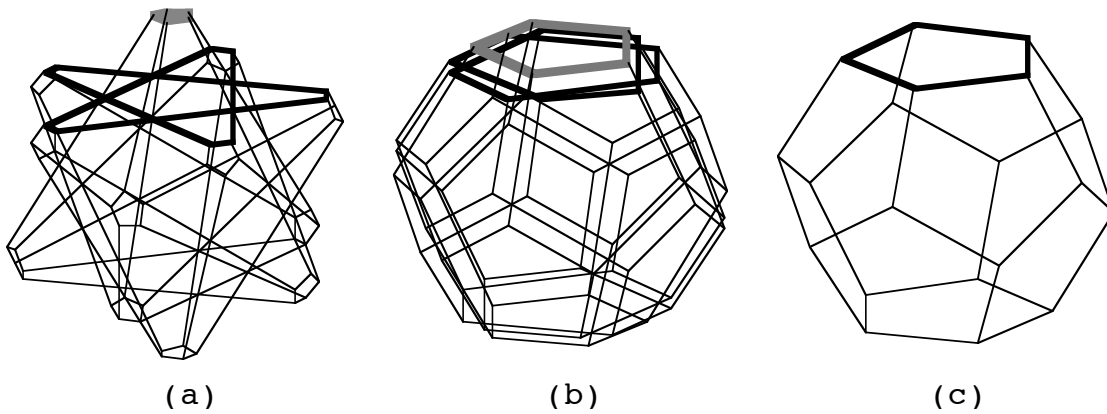
Figure 6. An example of the new approach to polyhedra: the truncation of the regular polyhedron \{5/2,5\} , Kepler's small stellated dodecahedron. (a) shows an early stage of the truncation; one of the pentagonal faces, and one of the decagonal faces are emphasized. (b) shows an almost complete truncation, illustrating the proximity of the emphasized pentagon and decagon. (c) is the complete truncation, in which each face of the "dodecahedron" represents one pentagon \{5\} and one decagon \{10/2\} . Each point that is a dodecahedral vertex represents three distinct vertices of the uniform polyhedron (5 \cdot 10/2 \cdot 10/2) , the complete truncation of \{5/2,5\} . From [12].
