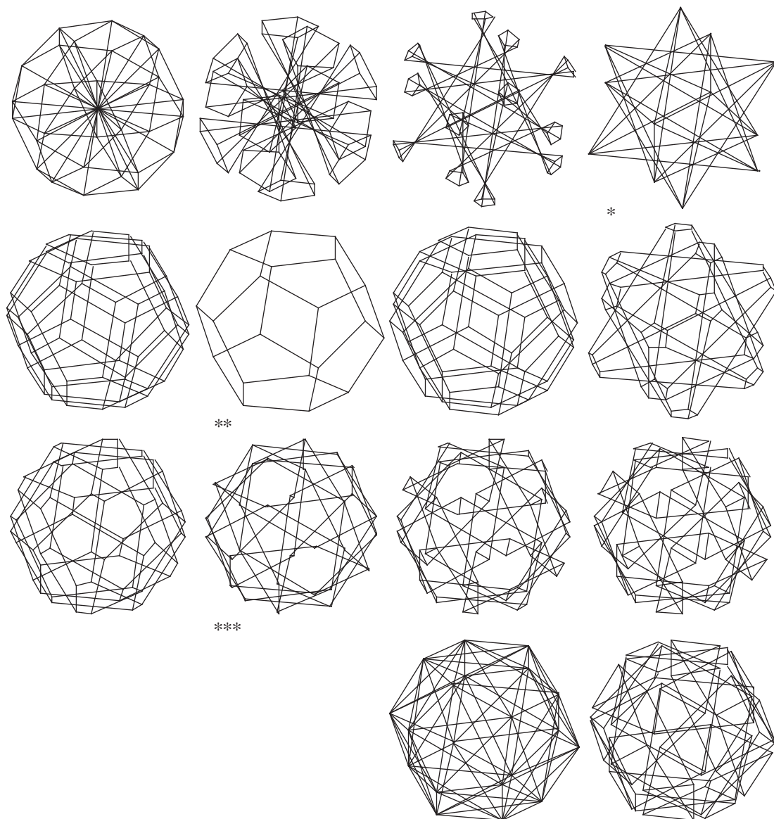
Fig. 13. A representation of a part of the continuous family of realizations of an abstract isogonal icositetrahedron (5.10.10), with 12 pentagonal and 12 decagonal faces. Each of the 60 vertices is incident with one pentagon and two decagons. The polyhedron is orientable, of genus 4. The realization marked by two asterisks is a “new” uniform polyhedron with symbol (5.10/2.10/2). The realizations marked by asterisks are isomeghetic (represented by the same point set) as well-known polyhedra: one asterisk and two asterisks indicate polyhedra isomeghetic with regular polyhedra (small stellated dodecahedron \{5/2, 5\} and dodecahedron \{5, 3\} , respectively). The polyhedron marked by three asterisks is isomeghetic with the uniform dodecadodecahedron (5.5/2.5.5/2). The polyhedra between those with one and two asterisks are isomeghetic with truncations of the small stellated dodecahedron.
