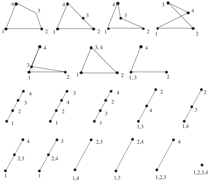
Fig. 5. Examples of different types of quadrangles, with vertices labeled 1, 2, 3, 4 for clarity. The quadrangles in the first two rows are full-dimensional , the ones in the last two rows are sub-dimensional . The last one is the trivial quadrangle. It should be noted that the traditional approach admits only three types of quadrangles (convex, simple but nonconvex, and self-crossing). In our interpretation there are 18 different types! The number increases even more if orientation is taken into account.
