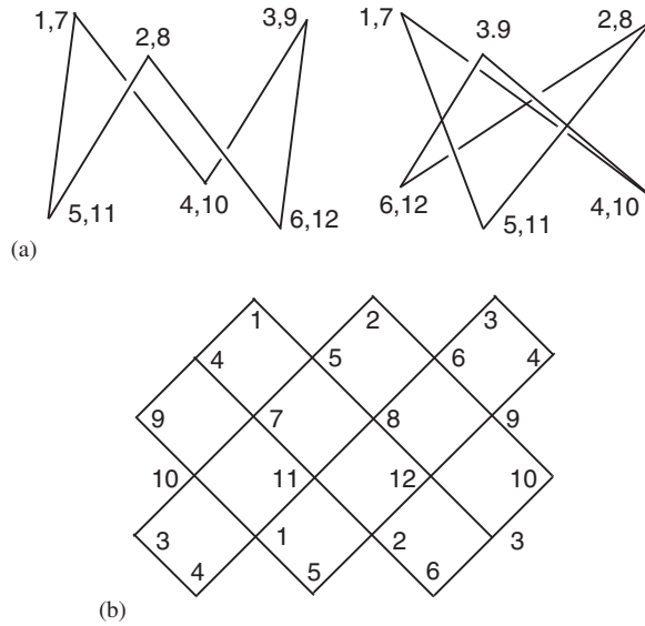
Fig. 11. (a) Two fully transitive realizations of the abstract polyhedron presented as a map (cell complex) in (b). The structure of these polyhedra is most easily visible from that map. In both realizations the faces are the full-dimensional “V-quadrangles”, exemplified by the last quadrangle in the second row of Fig. 5. Both are self-polar realizations of the underlying self-dual abstract polyhedron.
