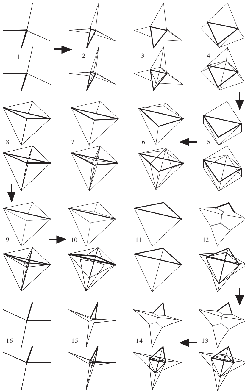
Fig. 14. A representation of the continuous family of realizations of an abstract isohedral triakis tetrahedron [3.6.6], with four 3-valent and four 6-valent vertices. Each polyhedron is shown in a “cardboard model” view, as well as in a skeletal view. All polyhedra are presented as inscribed in the same sphere. The first and last are approximations to the limit polyhedron, which is isomegnetic to four equiinclined segments. Polyhedra #4 and #11 have equilateral triangles as faces. (The latter was dismissed from the enumeration of isohedral deltahedra by Shephard [58] with the statement “. . . the construction leads to a set of twelve equilateral triangles which coincide in four sets of three”; this dismissal completely disregards the combinatorial structure of the polyhedron.) Polyhedron #5 is isomegnetic with the cube, and #6 is the Catalan polyhedron [3.6.6] (polar of the uniform polyhedron (3.6.6)). The faces of #8 coincide in pairs; this polyhedron marks the boundary between the acoptic representatives and those with self-intersections in the “cardboard model”. The grey segments mark these self-intersections.
