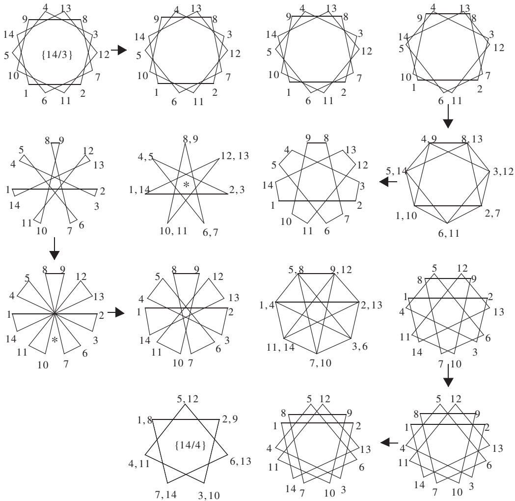
Fig. 9. A representation of a continuous family of isogonal 14-gons, that starts with the regular \{14/3\} and ends with \{14/4\} . The rotation number and the winding number w.r.t. the center (the “density” of the polygon) are equal before the polygon marked by the first asterisk * and after the one marked by the second asterisk, but differ for polygons between these two. The rotation number is not defined for the polygon marked by the first asterisk, and the winding number is undefined for the polygon marked by the second asterisk.
