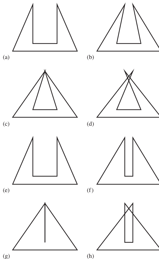
Fig. 4. Obvious continuous deformations of the hexagon in (a) and (e) lead to intermediate objects (c) and (g) that could not be considered polygons if the approach of Poincot is adopted.
