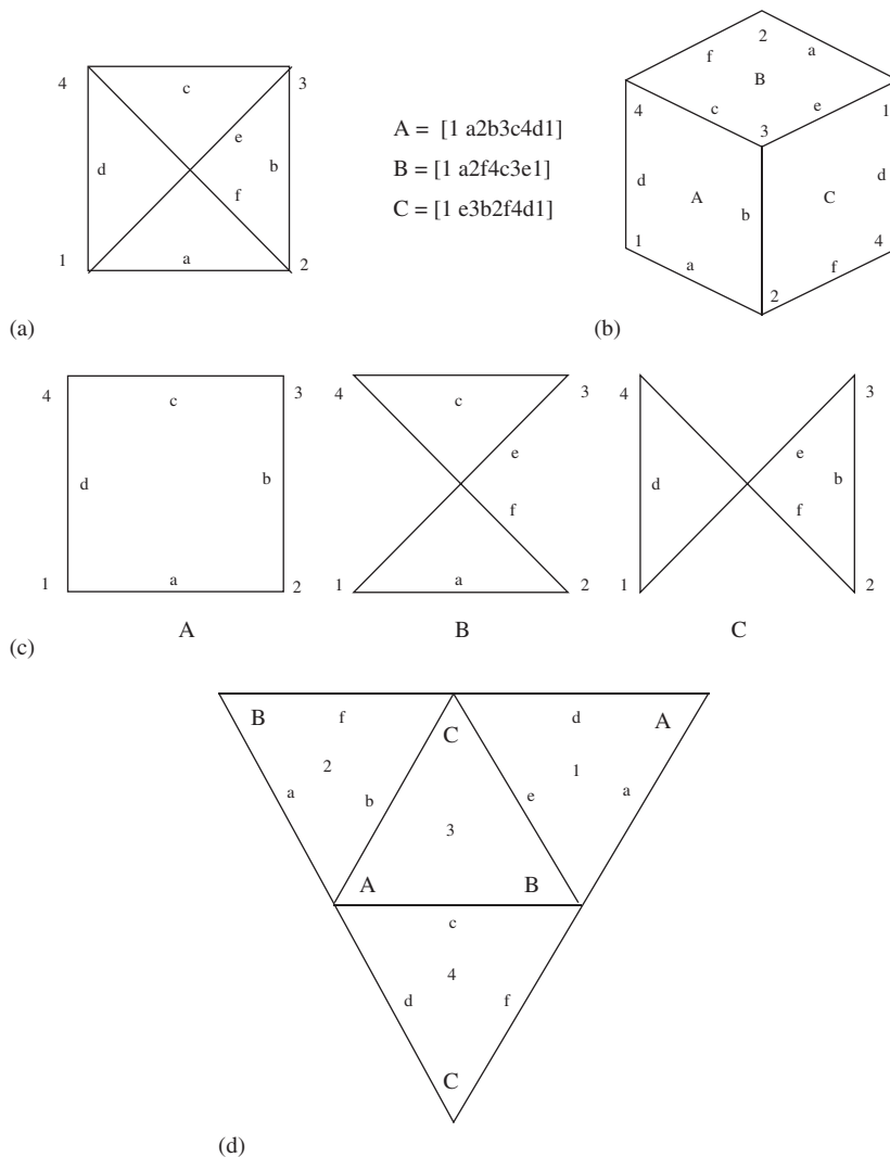
Fig. 10. (a) An isogonal sub-dimensional realization of a nonorientable abstract polyhedron (shown in (b) by its map) with the least possible number of faces. The three faces of the realization are shown separately in (c). Part (d) shows a map of the dual abstract polyhedron. It also indicates how the polyhedron can be realized: by folding the three outer triangles over the middle one, and identifying the appropriate edges. Thus, the polyhedron is isomeghetic (that is, looks like ) a triangle. However, each edge of the triangle is replaced by a pair of edges between the same vertices but incident with four different faces.
