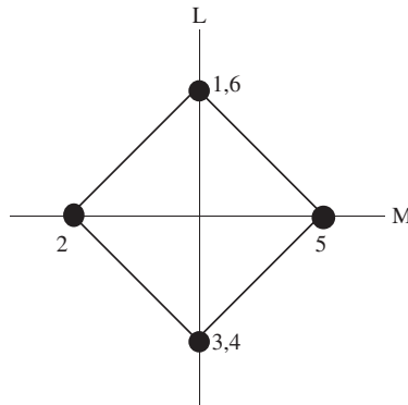
Fig. 6. Illustrations of the symmetries of the geometric hexagon with vertices 1, 2, 3, 4, 5, 6.
