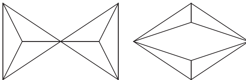
Fig. 1. These graphs (or complexes) are admitted as graphs of convex polyhedra by the definitions in all versions of Lyusternik's presentation of Steinitz's theorem.
