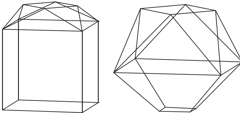
Fig. 2. A convex polyhedron, and its canonical representative obtained by the Hart algorithm [34].
