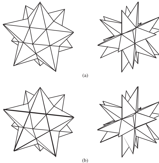
Fig. 3. Kepler's two "starshaped" regular polyhedra, presented in "cardboard model" views. In (b) one of the pentagrammatic faces of each polyhedron is emphasized.
