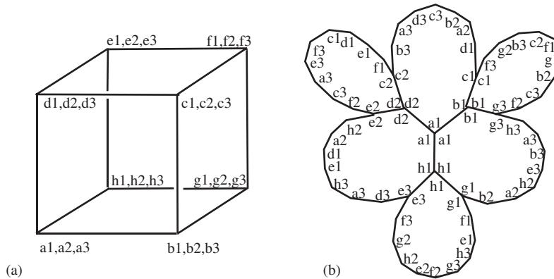
Fig. 12. (a) A regular polyhedron with Schläfli symbol \{12, 3\} , which realizes the abstract polyhedron given by the map in (b). The map is listed as #36.13 in Wilson’s catalog [65]. The polyhedron results from “vertex tripling” of the cube; this operation and related ones are described in [26].
