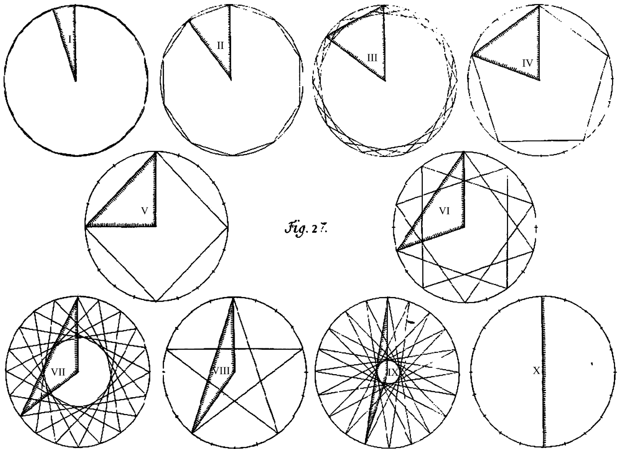
Fig. 8. A representation of the different regular 20-gons, presented by Meister to illustrate the existence of regular polygons \{n/d\} in cases n and d are not relatively prime.
