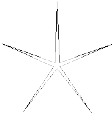
Figure 1. Any right prism over this starshaped polygon has no net.
