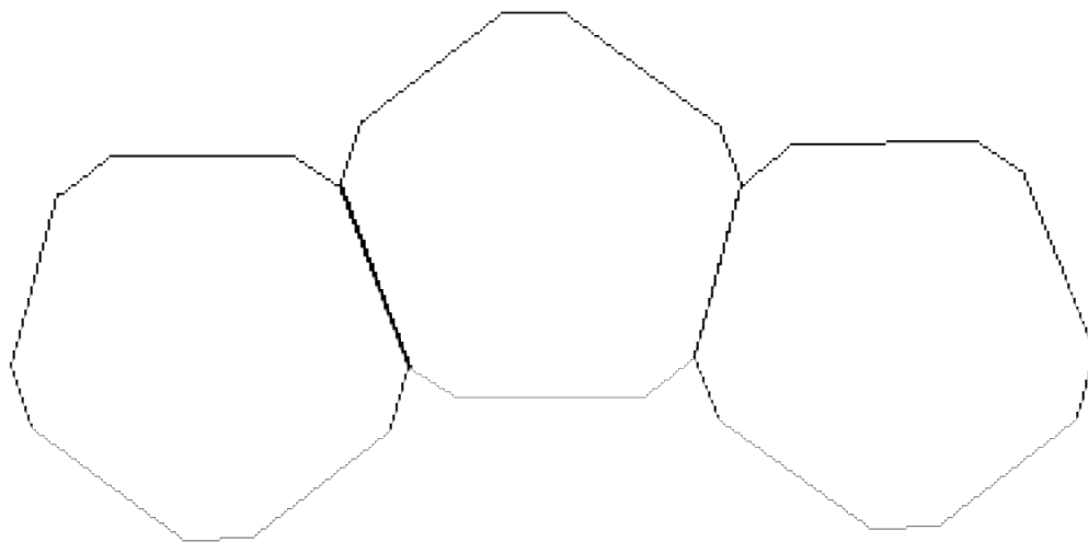
Figure 6. The only way one decagon can be adjacent to two other decagons.
