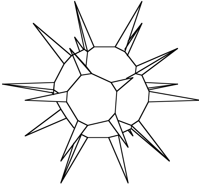
Figure 2. A polyhedron with no net, with convex faces and homeomorphic to the sphere.
