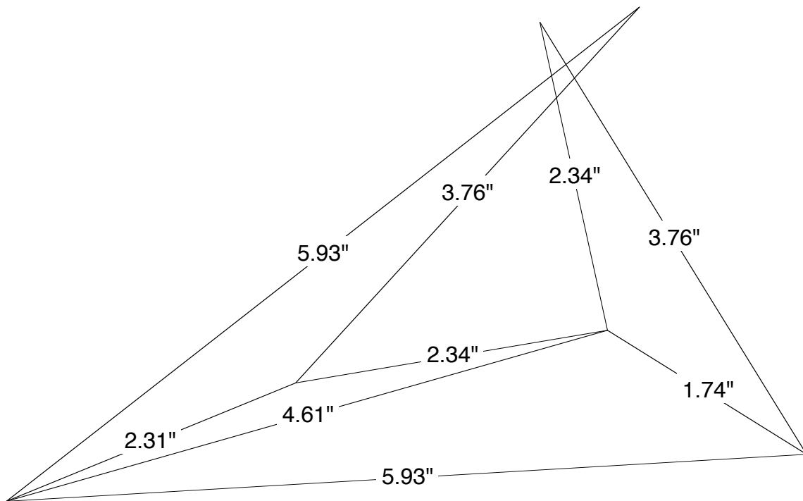
Figure 7. A would-be net for Namiki's tetrahedron.
