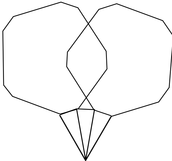
Figure 3. One type of obstruction to forming a net for the spiky dodecahedron.
