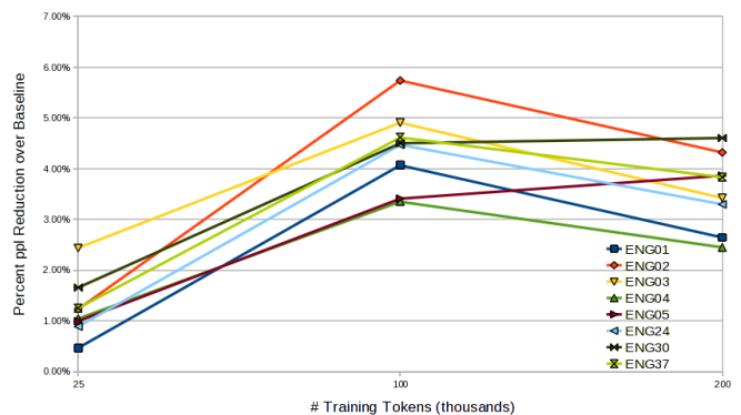
Figure 2: Percent perplexity reduction over baseline by topic and training set size.
