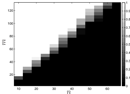
Figure 4: Performance of the recovery program minimizing \max\{\frac{\text{tr}(\mathbf{X})}{\text{tr}(\mathbf{X}_0)}, \frac{\|\mathbf{X}\|_{1,2}}{\|\mathbf{X}_0\|_{1,2}}\} with a PSD constraint. As predicted by Theorem 3.3, number of required measurements increases linearly with nr .
