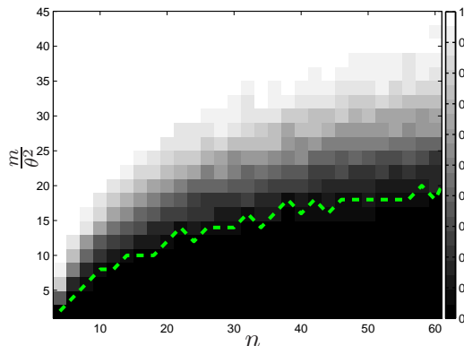
Figure 5: Performance of the recovery program minimizing \max\{\frac{\text{tr}(\mathbf{X})}{\text{tr}(\mathbf{X}_0)}, \frac{\|\mathbf{X}\|_1}{\|\mathbf{X}_0\|_1}\} with a PSD constraint. The matrix is rank 1, PSD and supported over an 8 \times 8 submatrix. Plot shows \frac{m}{\theta^2} versus n to better illustrate the saturation behavior predicted as \Omega(\min\{k^2, nr\}) by Theorem 3.3.
