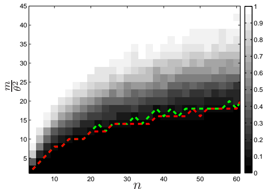
Figure 7: 90% frequency of failure where the threshold of recovery is 10^{-4} for the green and 0.05 for the red curve. Objective function is \max\{\frac{\text{tr}(\mathbf{X})}{\text{tr}(\mathbf{X}_0)}, \frac{\|\mathbf{X}\|_1}{\|\mathbf{X}_0\|_1}\} .
