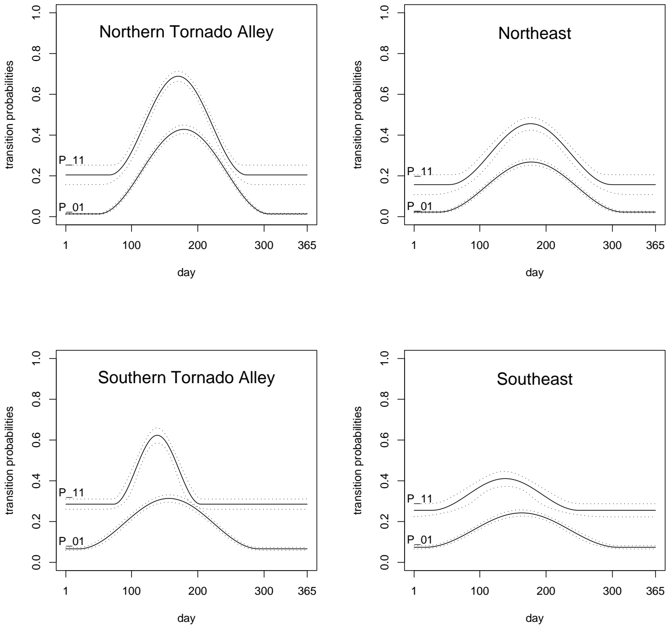
Figure 4: The MLE of the transition probabilities in the four regions and point-wise, i.e. daywise, 95%-confidence intervals.
