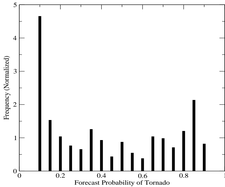
Figure 6: The discrimination (top) and the refinement diagram (bottom) for the model forecasts for the year 1979 over the entire U.S. In the top diagram, “0” indicates non-occurrence, and “1” indicates occurrence of a tornado.
