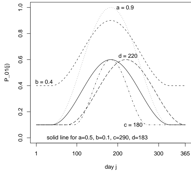
Figure 3: Illustration of the parameterization of the transition probabilities. Parameter b is a baseline—its variation shifts the curve vertically; d is the peak day—its change shifts the curve horizontally; c determines the length of the deviation from the baseline; a scales the deviation’s magnitude.
