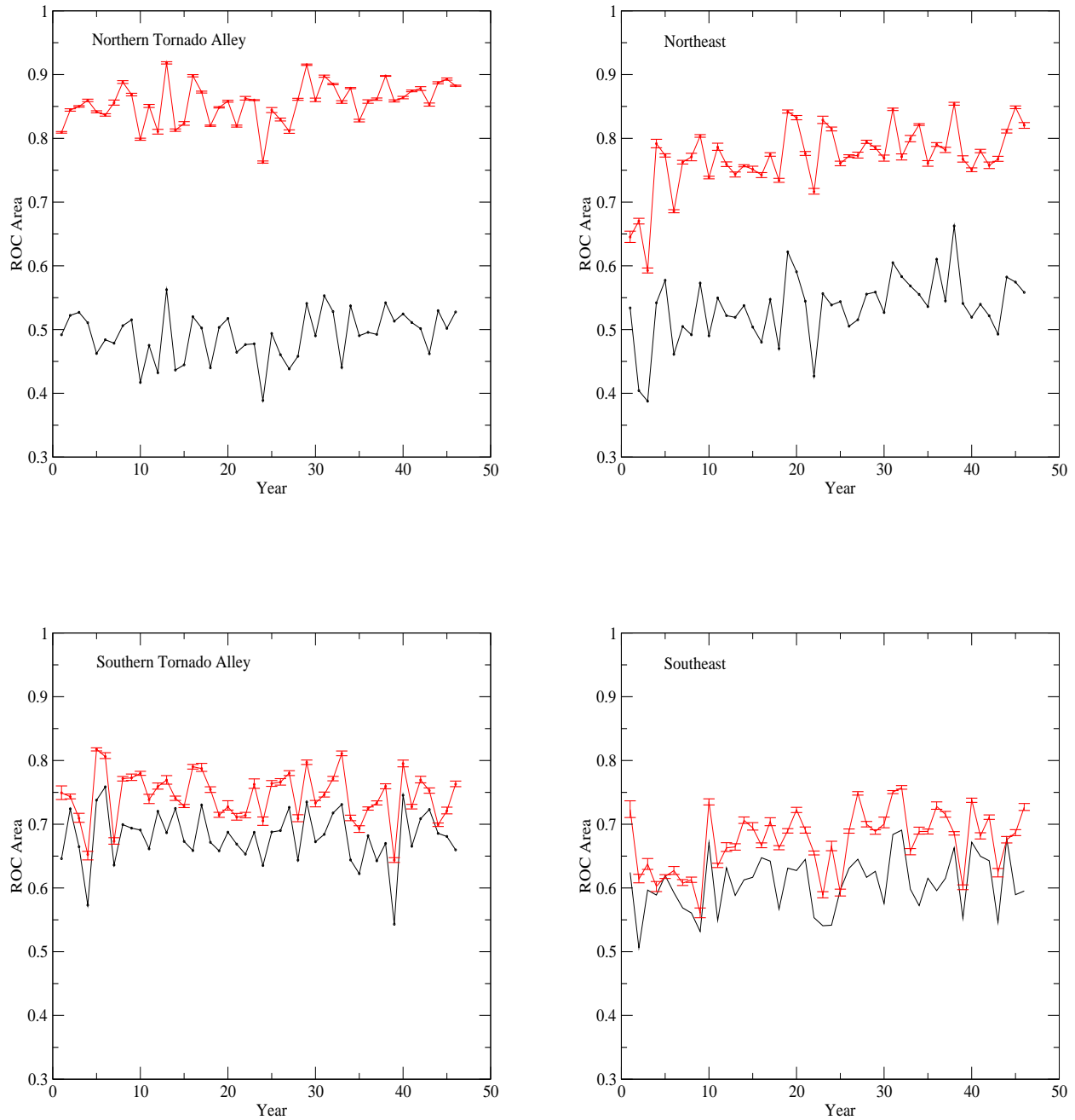
Figure 8: The performance of the model for each of the 46 validation years and the four geographic regions. The curve with error bars showing yearwise 95%-confidence intervals corresponds to the model, while the remaining curve refers to climatology. The graphs are laid out in relation to their corresponding geographic locations.
