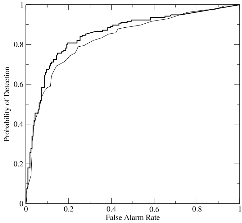
Figure 7: The ROC diagram for the entire U.S. and the year 1979 (thick curve). The thin curve corresponds to climatological forecasts.
