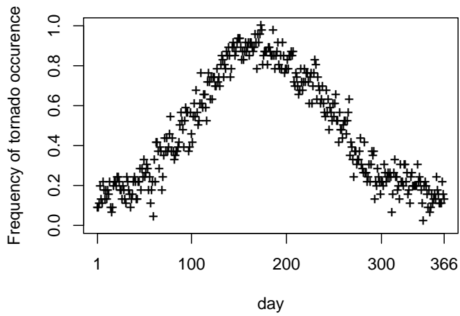
Figure 1: Number of days with tornado occurrence in the entire U.S. in a given year (top), and frequency of tornadic activity in the entire U.S. on a given day.
