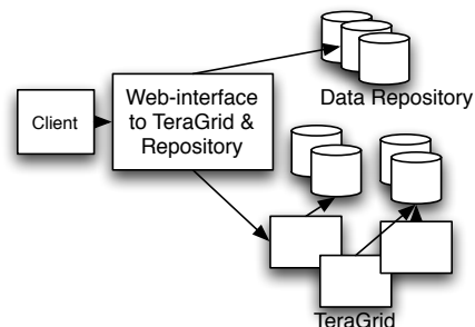
Figure 1: System Architecture
