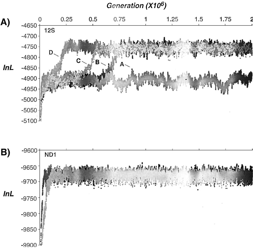
FIGURE 4. (a) Burn-in plots of the separate 12S Bayesian analyses. Letters A–D represent four independent analyses (each involving four incrementally heated Markov chains) beginning with random starting trees. (b) Burn-in plots of the separate ND1 Bayesian analyses. The results of the two independent analyses are superimposed, illustrating that the log-likelihood scores converged on similar values.
