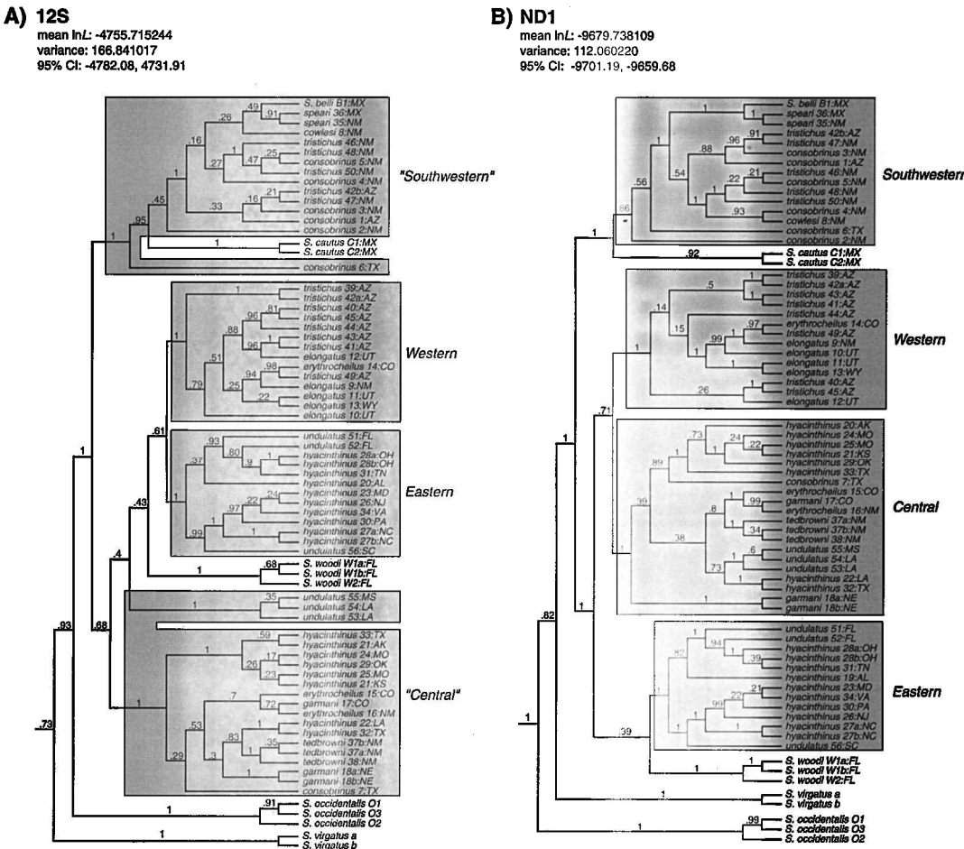
FIGURE 5. The 50% majority rule consensus trees from the separate Bayesian analyses of the 12S (a) and ND1 (b) data. Numbers on nodes represent posterior probability values.
