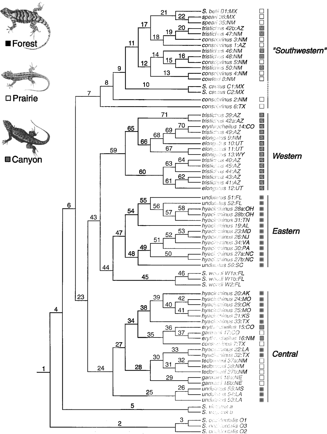
FIGURE 10. Evolution of ecomorphs within the Sceloporus undulatus species group. Boxes filled with black, white, or gray indicate habitat types as shown by the inset drawings. Support values (MP, ML, and Bayesian) for the numbered nodes are provided in Appendix 2.
