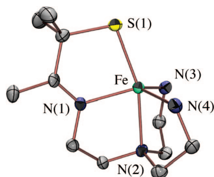
FIGURE 4. ORTEP diagram of thiolate-ligated, biomimetic superoxide reducing catalyst [\text{Fe}^{\text{II}}(\text{S}^{\text{Me}_2}\text{N}_4(\text{tren}))]^+ ( 2 ) synthesized by Jason Shearer, a graduate student in the Kovacs lab.
