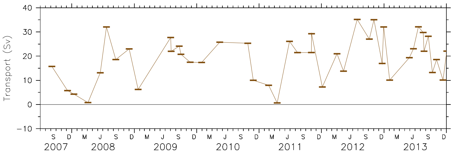
Solomon Sea glider transport: raw data values
