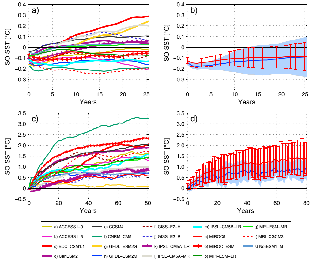
Figure 2. Left: Response functions of the annually averaged SO SST ( 55^{\circ} S to 70^{\circ} S) in CMIP5 models to a 1 standard deviation step increase in the (a) December–May SAM index and to an (c) abrupt \text{CO}_2 quadrupling (smoothed with a 20 year running mean). Different colors and line styles indicate individual model responses; right: Subset of the step-response functions to (b) SAM and (d) GHG forcing that favor multidecadal SO cooling (section 3.2) induced by the observed SAM trend as estimated from ERA-Interim (blue) and HadSLP2r (red) data. The thick blue/red lines show the mean response of the subset. Blue shading/red bars show one standard deviation for each subset.
