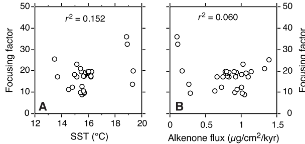
Fig. 2. Sediment focusing factors (14) are uncorrelated to both (A) alkenone-derived SST and (B) ^{230}\text{Th} -normalized alkenone fluxes, indicating that changing horizontal transport of fine-grained sediment did not cause the observed down-core variations in alkenone-derived temperatures.
