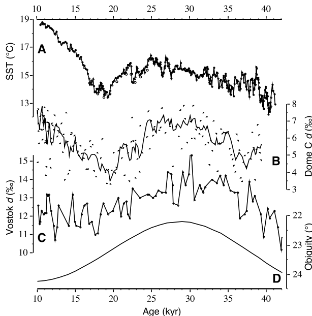
Fig. 3. (A) Cape Basin SSTs on the GISP2 time scale from Stoner et al. (15). (B) Deuterium excess, d , in the Dome C ice core (26). The solid line is a five-point running mean of the data. (C) Deuterium excess in the Vostok ice core (27) on the GRIP time scale (3, 50). (D) Obliquity variation through time with a reversed y-axis scale.
