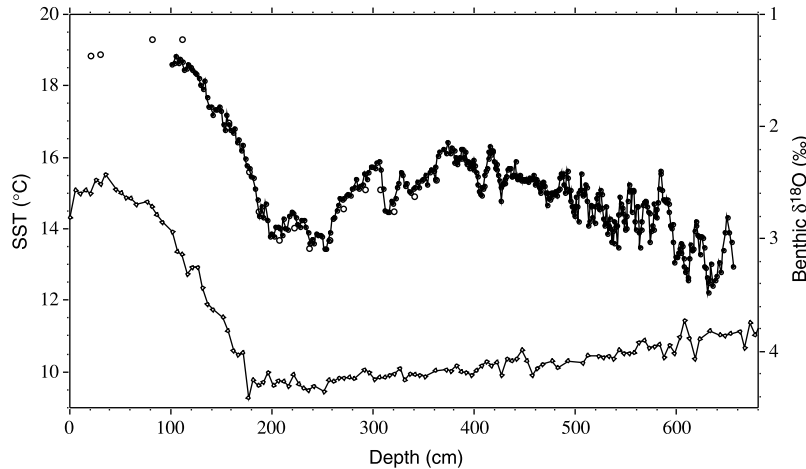
Fig. 1. SSTs derived from alkenone unsaturation ratios (7, 9) (circles; top trace) in core TN057-21-PC2. A benthic oxygen isotope stratigraphy (diamonds; bottom trace) was previously derived from the benthic foraminifera, Cibicides spp. (4). Open circles represent measurements performed on independently sampled sediment and, in the 100- to 380-cm interval, provide an indication of the reproducibility of the procedure. Alkenone analyses were performed on adjacent 1-cm samples from 380 to 630 cm, and on every other 1-cm interval from 100 to 380 cm and 630 to 656 cm, giving a temporal resolution of 60 and 120 years, respectively.
