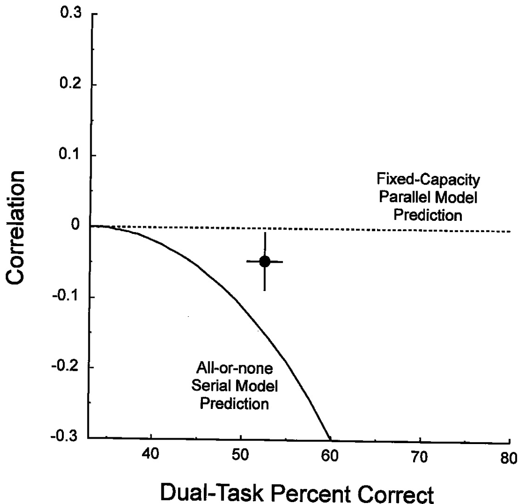
Figure 5. Predicted and observed correlations plotted as a function of dual-task percent correct. The dashed line represents predicted zero correlations under crowding theory and the fixed-capacity parallel model. The curve represents predicted negative correlations under the all-or-none serial model. The closed circle represents the average correlation, and error bars represent the standard error of the mean.
