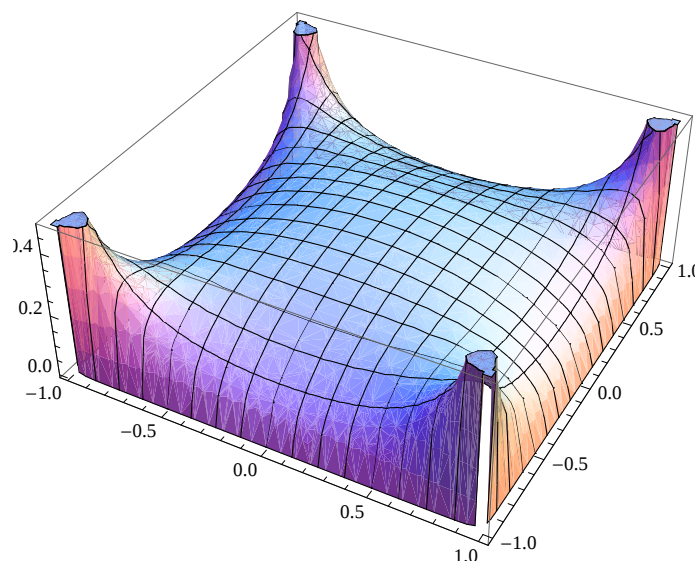
Figure 13. Joint density f(u, v) of (U, V) in (40).
