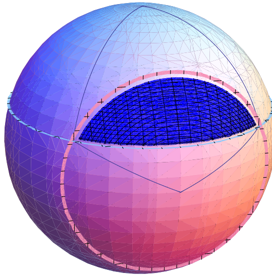
Figure 5. Intersection of two spherical caps, circular representation (modified from Tovchigrechko and Vakser [7]).
