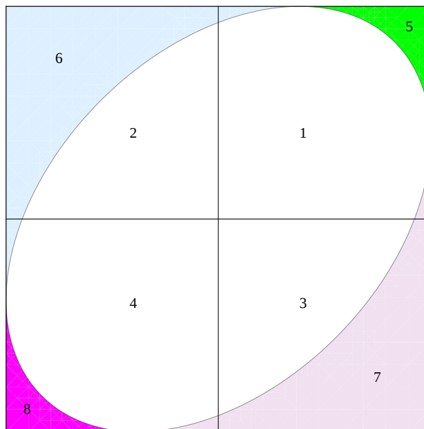
Figure 9. Eight regions R_1(\gamma) - R_8(\gamma) for an elliptical copula (with \gamma = \pi/8 ).
