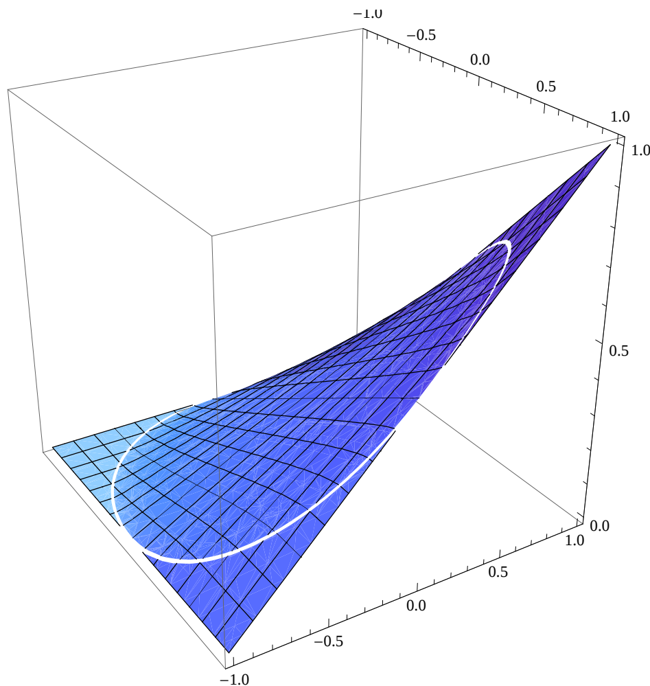
Figure 6. The copula (17) in Theorem 3.1.
