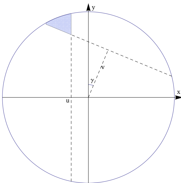
Figure 11. The region [X < u, X \sin(\gamma) + Y \cos(\gamma) > v] for Case 2 (with \gamma = \pi/8 ).
