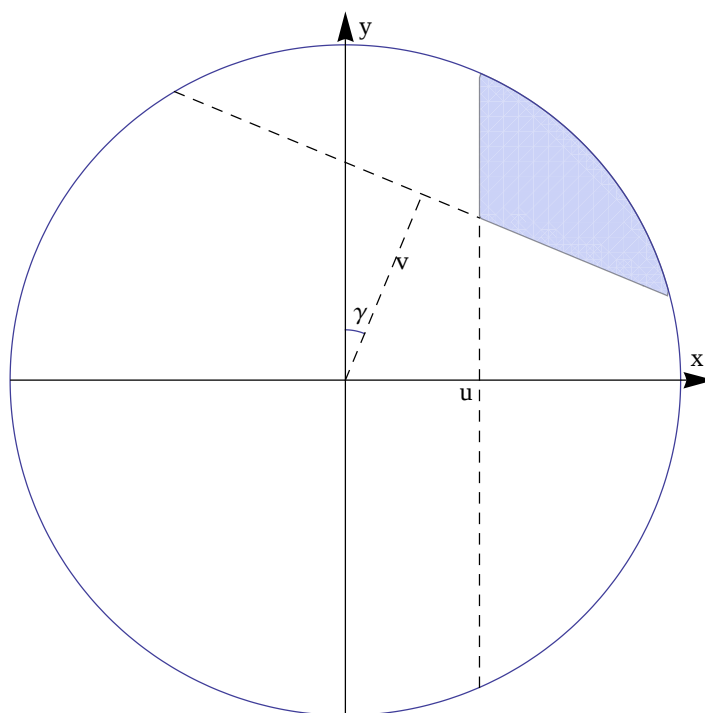
Figure 10. The region [X > u, X \sin(\gamma) + Y \cos(\gamma) > v] for Case 1 (with \gamma = \pi/8 ).
