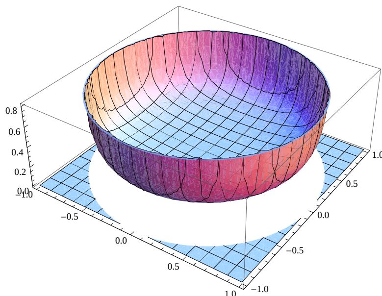
Figure 2. Circularly symmetric bivariate density (6) on B_2 .
