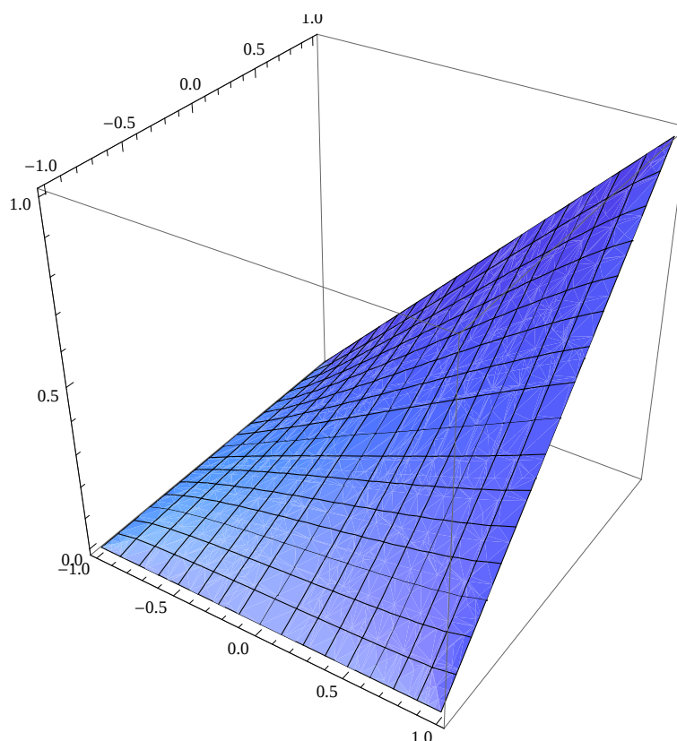
Figure 15. Nonlinear transformation copula F(u, v) in Theorem 6.1.
