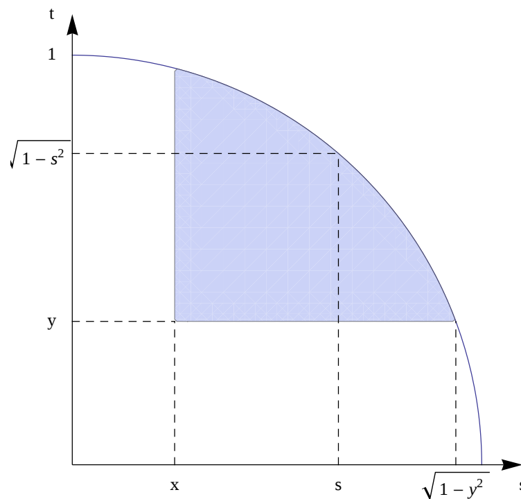
Figure 3. Region of integration, 2-dimensional case.
