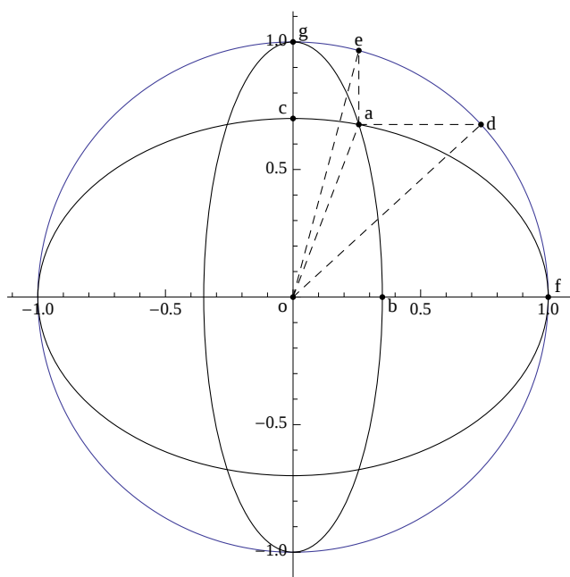
Figure 14. Integration regions for Lemma 6.2.
