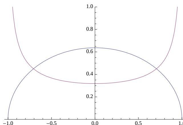
Figure 1. The densities (3) (lower, blue) and (4) (upper, purple).
