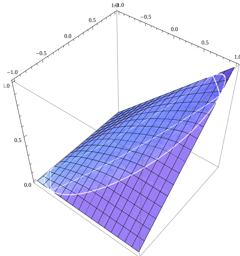
Figure 12. The copula F_\gamma(u, v) in (38) (with \gamma = \pi/4 ).
