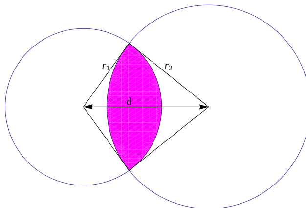
Figure 5. Intersection of two spherical caps, circular representation (modified from Tovchigrechko and Vakser [7]).
