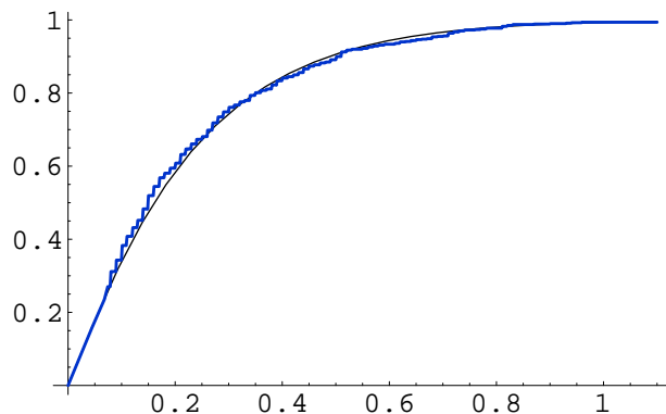
Figure 2: Empirical distribution function (blue) and fitted Weibull c.d.f. (via MLE).
