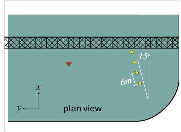
Fig. 4. Plan view of the scaled model test locations in the Carderock Wave Basin. Red triangle is the scaled model of the Wind Float platform. Yellow circles are the SWIFT buoys. The wave-maker produced waves propagating in the +x direction.
