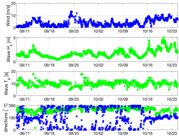
Fig. 8. Wind (blue) and wave (green) conditions during the Portugal deployment at the WindFloat® Atlantic deployment in September and October of 2022.
