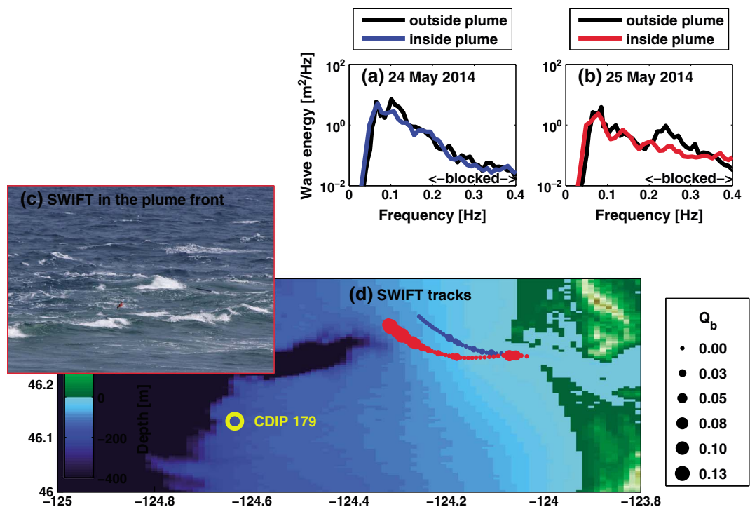
Figure 1. Wave energy spectral density versus frequency for (a) 24 and (b) 25 May 2014. Red and blue lines are SWIFT measurements within the plume, and black lines are CDIP measurements outside of the plume. The frequencies at which waves are expected to break against the plume currents are shown with the annotation “blocked.” (c) Photo of a SWIFT in the breakers at the offshore front. Photo taken by Chris Bassett on 28 May 2014, which was similar to 25 May 2014. (d) Tracks of SWIFT drifters as 5 min average positions, colored by day (blue is 24 May, and red is 25 May) and scaled by the fraction of breaking, Q_b .
