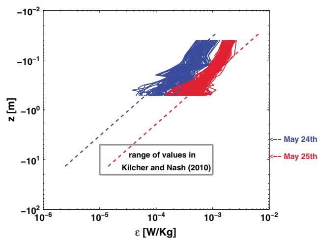
Figure 3. Observed (solid lines) and extrapolated (dashed lines) TKE dissipation rate profiles \epsilon(z) from 24 May (blue) and 25 May (red). Also shown are the plume depths in the frontal region for both days, as well as the range of values reported in Kilcher and Nash [2010] . Near-surface TKE dissipation rates are enhanced by wave breaking at the plume front on 25 May, and the values extrapolated down to plume depths are within the range of subsurface frontal values reported in Kilcher and Nash [2010] . Extrapolations use \alpha = 0.01 and \lambda = 1 in equation (6).
