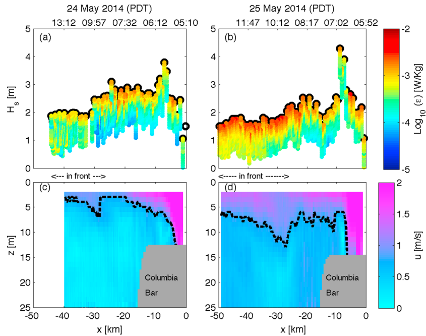
Figure 2. SWIFT results plotted versus local time and drift distance (along-track distance offshore from river mouth) for a case without wave breaking (24 May 2014) and a case with wave breaking (25 May 2014). Significant wave height and vertical profiles of near-surface turbulent dissipation rate (color scale) from the up-looking SWIFTs for (a) 24 and (b) 25 May. Current profiles (color scale) and level of maximum shear from the down-looking SWIFTs for (c) 24 and (d) 25 May. The SWIFTs are trapped in the plume front at approximately x < -30 km.
