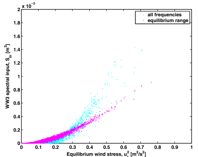
Figure 13. Spectral input terms from WAVEWATCH III versus equilibrium wind friction velocity squared. Cyan points are calculated from all frequencies in each wave spectrum. Magenta points are calculated from equilibrium frequencies (twice the peak frequency and above) in each wave spectrum.
