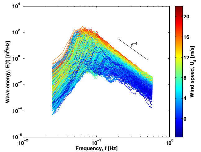
Figure 3. Hourly wave energy spectra from OWS-P buoy, colored by observed wind speed. The f^{-4} line indicates the theoretical spectral slope in the equilibrium range. Spectra in the equilibrium range are well sorted by observed wind speed.
