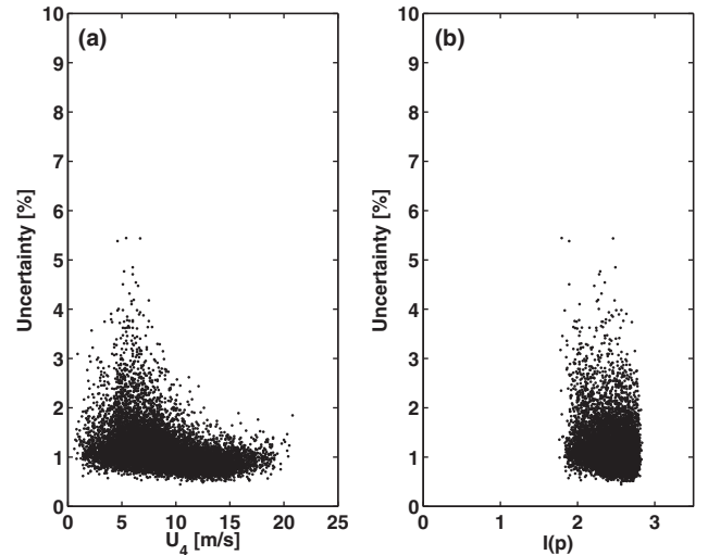
Figure 10. Relative uncertainty in equilibrium u_* as a function of (a) measured wind speed and (b) calculated directional function I(p) .
