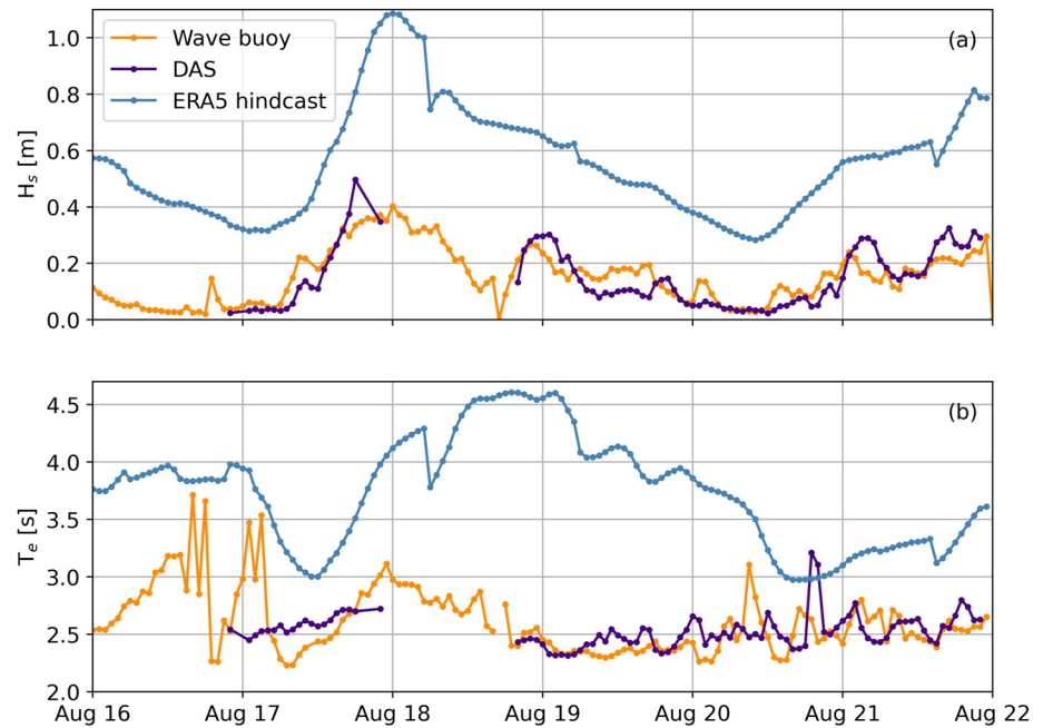
Figure 3. Time series of (a) significant wave height, (b) and energy-weighted wave period as measured by Surface Wave Instrument Float with Tracking wave buoy (orange), seafloor cable distributed acoustic sensing (DAS; purple; 16.2 km along-cable distance), and estimated by ERA5 hindcast model (blue). Buoy and ERA5 hindcast cover the period from August 16–22, 2022, while DAS observations are available for August 16 22:00–August 17 22:00 and August 18 20:00–August 21 22:00.
