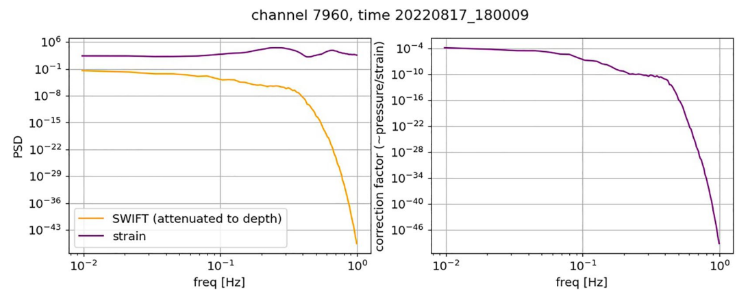
Figure A1. Example calculation of empirical correction factor for channel 7,960 (16.2 km along-cable distance) at 18:00 on 17 August 2022. Left panel shows power spectral density of raw distributed acoustic sensing strain-rate (purple) and inferred seafloor pressure from Surface Wave Instrument Float with Tracking (orange). Right panel shows the empirical correction factor calculated as a ratio of the PSDs.
