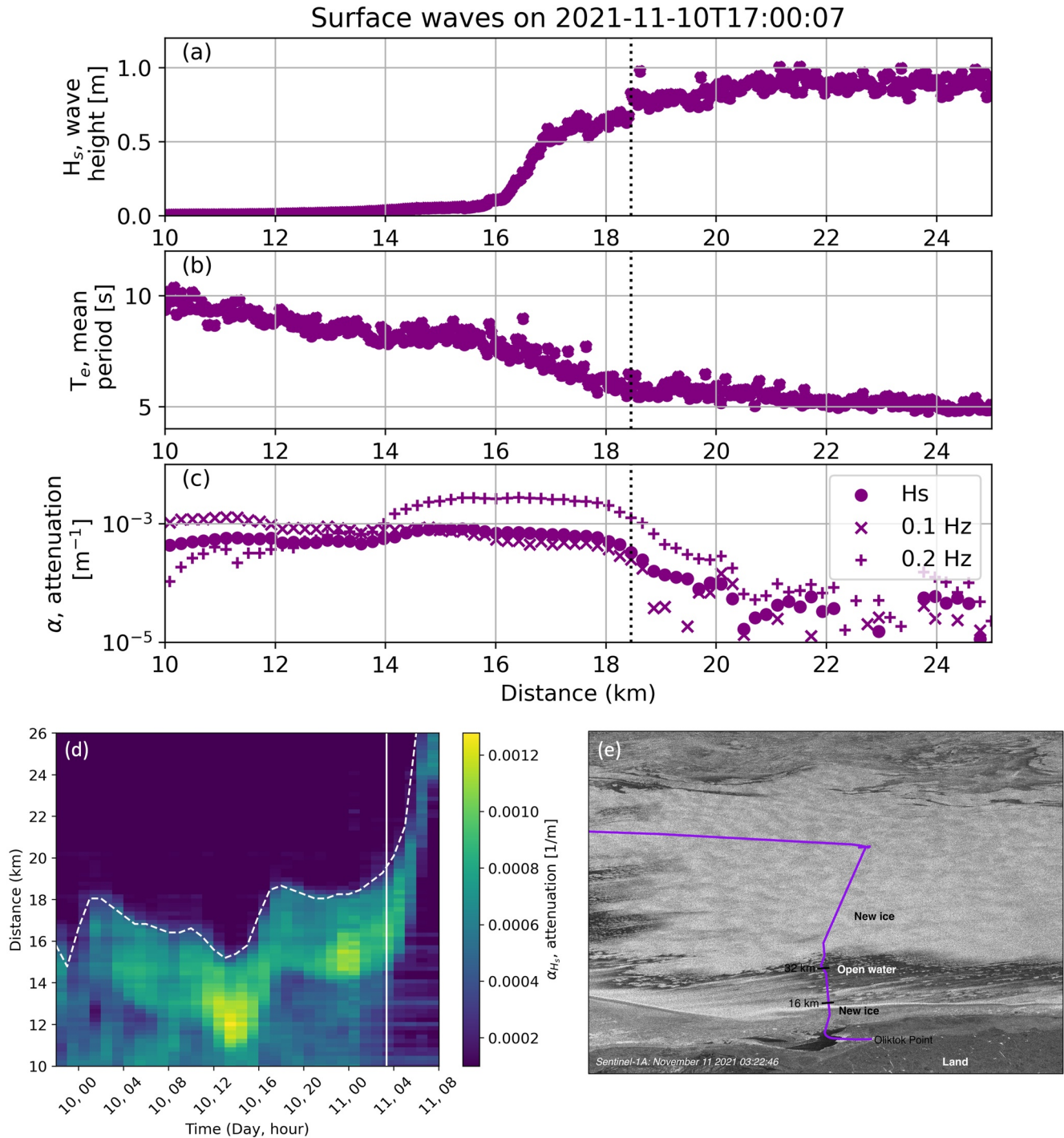
Figure 4. Wave parameters during November 2021 ice advance, where panels (a–c) shows along-cable estimates from a cross-section with partial ice cover on 10 November 2021, 17:00 for: (a) significant wave height, (b) energy-weighted mean wave period, and (c) wave attenuation rates. Wave attenuation is shown for significant wave height (circles), and at 0.1 Hz (x's) and 0.2 Hz (+s), which bracket the range of mean wave periods observed (5–10 s; (c)). The dotted vertical line suggests the inferred location of the ice edge based on a bulk wave height attenuation rate of 3 \times 10^{-4} \text{ m}^{-1} . (d) Map of bulk wave height attenuation from November 9, 22:00 – November 11, 08:00, from 10 to 26 km along-cable distance. Dark blue suggests near-zero attenuation likely associated with open water. Green-yellow corresponding to higher attenuation rates suggest the presence of sea ice, where the dashed white line denotes the approximate ice edge associated with attenuation of greater than 3 \times 10^{-4} \text{ m}^{-1} . Vertical white line corresponds to time of synthetic aperture radar backscatter in (e) from November 11, 03:22, which suggests new ice (lower backscatter; white) to approximately 18 km along-cable distance. Black ticks correspond to 16 and 32 km along-cable distance. The full cable path is shown in purple, but observations only extend to 37.4 km along-cable distance (Section 2.1). Copernicus Sentinel data 2021 retrieved from ASF DAAC 18 May 2023, processed by ESA.
