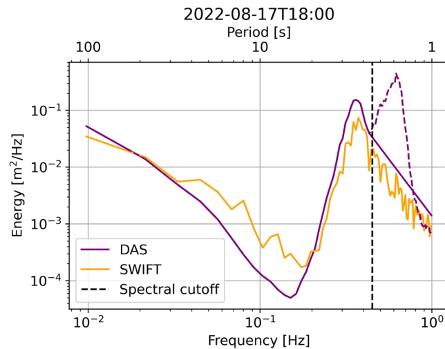
Figure A4. Example of methods for correcting high-frequency noise in wave spectra (see Section 2.4). An inflection point is determined empirically from original DAS-derived spectra (dashed purple line), here around 0.45 Hz. Beyond that, corrected spectra (solid purple line) is fit with the canonical f^{-4} slope for high-frequency waves. Observed wave spectra from Surface Wave Instrument Float with Tracking (orange) shows improved agreement with the corrected spectra. Note that the secondary peak at 0.7 Hz may be evidence of acoustic harmonics from ocean surface gravity waves (e.g., Ardhuin et al., 2013), which will be explored with this data set in future work.
