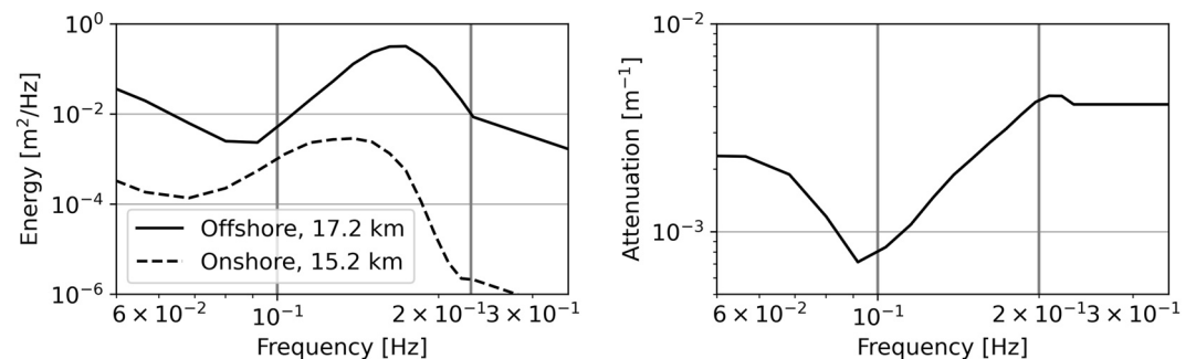
Figure A5. Example calculation of spectral attenuation following Equation 1. DAS-derived wave spectra from 17.2 to 15.2 km along-cable distance (left) are used to calculate attenuation rate (right). Vertical lines correspond to the frequency values shown in Figure 4c (x's and +s).
