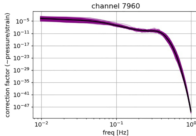
Figure A2. All empirical correction factors for channel 7,960 (16.2 km along-cable distance, as in example in Figure A1). Black line indicates the median value that is used as the channel-specific empirical correction factor in subsequent analysis.
