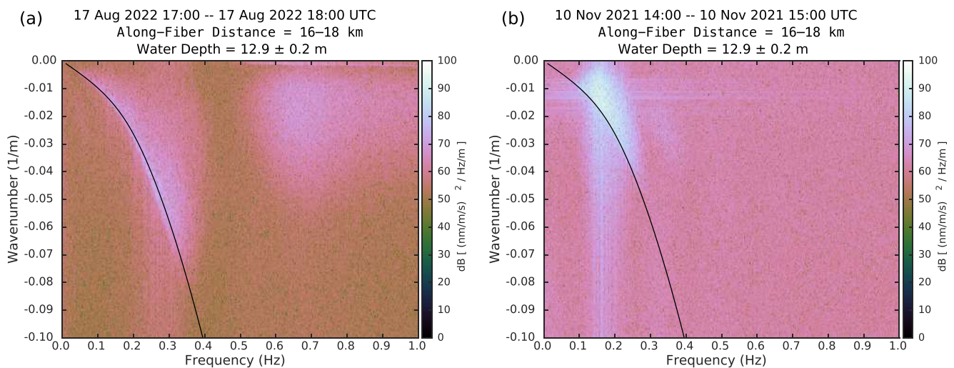
Figure 2. Frequency-wavenumber (f–k) plots using 1 hr of data at 1001 distributed acoustic sensing channels from 16 to 18 km along-fiber distance. Gravity wave dispersion curves (black lines) were calculated using the mean water column depth. Ocean gravity waves are observable both in panel (a) open water, 17 August 2022, 17:00–18:00 and (b) seasonal ice-cover, 10 November 2021, 14:00–15:00.
