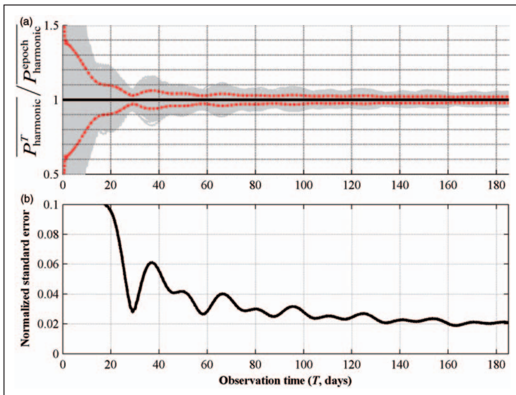
Figure 5. (a) Convergence of average power generation (calculated from harmonic currents) to its epoch value (thin lines denote individual realizations over the epoch and dashed lines denote standard error) and (b) standard error normalized by running mean of power generation as a function of observation time.
