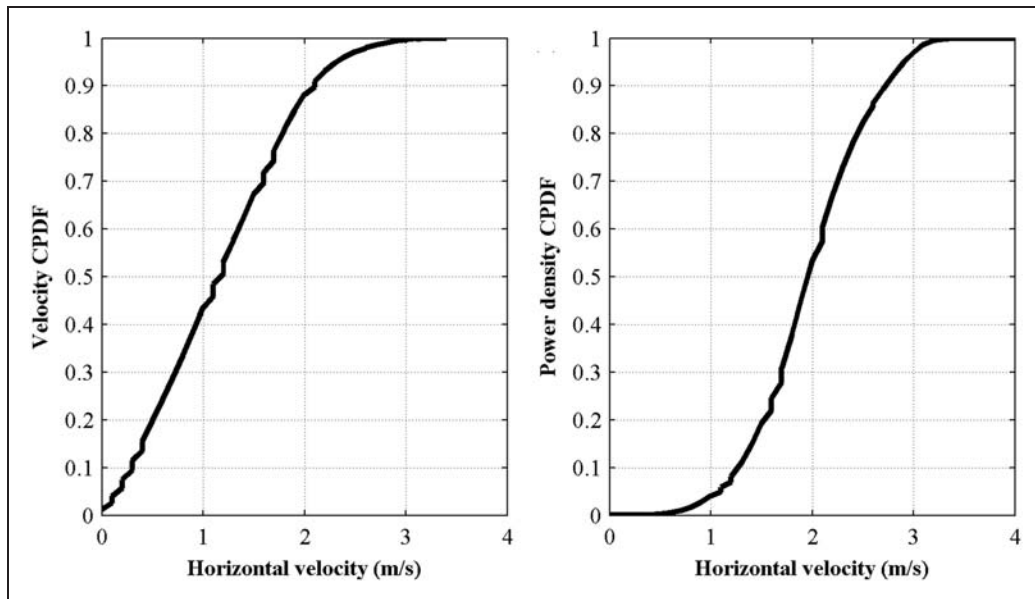
Figure 11. Cumulative probability density functions (CPDFs) of velocity and power density (site 1, mid-water depth).
