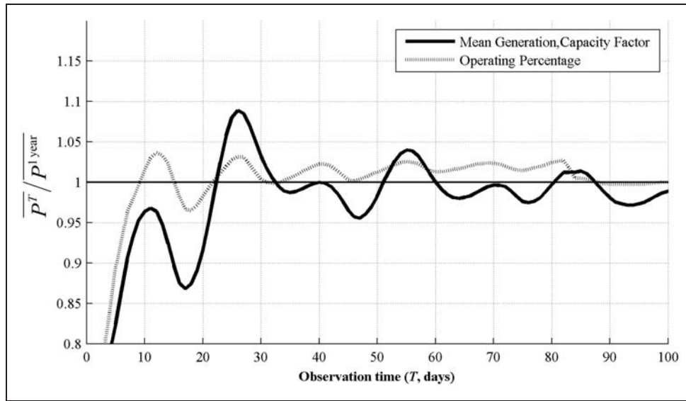
Figure 9. Convergence of turbine performance metrics to long-term values (site 1, passive yaw).
