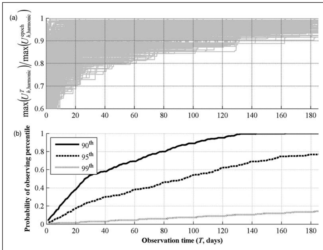
Figure 4. (a) Convergence of the maximum harmonic current to its epoch value (thin lines denote individual realizations over the epoch) and (b) probability of observing the N th percentile harmonic currents over a given observation time.
