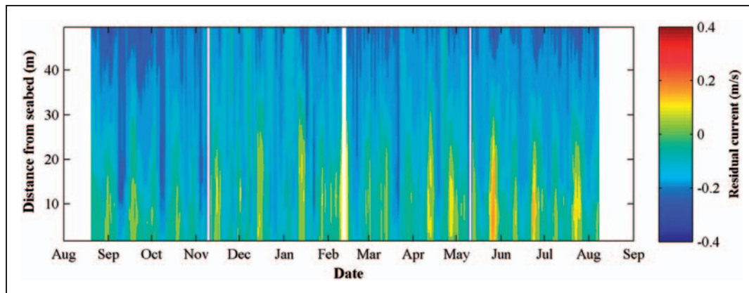
Figure 6. Residual currents for site 1. Gaps in the record correspond to recovery and redeployment of the instrumentation package.
