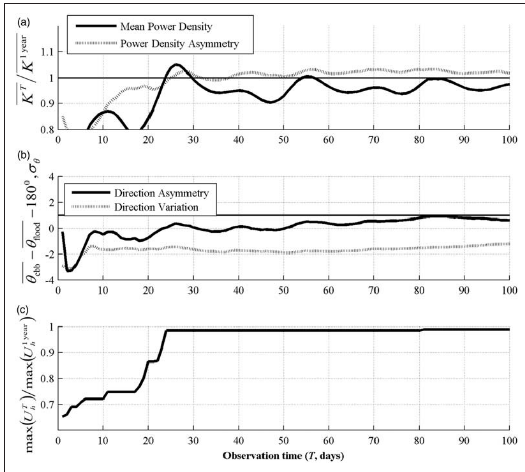
Figure 7. Convergence of resource metrics to annual average values (site 1): (a) power density, (b) mean direction, and (c) maximum velocity.
