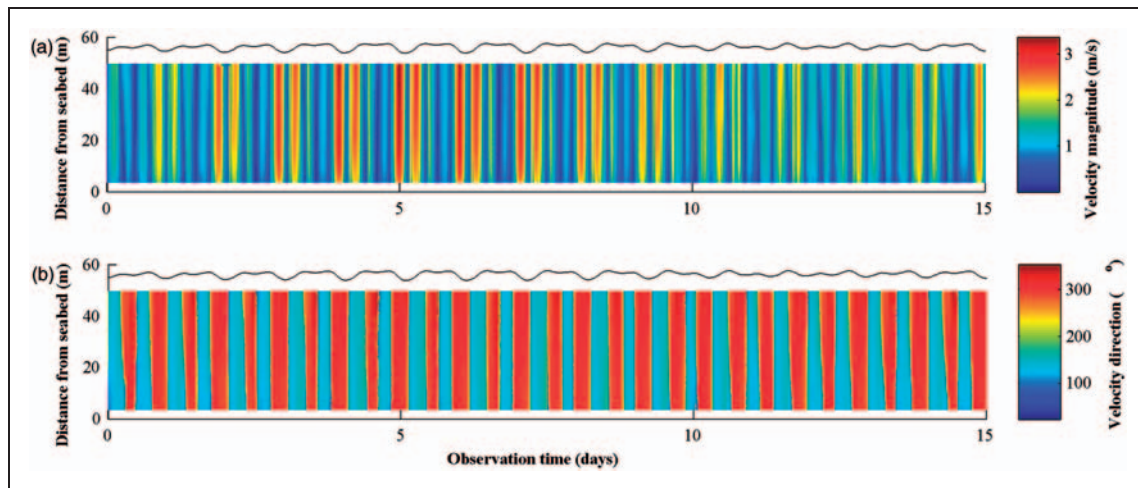
Figure 2. Representative acoustic Doppler current profiler (ADCP) data (days 0–15 from site 5): (a) horizontal velocity magnitude and (b) horizontal velocity direction.
