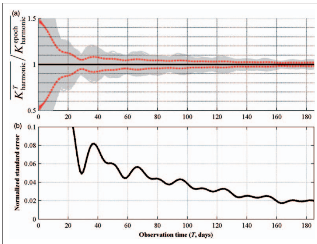
Figure 3. (a) Convergence of mean power density (calculated from harmonic currents) to its epoch value (thin lines denote individual realizations over the epoch and dashed lines denote standard error) and (b) standard error normalized by running mean power density as a function of observation time.
