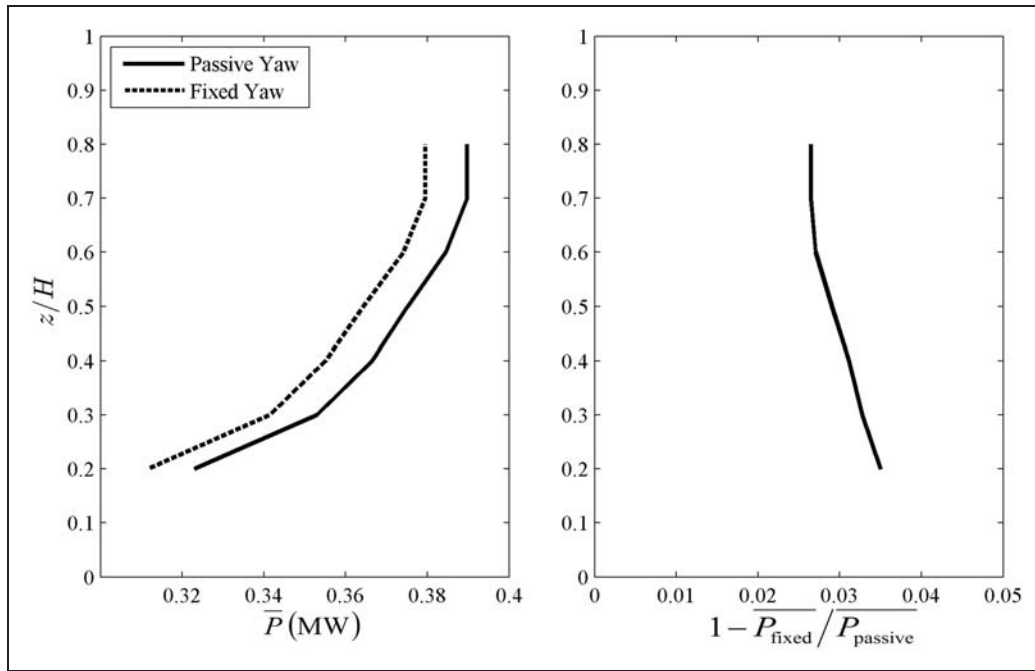
Figure 10. Vertical profiles of average power generation for a turbine (site 7), contrasting performance between passive and fixed yaw devices over a range of depths.
