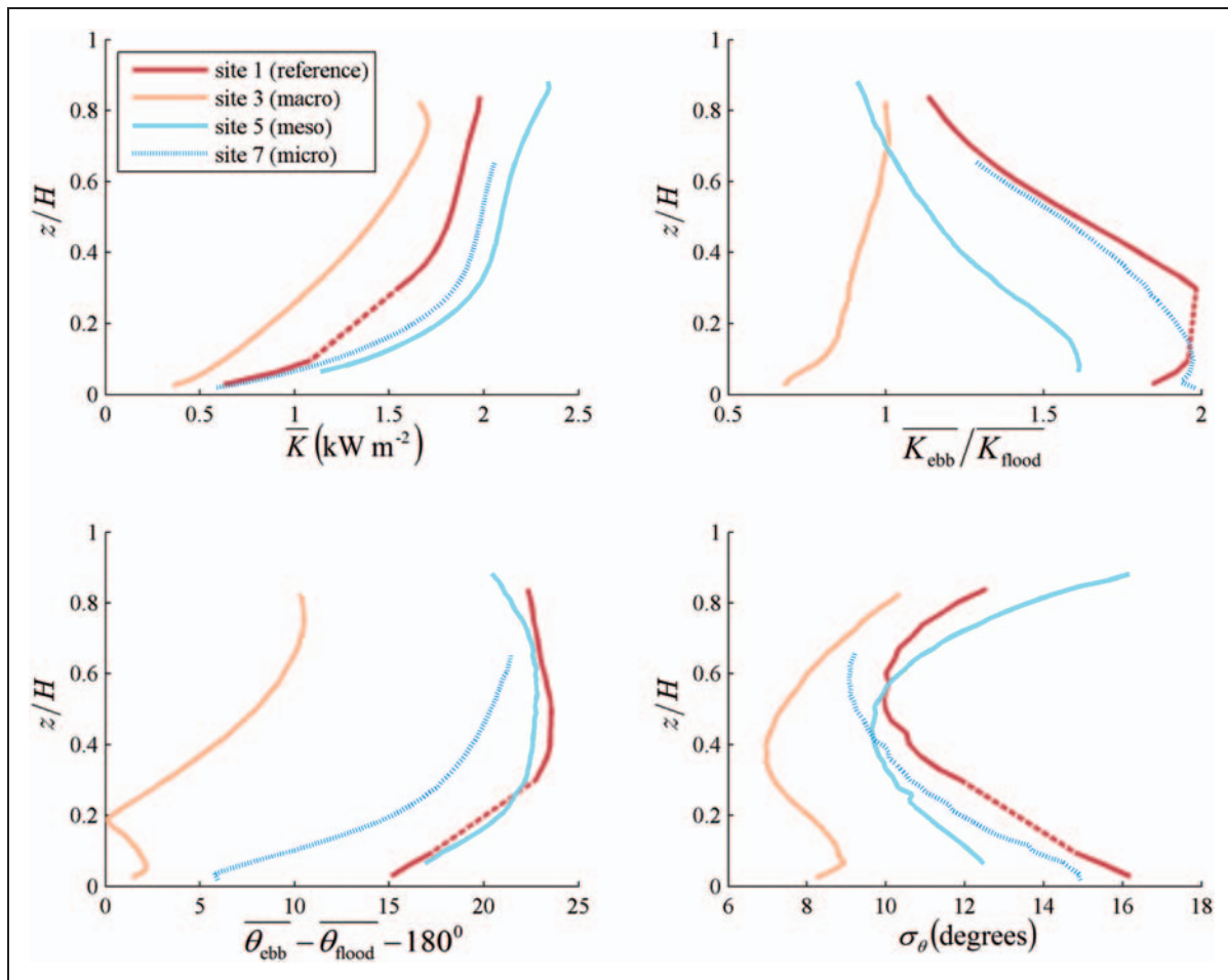
Figure 8. Vertical variations in resource characteristics at sites in northern Admiralty Inlet, Puget Sound, WA. Acoustic interference over dashed portion of reference site profiles.
