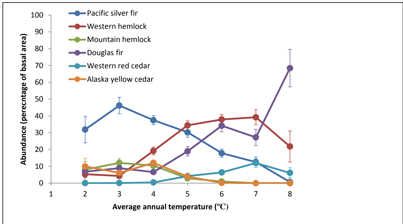
Figure 3. The relationship between tree species abundance and average annual temperature. Tree abundance is measured in terms of the percentage of total tree basal area for the given species (basal area is the area of a cross section of a tree’s trunk measured at 137cm, or 4.5ft, above the ground). Error bars show standard error. The temperature data was produced by the PRISM climate model (Daly et al. 2008), while the data on tree abundance came from surveys of forest plots around the Park (Franklin et al. 1988).
