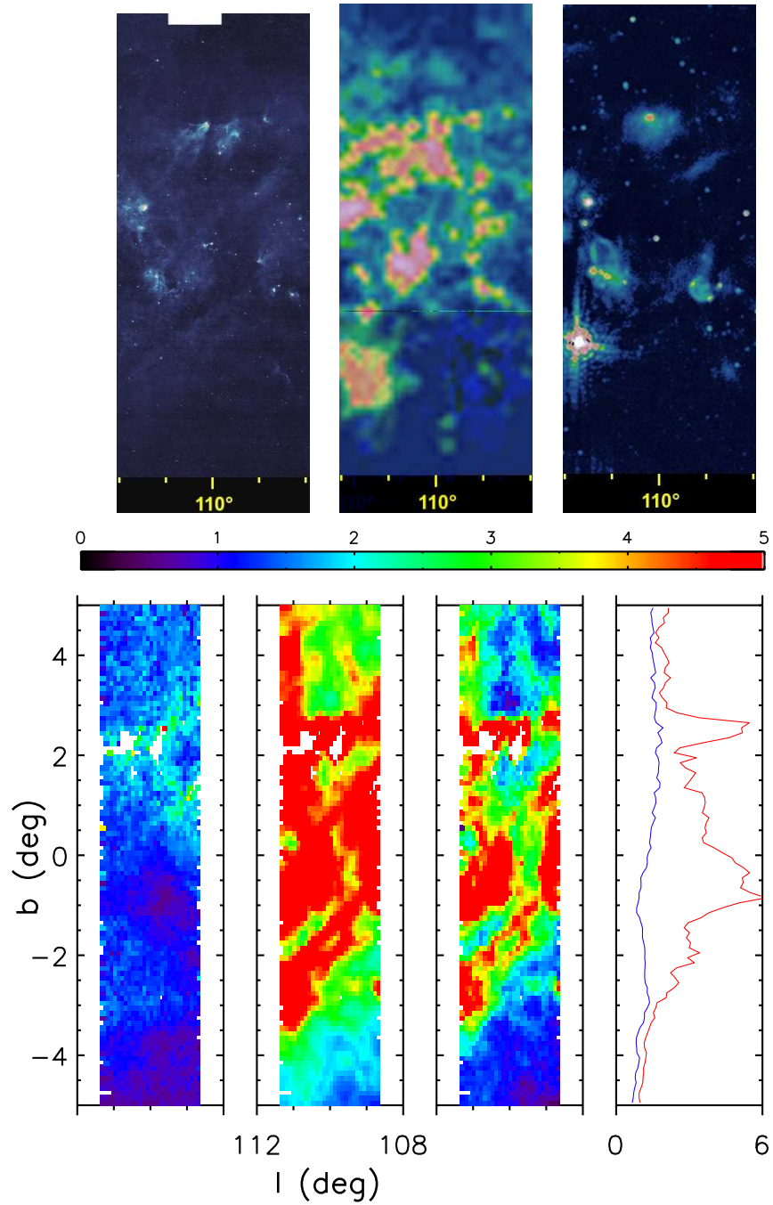
Fig. 28.— The bottom three panels show the |b| < 5^\circ subregion of the panels shown in Fig. 27. The top three panels show the mid-IR (left), CO (middle) and radio continuum (right) maps on approximately the same scale (obtained using “The Milky Way Explorer” by Kevin Jardine). Assuming that the SFD map is not grossly incorrect, the dust extinction determined here implies that most of the molecular cloud structures seen in the top middle panel must be more distant than \sim 1 kpc.
