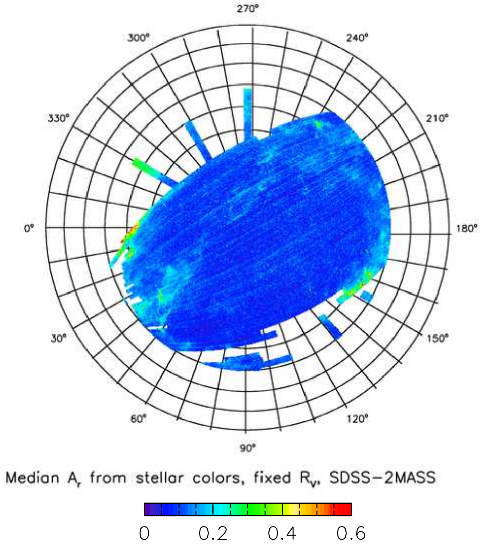
Fig. 17.— The color-coded maps shows the median best-fit A_r based on SDSS and 2MASS data for 12 million stars with 15 < r < 20 from the northern galactic cap ( |b| > 30^\circ ). The values are linearly color-coded according to the legend. The fitting was done with a fixed extinction curve, and only the stellar SEDs and the amount of dust ( A_r ) are varied when fitting the observed colors.
