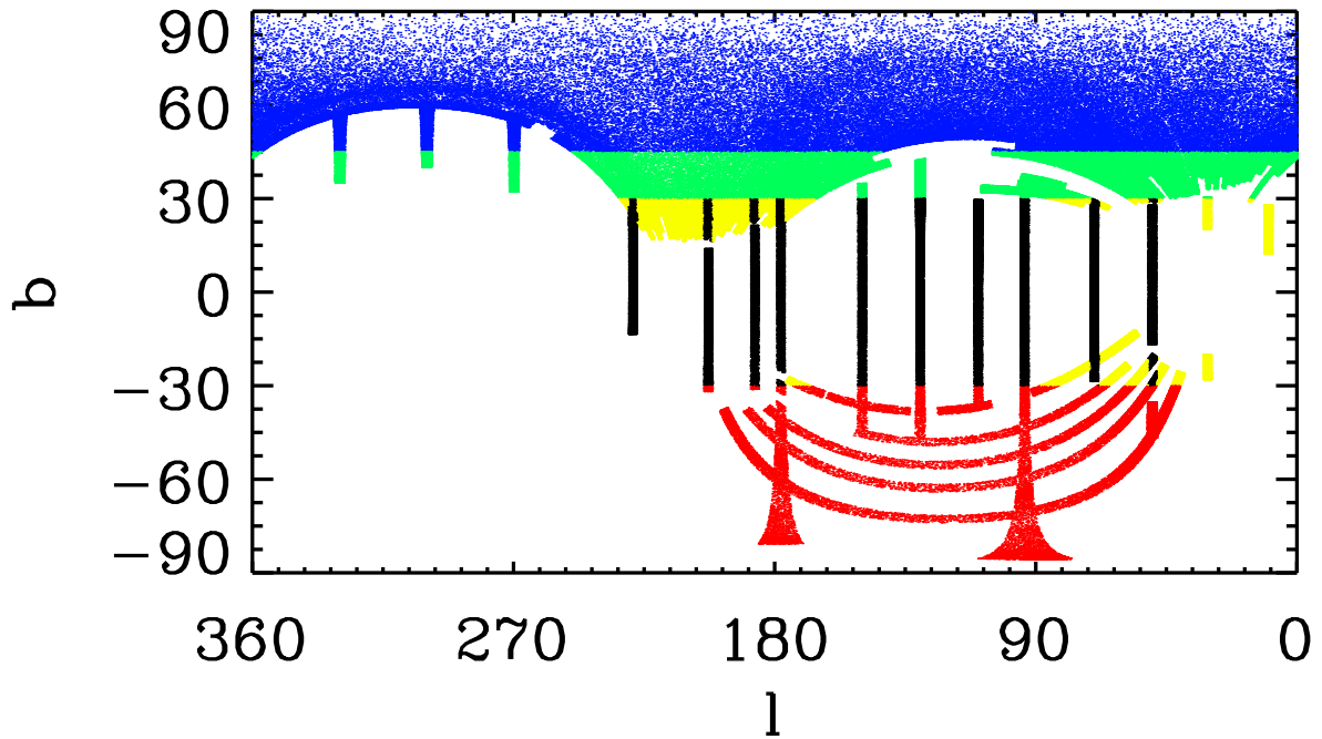
Fig. 1.— The sky coverage for SDSS Data Release 7, used in this study. The points show a small random subsample of the full sample of 73 million stars. The different colors represent the various data file sets (blue, b > 45 ; green, 45 > b > 30 ; black, the 10 SEGUE strips; yellow |b| < 30 , stars not in SEGUE strips; and red, b < -30 ). In this paper, only the results from the 10 SEGUE strips are reported.
