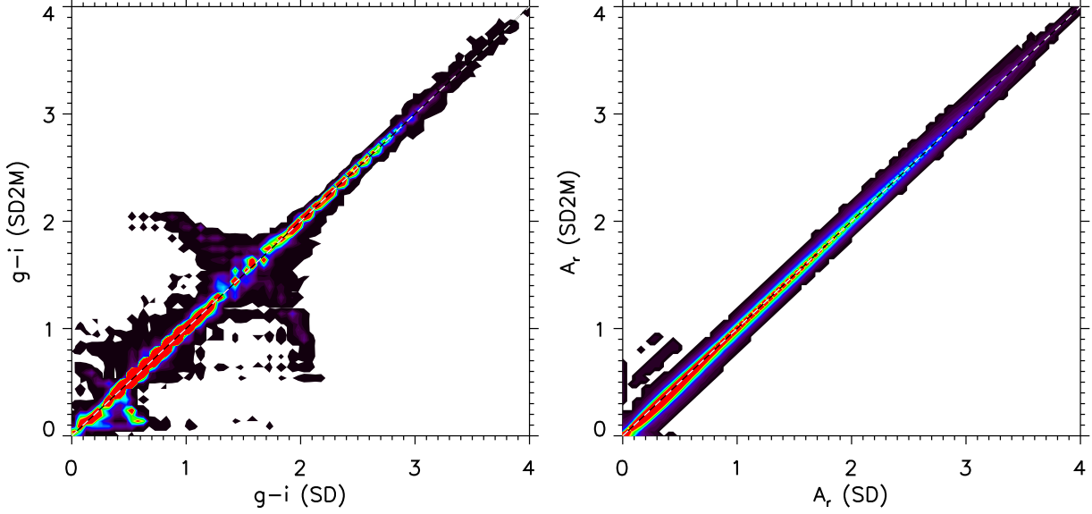
Fig. 23.— A comparison of the best-fit g-i (left panel) and A_r (right panel) values obtained with a fixed R_V = 3.1 for SDSS-2MASS sample from the SEGUE l \sim 110^\circ stripe, using two different fitting methods. The x axes show the best-fit values obtained using only-SDSS dataset (four fitted colors), and the y axes correspond to SDSS-2MASS dataset (seven fitted colors). The number density of stars increases linearly from black to blue to red. The dashed lines have a slope of unity and are added to guide the eye.
