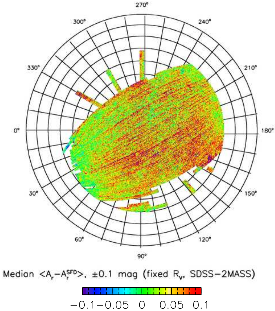
Fig. 18.— The color-coded maps shows the median difference between the best-fit A_r shown in Figure 18 and the values given by the SFD map at the position of each star. The values are linearly color-coded according to the legend. Note the striping that is reminiscent of the SDSS scanning pattern. These coherent residuals imply problems with the transfer of SDSS photometric zeropoints across the sky.
