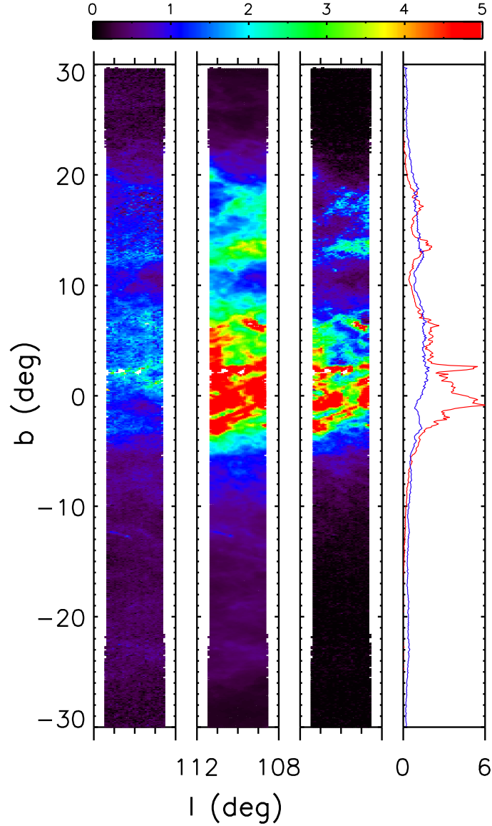
Fig. 27.— Analysis of the differences between best-fit A_r values (left panel, based on only-SDSS data; SDSS-2MASS version looks similar) and the SFD values (middle panel) for stars with \chi_{pdf}^2 < 2 , and main-sequence distance in the range 0.8 – 1.2 kpc. Each 6 \times 6 arcmin 2 pixel in the first three panels is color coded according to the legend on top. The fourth panel shows the median best-fit A_r (blue line) and the median SFD value (red line) for 0.2 deg. wide bins of Galactic latitude. If the SFD maps are correct, then the dust structures discernible in the two right panels at b \sim 0^\circ and b \sim 2^\circ must be more distant than \sim 1 kpc. This conclusion is independently confirmed for the latter dust cloud in Figure 26.
