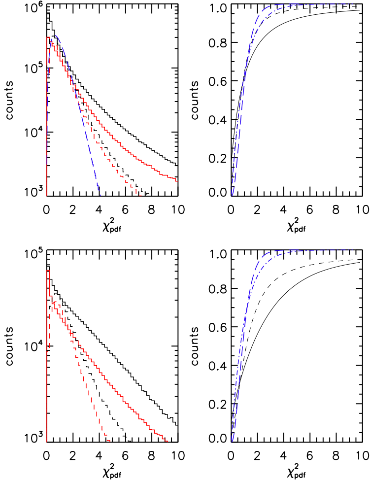
Fig. 16.— The distribution of the best-fit \chi_{\text{pdf}}^2 ( R_V = 3.1 ), with differential distributions in the left two panels, and cumulative distributions in the right two panels. The top two panels correspond to the north galactic cap region ( b > 45^\circ ) and the bottom two panels to the SEGUE l \sim 110^\circ strip, limited to |b| < 5^\circ (a high-extinction region). The solid lines are used for SDSS-only fits, and the dashed lines for fits to SDSS-2MASS data. In the two left panels, the top solid line corresponds to subsamples of stars with r < 20 , and the bottom solid line to stars with 20 < r < 21 . The top dashed line corresponds to the full SDSS-2MASS sample, and the bottom dashed line to subsamples with K < 13.9 (Vega scale, approximately corresponding to K band errors up to 0.05 mag). The solid lines in the right panels correspond to full SDSS sample, and the short-dashed lines to full SDSS-2MASS sample. The dot-dashed and long-dashed lines correspond to \chi_{\text{pdf}}^2 distributions with 2 and 5 degrees of freedom.
