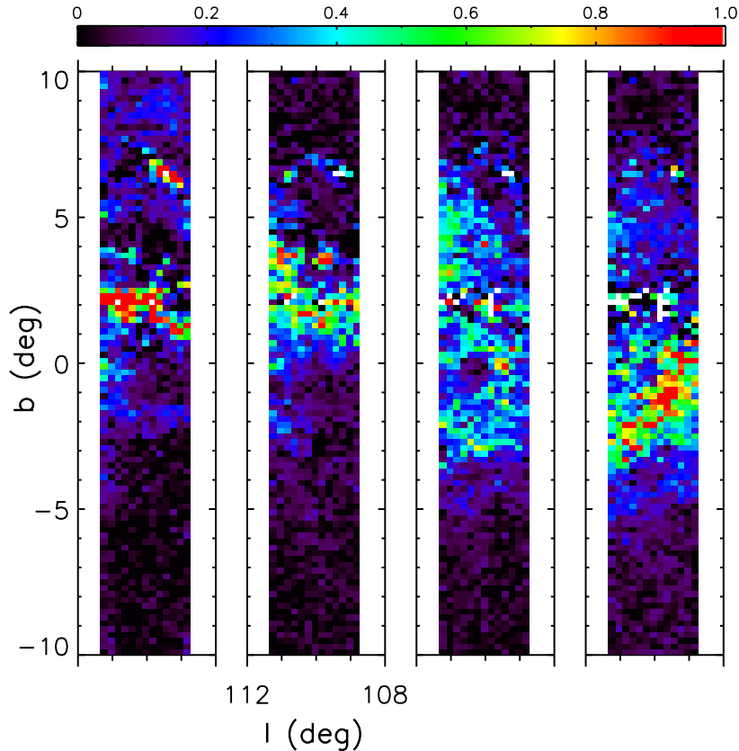
Fig. 34.— Illustration of the three-dimensional dust distribution for SEGUE stripe l \sim 110^\circ at mean distances of 1.0, 1.5, 2.0 and 2.5 kpc. Unlike other figures that show the median A_r along the line of sight, this figure shows the differences in the median A_r (per 12 \times 12 arcmin 2 pixel) for limiting distances 0.25 kpc larger and smaller than the mean distance. It is easily discernible that the dust structure observed at b \sim 2^\circ is confined to 1-1.5 kpc distance range, while the structure seen at -3^\circ < b < 0^\circ is due to dust at a distance of \sim 2.5 kpc (an analogous panel for a mean distance of 3.0 kpc shows that this structure is mostly confined to smaller distances). Note that the linear extent perpendicular to the line of sight of a given angular size is 2.5 times larger in the last than in the first panel.
