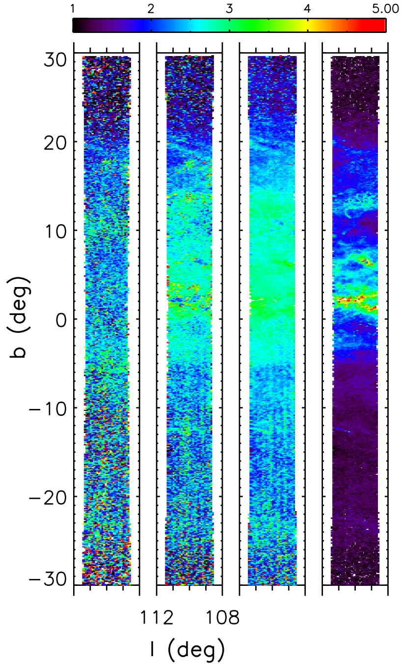
Fig. 33.— The first three panels show the median R_V obtained using SDSS-2MASS sample for the SEGUE l = 110 strip, and for distance range 0.1–0.5 kpc (left), 0.5–1 kpc (middle), and 0.8–1.2 kpc (right). Only stars outside the “red giant” region, see Figure 21, and with \chi_{pdf}^2 < 2 , r < 21 and K < 14.3 (Vega) are used for the plot. The pixel size is 6 \times 6 arcmin 2 . The fourth panel shows for reference the best-fit A_r , for the distance slice 0.8–1.2 kpc.
