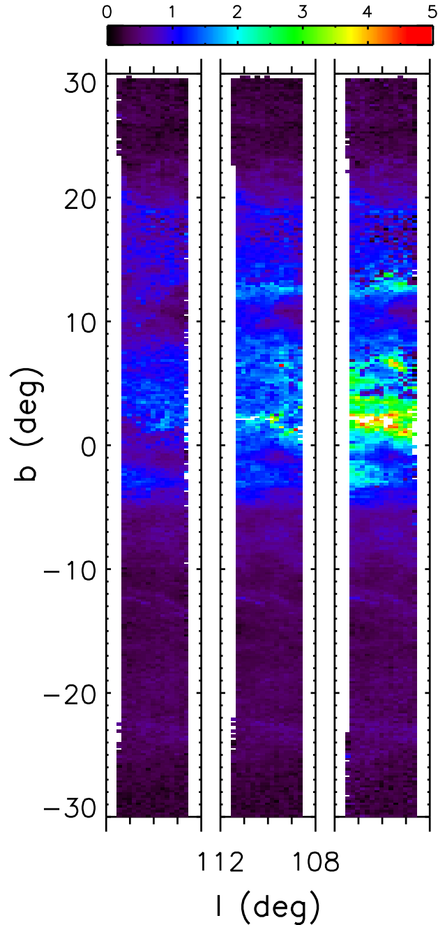
Fig. 25.— The color-coded maps shows the best-fit A_r based on only-SDSS dataset for the SEGUE l \sim 110^\circ strip. The legend shows the color scale, and each 12 \times 12 arcmin 2 pixel shows the median A_r . The three panels correspond to main-sequence distance range: 0.3 – 0.6 kpc (left), 1 – 1.5 kpc (middle) and 2 – 2.5 kpc (right). Only stars with best-fit \chi_{pdf}^2 < 2 and outside the red giant region (selected here by A_r < 1.5 + 1.5 D_{\text{kpc}} ) are used for the plot.
