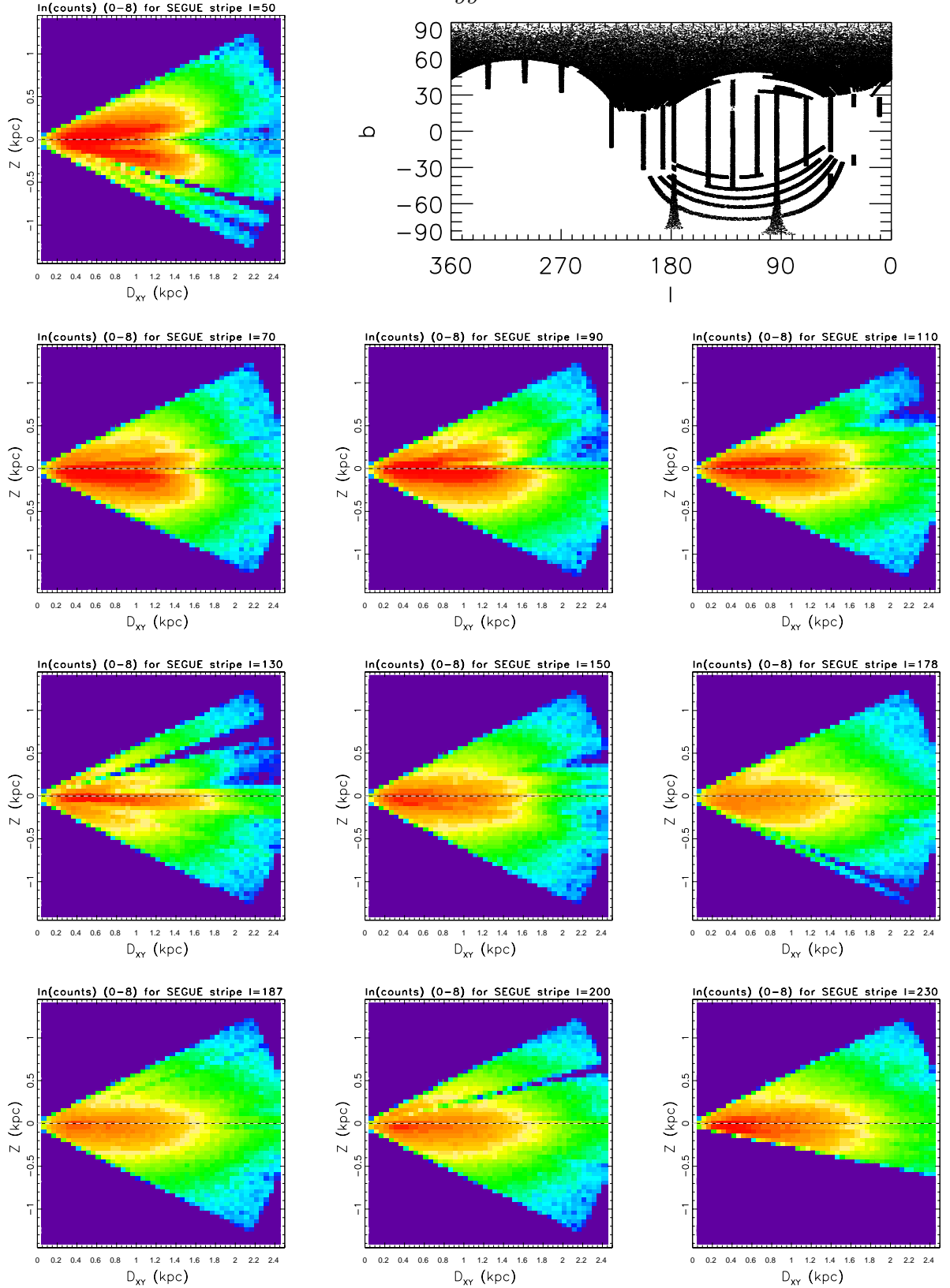
Fig. 36.— The local volume number density of stars is shown as a function of distance from the Galactic plane, Z , and distance along the plane, D_{xy} , for 10 SEGUE stripes. Each pixel is 50 \times 50 \text{ pc}^2 (and subtending whole 2.5 \text{ deg} wide stripe), and the color scheme shows the counts on a log scale (same arbitrary normalization for all stripes). The fall-off of the stellar
