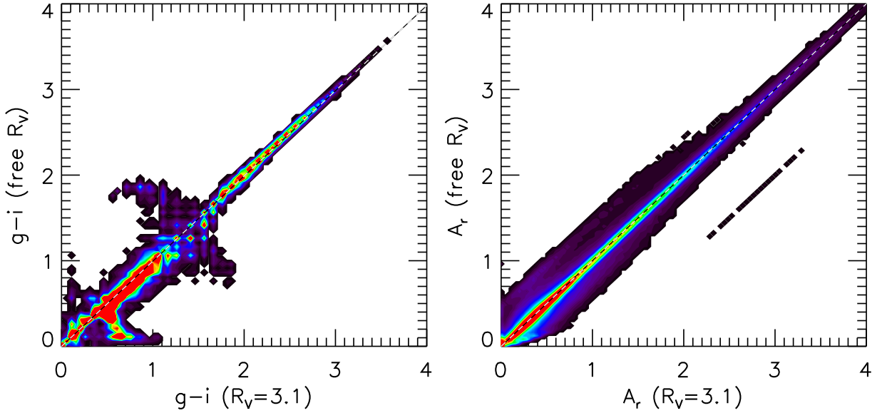
Fig. 29.— A comparison of the best-fit g - i (left panel) and A_r (right panel) values for two different treatments of R_V , for stars in the l = 110 SEGUE strip (using SDSS-2MASS data). Only stars with best-fit \chi_{pdf}^2 < 2 , r < 20 and K < 13.9 (Vega) are used for the plot. The x axes show the best-fit values obtained for a fixed R_V = 3.1 and the y axes correspond to values obtained with R_V as a free fitting parameter. The number density of stars increases from black to blue to red. The dashed lines have a slope of unity and are added to guide the eye.
