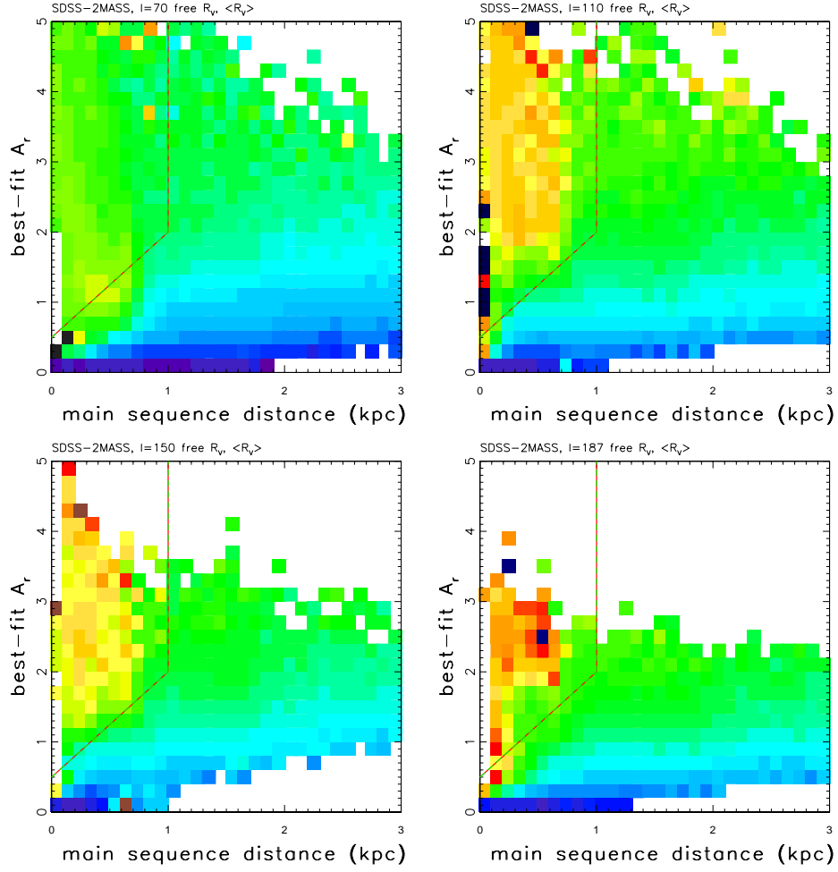
Fig. 31.— Similar to Figure 21, except that R_V is treated as a free parameter, and the color-coded map shows the median value of R_V (ranging from blue for R_V = 2 to red for R_V = 4 , green corresponds to R_V = 3 ). Note that red giant stars (top left corner) have consistently larger values of R_V , and that consistently R_V < 3 when A_r < 1 for main sequence stars.
