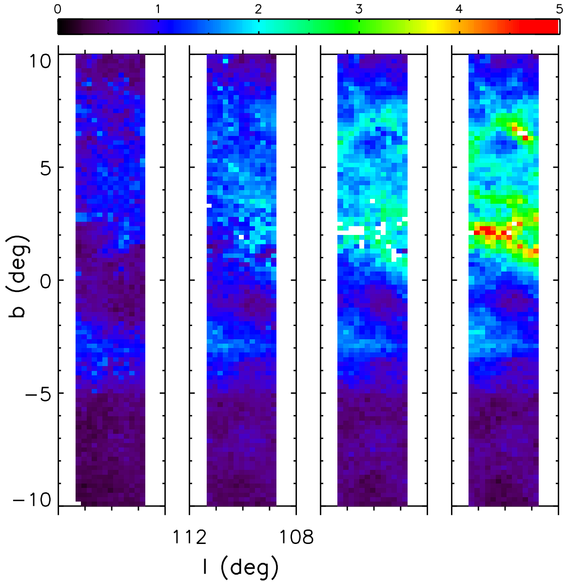
Fig. 26.— Analogous to Figure 25, except for using SDSS-2MASS dataset and different distance slices (left to right: 0.1 – 0.5 kpc, 0.5 – 0.7 kpc, 0.7 – 0.9 kpc, 0.9 – 1.1 kpc). Note the abrupt increase in A_r for stars more distant than 0.9 kpc.
