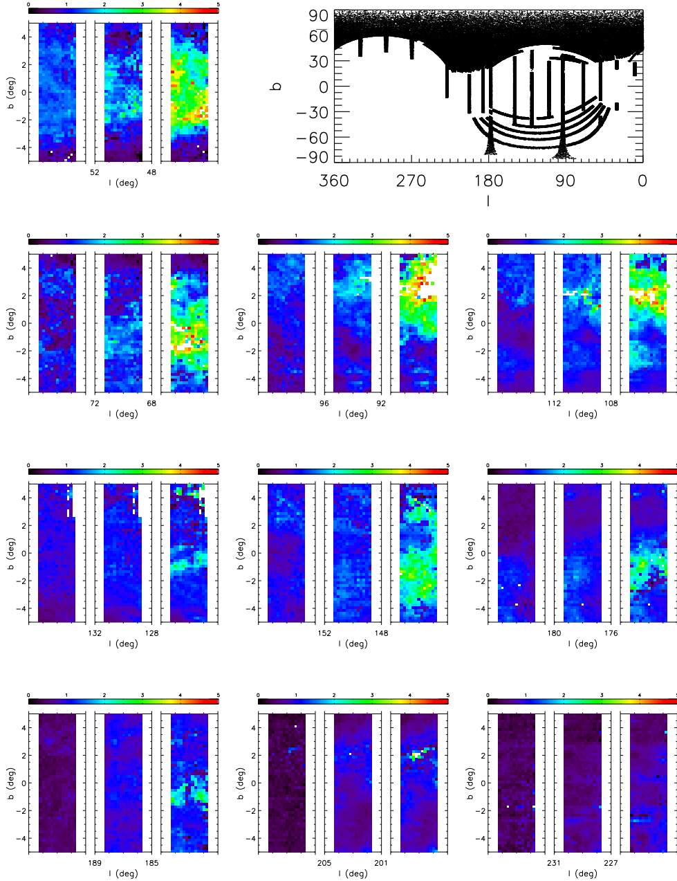
Fig. 19.— The color-coded maps show the best-fit A_r based on SDSS data for the ten analyzed SEGUE stripes. Each stripe is limited to the range of galactic latitude, |b| < 5^\circ . A fixed R_V = 3.1 is assumed. The legend above each panel shows the color scale, and each 12 \times 12 arcmin 2 pixel shows the median A_r . For each stripe, three distance ranges are shown: 0.3-0.6 kpc (left), 1-1.5 kpc (middle) and 2-2.5 kpc (right). It is assumed that all stars are on main sequence when estimating distances. Only stars with best-fit \chi_{pdf}^2 < 2 and outside the red giant region (selected here by A_r < 1.5 + 1.5 D_{\text{kpc}} ) are used for the plot. The top right panel shows the sky coverage of the full analyzed dataset.
