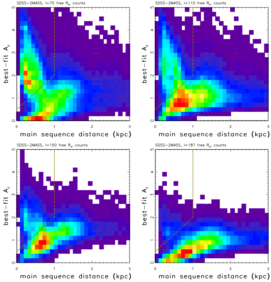
Fig. 30.— The A_r map analogous to Figure 21, except that R_V is treated as a free parameter.
