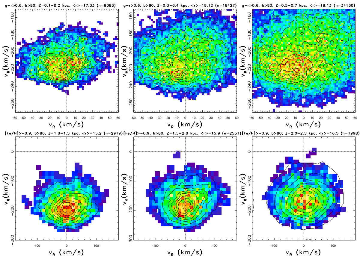
Fig. 3.— Similar to Figure 2, except that the v_\Phi vs. v_R velocity distribution is plotted for a range of Z . The top row shows the v_\Phi vs. v_R diagrams for \sim 60,000 red ( g - r > 0.6 ) stars at Z = 100 - 700 pc and observed towards the North Galactic Pole. Each panel corresponds to a narrow range in Z , given above each panel. The measurement errors vary from \sim 3 km s ^{-1} in the closest bin to \sim 12 km s ^{-1} in the most distant bin. Note the complex multi-modal substructure in the top left panel. The bottom three panels are analogous, and show the v_\Phi vs. v_R diagrams for \sim 7,000 blue ( 0.2 < g - r < 0.4 ) stars with high metallicity ( [Fe/H] > -0.9 ). The measurement errors vary from \sim 20 km s ^{-1} in the closest bin to \sim 35 km s ^{-1} in the most distant bin. Note that the median v_\Phi approaches zero as Z increases.
