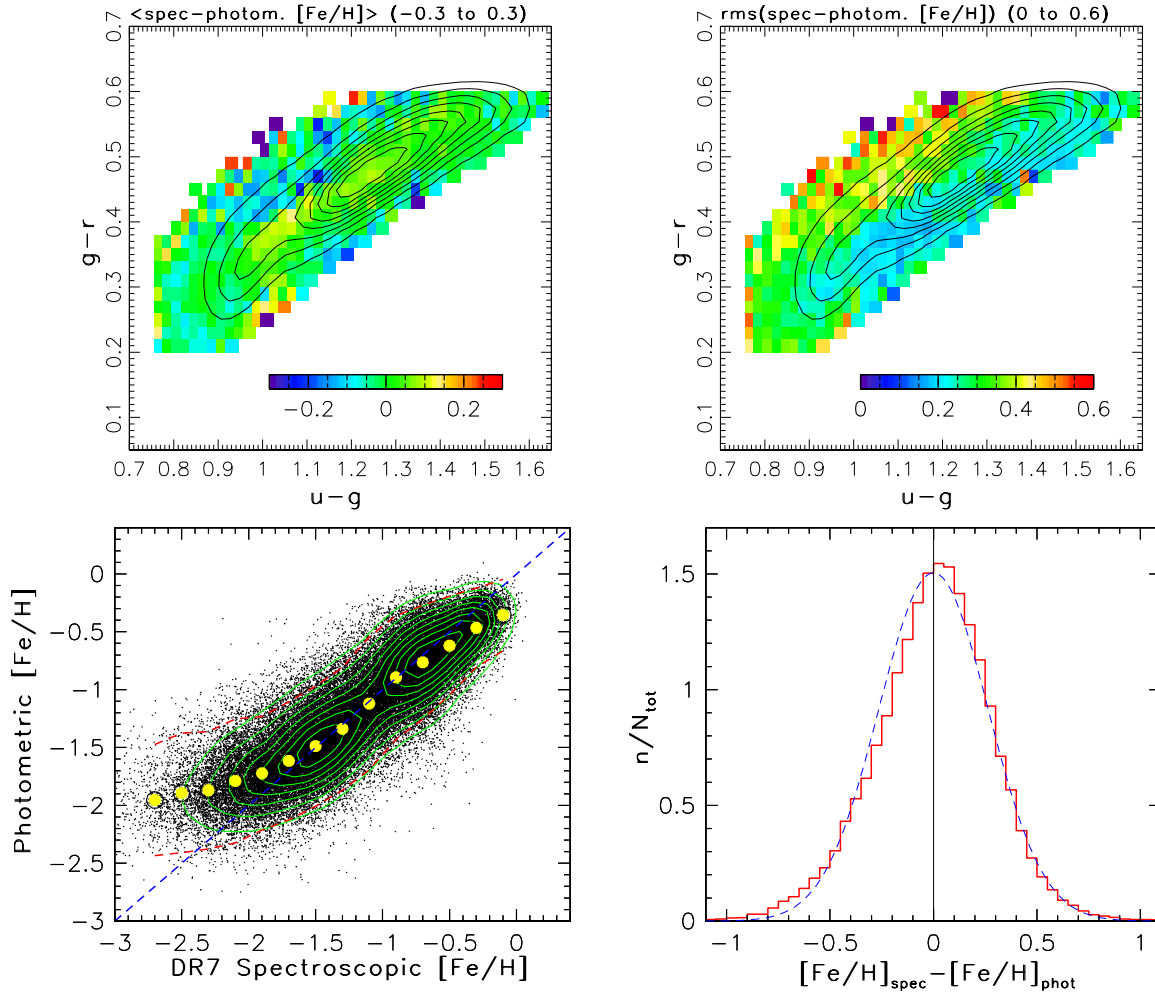
Fig. A2.— The color-coded map in the top left panel shows the median difference between spectroscopic and revised photometric metallicities for \sim 50,000 stars from SDSS Data Release 7. The median value is zero, and the root-mean-square scatter is 0.07 dex. The contours show the distribution of stars with r < 20 and at high Galactic latitudes. The top right panel shows the root-mean-square scatter of the difference between spectroscopic and photometric metallicities in each pixel. The top two panels are analogous to the bottom two panels in Figure 2 from I08. The bottom left panel shows the photometric metallicity as a function of the spectroscopic metallicity. Individual stars are shown by small dots, and the median values of the difference are shown by large circles. The distribution of stars is shown as linearly-spaced contours. Note that the photometric metallicity saturates at [Fe/H] \sim -2 at the low-metallicity end. The histogram in the bottom right panel shows the distribution of the difference between spectroscopic and photometric metallicities for stars with spectroscopic metallicity [Fe/H] > -2.2 . A best-fit Gaussian centered on zero and with a width of 0.26 dex is shown by the dashed line.
