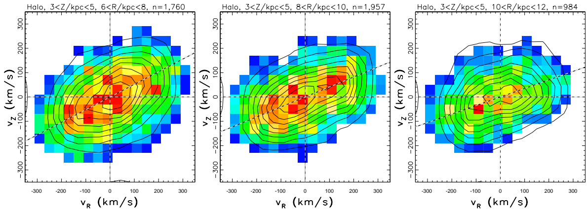
Fig. 13.— An illustration of the velocity-ellipsoid tilt- angle variation. Analogous to Fig. 12, except that only the v_Z vs. v_R projection is shown for a constant Z , for three ranges of R , as marked on the top of each panel.
