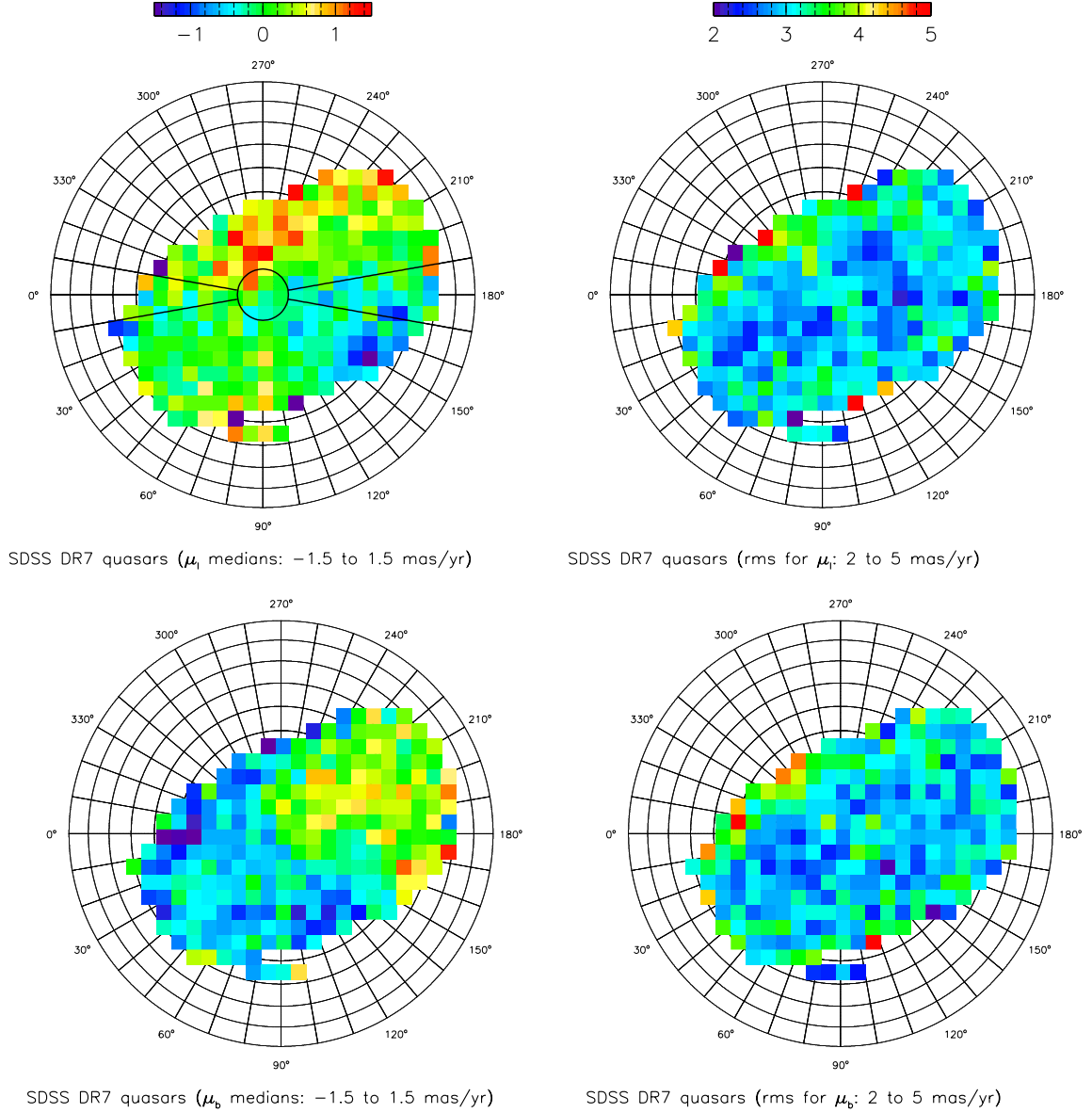
Fig. 1.— Behavior of proper-motion measurements for 60,006 spectroscopically confirmed SDSS quasars with b > 0^\circ . The color-coded maps (see the legend on top, units are \text{mas yr}^{-1} ) show the distribution of the median (left) and rms (right) for the longitudinal (top) and latitudinal (bottom) proper motion components in a Lambert projection of the northern Galactic cap. The median number of quasars per pixel is \sim 250 . For both components, the scatter across the sky is 0.60 \text{ mas yr}^{-1} . The median proper motion for the full quasar sample is 0.15 \text{ mas yr}^{-1} in the longitudinal direction, and -0.20 \text{ mas yr}^{-1} in the latitudinal direction. The thick line in the top left panel shows the selection boundary for the “meridional plane” sample.
