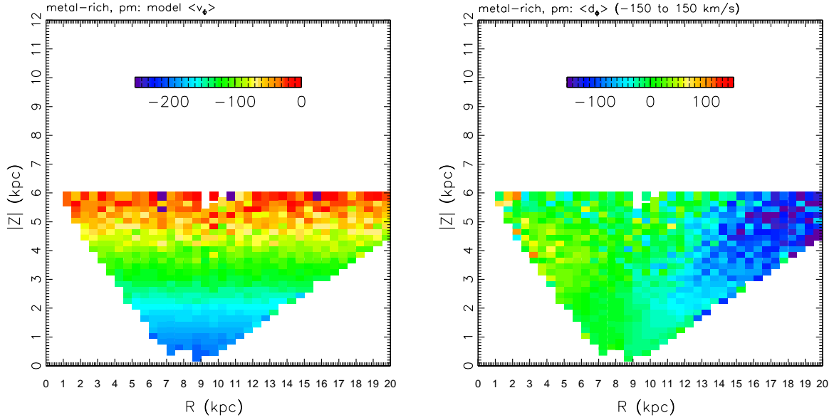
Fig. 9.— Left panel is analogous to the bottom left panel in Figure 8, but for the model described in the text. The right panel shows the median difference between the data and model. Large discrepancies at R > 12 kpc are due to the Monoceros stream (at R = 18 kpc and Z = 4 kpc; disk stars rotate with a median v_\phi \sim -100 km s ^{-1} , while for the Monoceros stream, v_\phi \sim -200 km s ^{-1} ).
