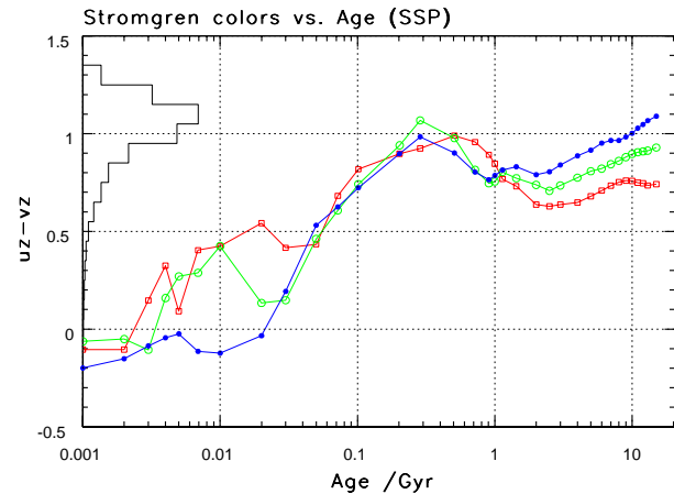
Figure 27. The Bruzual & Charlot model predictions for the dependence of the uz - vz color on age and metallicity ( [Z] = 0.004 , squares; 0.02, circles; 0.05, dots) of single stellar populations. Note that for small ages ( \lesssim 30 Myr) metallicity can have a strong impact on the uz - vz color, while for intermediate ages ( 30 \text{ Myr} \lesssim \text{age} \lesssim 2 \text{ Gyr} ) it plays only a minor role. For old stellar populations ( \gtrsim 2 \text{ Gyr} ), the uz - vz color becomes again increasingly sensitive to metallicity. However, not even for the oldest galaxies the model uz - vz color is sufficiently red to explain the observations.
