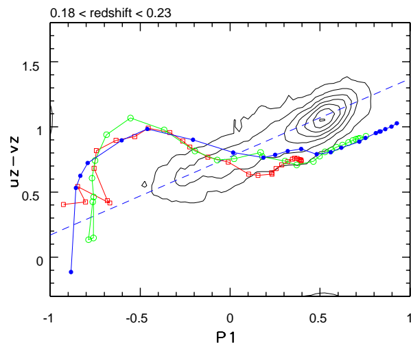
Figure 28. The uz - vz color vs. P1 color-color diagram. The observed galaxy distribution is shown by linearly spaced contours (the same distribution is shown by dots in Fig. 26). The Bruzual & Charlot model predictions are shown by lines and symbols, analogously to Fig. 27. The position along each model track is controlled by the age of single stellar population, while different track correspond to different metallicities. Note that the effects of age and metallicity are largely degenerate such that different model tracks do not deviate from each other by more than \sim 0.1 mag. Note also the discrepancy between the model tracks and the observed distribution.
