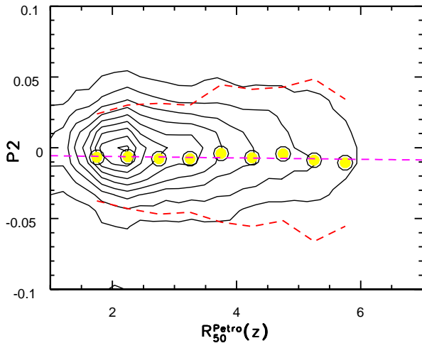
Figure 7. Analogous to Fig. 6, except for the P2 color and only for galaxies with P1 < 0 . The slope of the best fit line is -0.0005 mag/arcsec.
