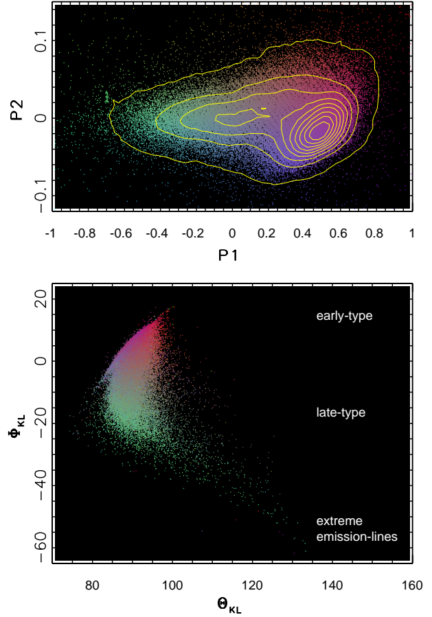
Figure 25. The bottom panel shows a spectral classification plane for galaxies proposed by Yip et al. (2004). Each galaxy is represented by a dot color-coded according to its position in the P1-P2 plane, shown in the top panel. The sequence from early-type to extreme emission line galaxies adopted from Yip et al. (2004) is shown on the right side in the bottom panel. Note the good correspondence between P1 and P2 colors and the Yip et al. classification.
