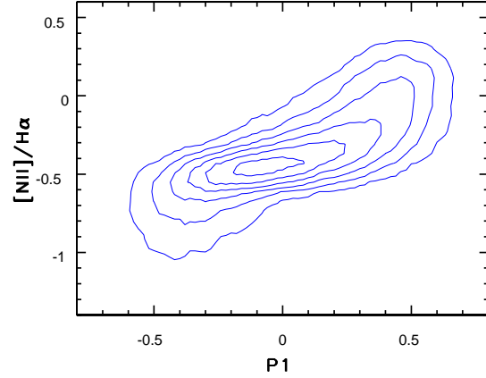
Figure 11. The correlation between the first principal axis in the rest-frame Strömgren color-color diagram, and the [NII]/H_{\alpha} line strength ratio. The distribution of all emission-line galaxies in the sample is shown by linearly spaced isopleths.
