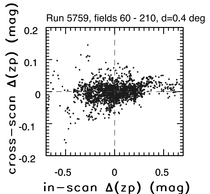
FIG. 14.— Comparison of cloud extinction gradients in the in-scan (right ascension, horizontal axis) and cross-scan (declination, vertical axis) directions for SDSS run 5759, on a spatial scale of \sim 0.4^\circ (each point is derived using zero points from three calibration patches). Note the different axis scales. For this particular run, the distribution width is 9.6 times larger for the in-scan than for the cross-scan direction. This is a consequence of cloud motion relative to the boresight and the drift-scanning technique. [See the electronic edition of the Journal for a color version of this figure.]
