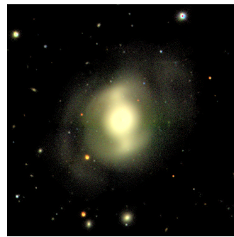
NGC 936: SB0
