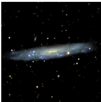
NGC 5496: Sc
