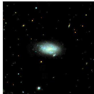
NGC 4668: Irr
