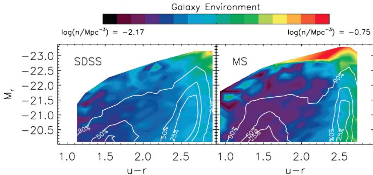
FIG. 5.—Color-magnitude diagram for SDSS and MS galaxies in the left and right panels, respectively. The labeled white lines show which regions on the plot are most populated (these are complete volume-limited samples), and the color-coded background shows the median local environment around galaxies with a given color and magnitude (dark corresponds to low densities; bright corresponds to high densities).
