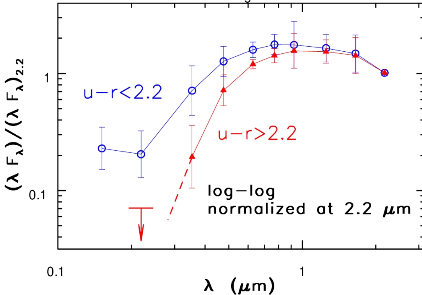
GALEX/SDSS/2MASS SEDs of galaxies
