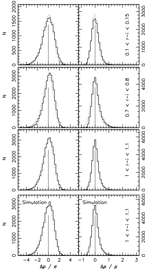
FIG. 29.— Left column: Poisson noise-normalized distribution of residuals in three-dimensional ( X, Y, Z ) pixels for three representative color bins. Right column: Model-normalized distribution of residuals in each pixel, (\text{data} - \text{model})/\text{model} . The black solid-line histograms show the data, while the red dotted-line histograms show the expectation from residuals due to Poisson noise only. The bottom row shows the same distributions derived from a Monte Carlo-simulated catalog, with 25% unresolved binary fraction, \sigma_M = 0.3 parallax dispersion, and SDSS photometric errors. [See the electronic edition of the Journal for a color version of this figure.]
