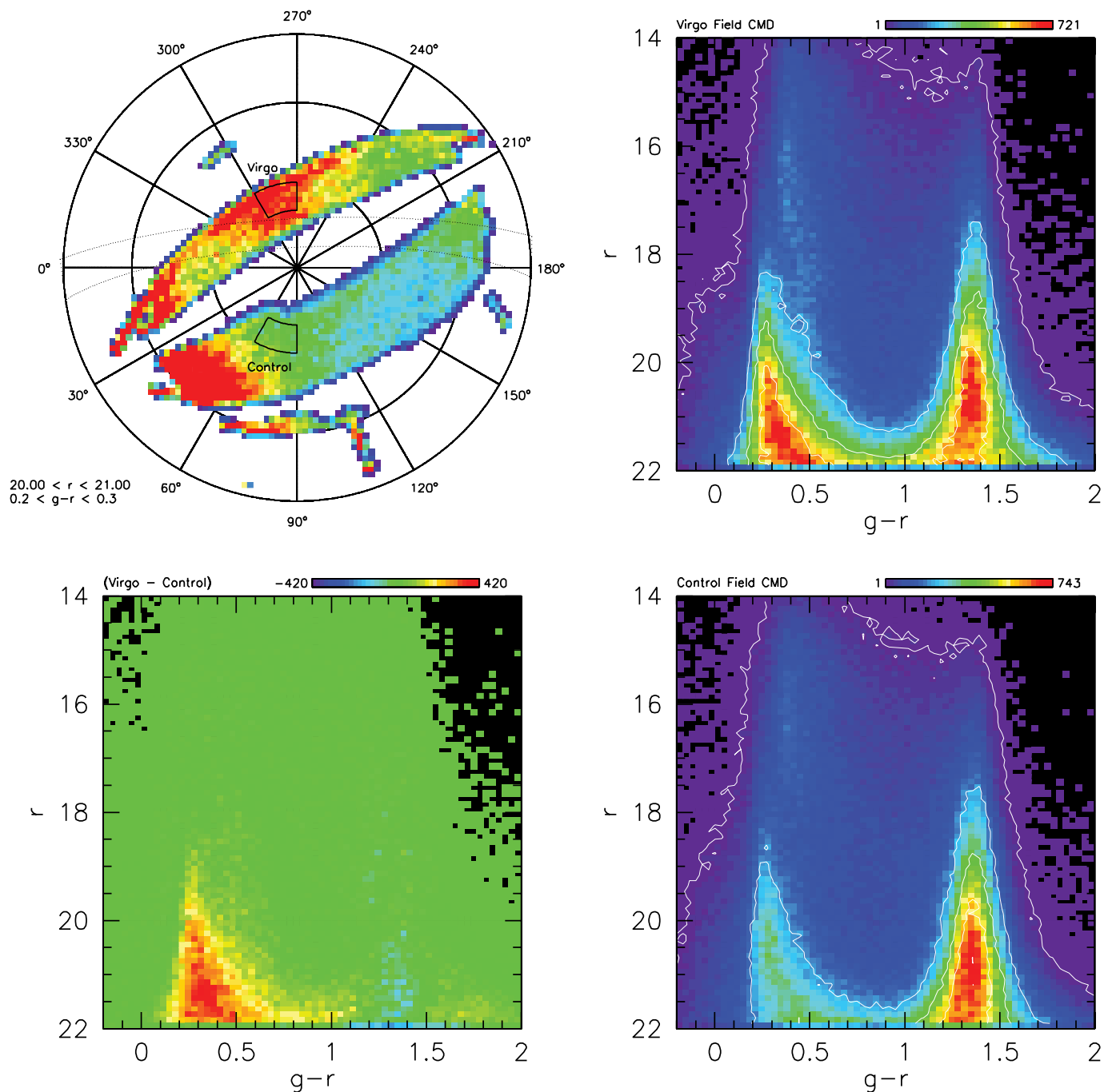
FIG. 37.— Top left : Sky density of stars with b > 0^\circ , 0.2 < g-r < 0.3 , and 20 < r < 21 in the Lambert projection (concentric circles correspond to constant Galactic latitude; equal area corresponds to equal solid angle on the sky) of Galactic coordinates (the north Galactic pole is in the center, l = 0 is toward the left, and the outermost circle is b = 0^\circ ). The number density is encoded with a rainbow color map and increases from blue to red. Note that the sky density distribution is not symmetric with respect to the horizontal l = 0, 180 line. When the stellar color range is sufficiently red (e.g., 0.9 < g-r < 1.0 ), this asymmetry disappears (not shown). Right column : Hess diagrams for two 540 \text{ deg}^2 large regions toward ( l = 300^\circ , b = 60^\circ ; top ) and ( l = 60^\circ , b = 60^\circ ; bottom ), marked as polygons in the top left panel. Bottom left : Difference between these Hess diagrams; note the strong statistically significant overdensity at g-r \sim 0.3 and r \gtrsim 20 . The pixel size in each of the three Hess diagrams is (d(g-r), dr)t = (0.033, 0.1) .
