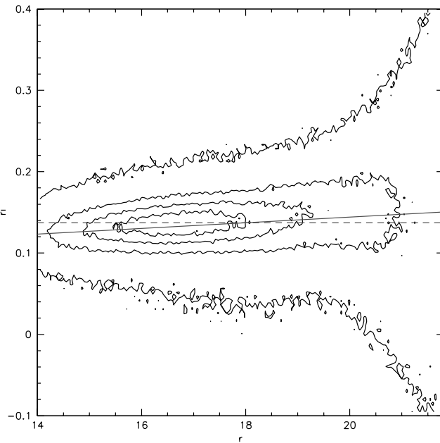
FIG. 45.—Dependence of the measured r - i color on the r -band magnitude for stars with 0.29 < g - r < 0.31 . An approximately linear dependence, with d(r - i)/dr \sim 0.007 mag/mag is observed (solid line). The horizontal dashed line shows the location of the locus for this bin as given by eq. (4). The two match for r = 18 . [See the electronic edition of the Journal for a color version of this figure.]
