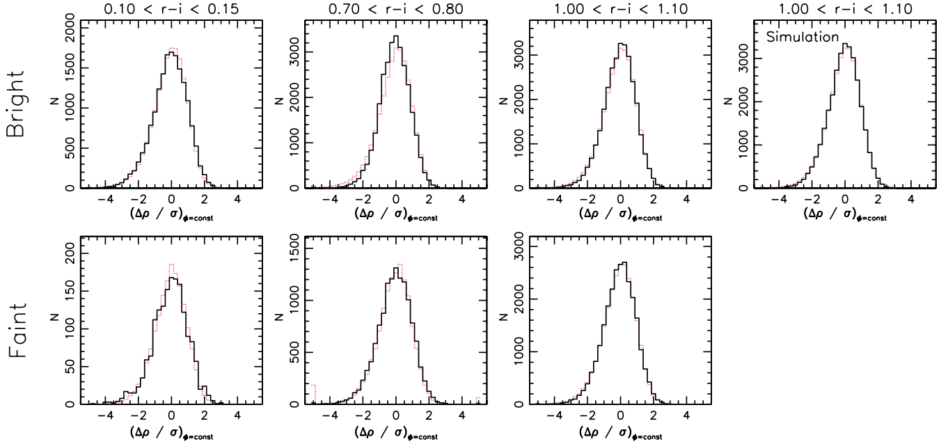
FIG. 25.—Distribution of noise-normalized deviations of density in pixels (X, Y, Z) from the mean density measured along their corresponding annuli [R = (X^2 + Y^2)^{1/2}, Z] . Black solid-line histogram shows the data. Red dotted-line histogram shows a Poisson noise model. Histograms in the top and bottom rows have been calculated assuming the bright (eq. [2]) and faint (eq. [1]) photometric parallax relation, respectively. The rightmost panel in the top row shows the same distributions derived from a Monte Carlo-simulated catalog, with 25% unresolved binary fraction, \sigma_{M_r} = 0.3 parallax dispersion, and SDSS photometric errors.
