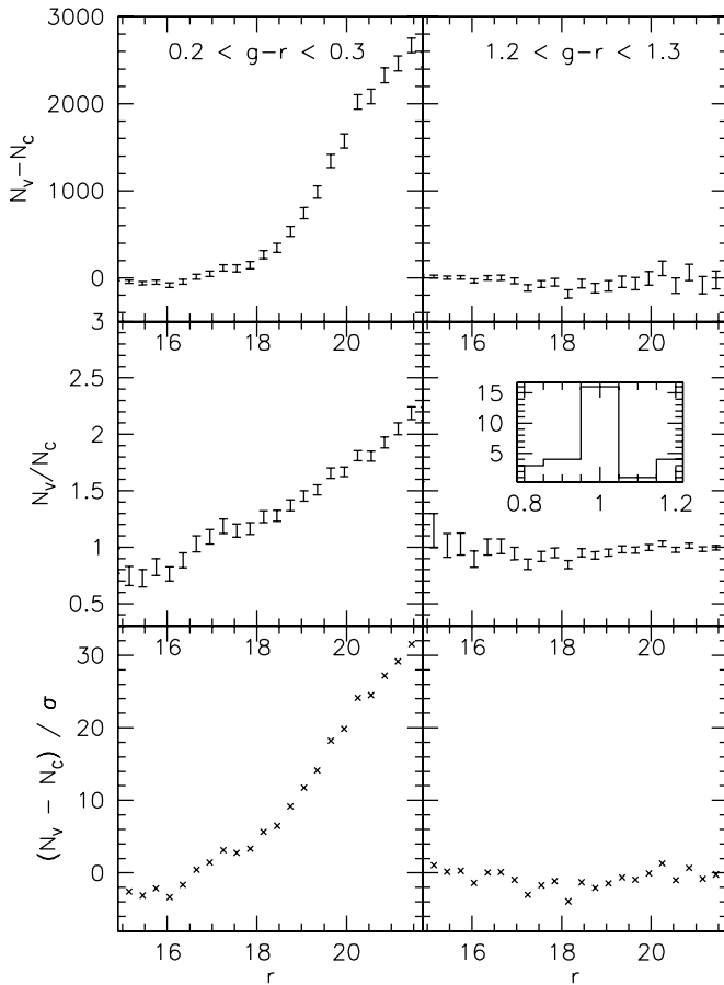
FIG. 38.—Quantitative analysis of the Hess diagram difference shown in the bottom left panel in Fig. 37. The left column corresponds to the color bin 0.2 < g-r < 0.3 that is representative of the Virgo overdensity, and the right column is a control sample with stars satisfying 1.2 < g-r < 1.3 . The top panels show the counts difference as a function of apparent magnitude, and the middle panels show the counts ratio. The inset in the middle right panel shows a histogram of the counts ratio for r < 21.5 . The bottom panels show the counts difference normalized by the expected Poisson fluctuations. Note that for red stars the counts are indistinguishable, while for blue stars the difference is highly statistically significant.
