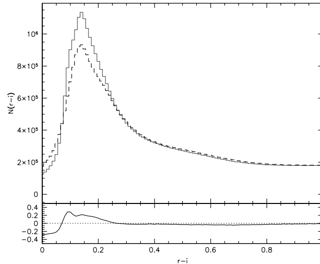
FIG. 44.—Comparison of the number of stars per r-i bin for observed r-i (dashed-line histogram) and the locus-corrected (r-i)_e colors (solid-line histogram) for the 48 million stars in our star catalog. In the regions of maximal gradients, the locus projection has a \sim 20\% effect on the total number of stars per r-i bin. Not including this correction would similarly bias the density normalization of Galactic models. [See the electronic edition of the Journal for a color version of this figure.]
