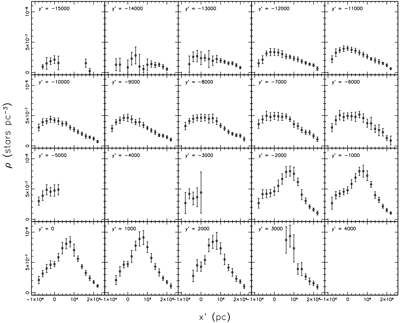
FIG. 36.—Distribution of stellar number density for 0.10 < r - i < 0.15 color bin at Z = 10 kpc above the Galactic plane. Each panel shows a narrow Y' cross section in coordinate system defined by \phi = 30^\circ (see the caption of Fig. 35). Note a clear and strong density excess around X' \sim 8 kpc in Y' > 0 panels, coming from the Virgo overdensity.
