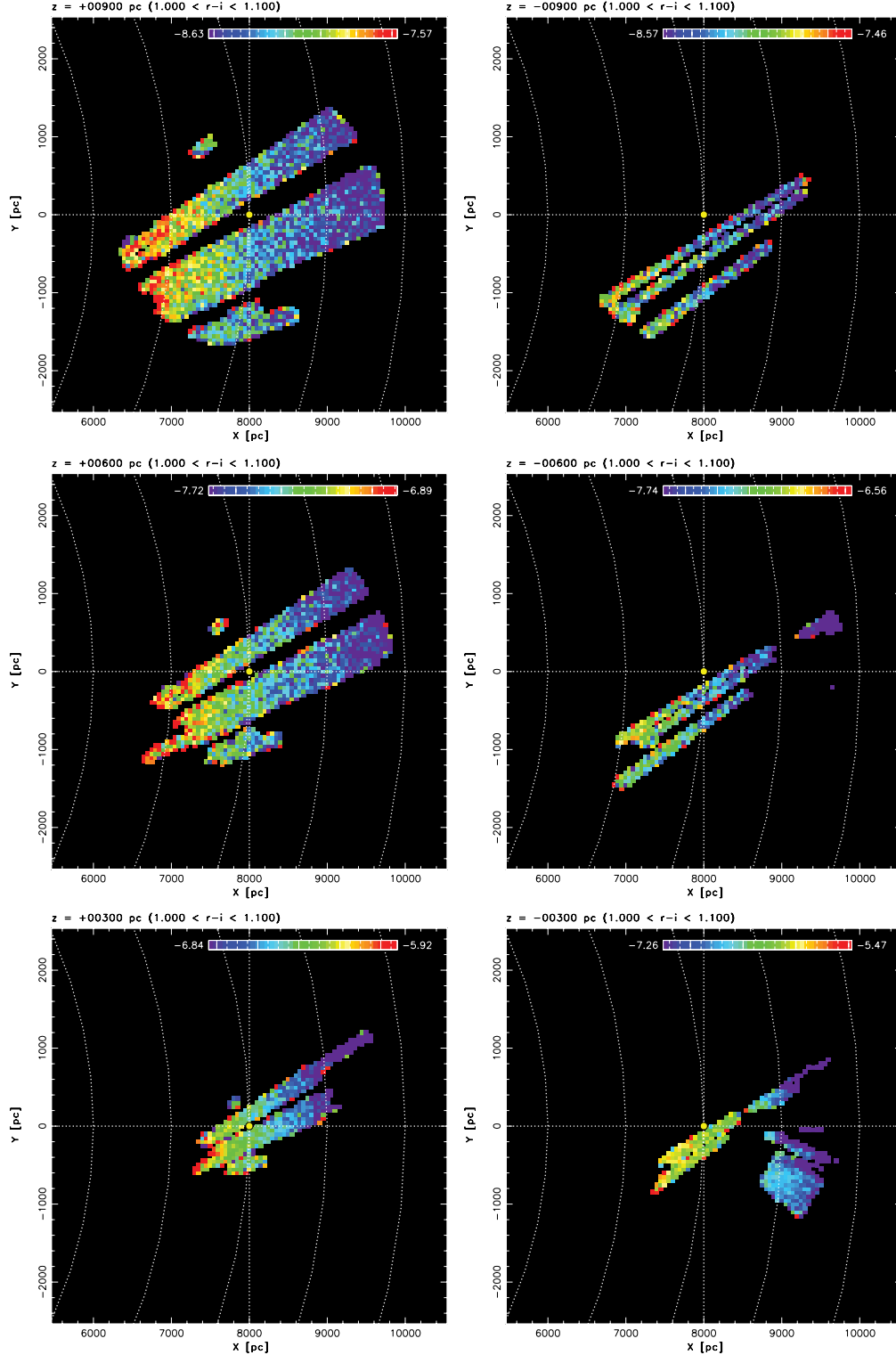
FIG. 14.— Same as Fig. 12, except that here three symmetric slices at Z = 300, 600 , and 900 pc above and below the plane are shown, for the 1.00 < r-i < 1.10 color bin. Note that at these distance scales there is no obvious discernible substructure in the density distribution.
