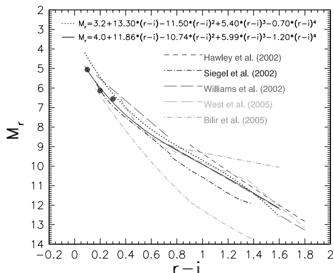
FIG. 2.— Comparison of photometric parallax relations in the SDSS ugriz system from the literature and adopted in this work. The two relations adopted here are shown by the dotted (“bright” normalization) and solid (“faint” normalization) lines. Other lines show photometric parallax relations from the literature, as marked. The bottom thin line from Siegel et al. corresponds to low-metallicity stars. The large symbols show SDSS observations of globular cluster M13. [See the electronic edition of the Journal for a color version of this figure.]
