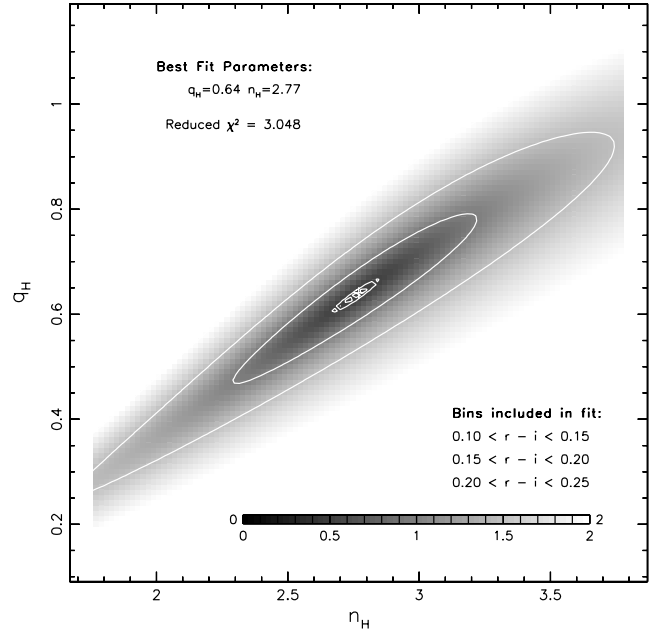
FIG. 22.—Reduced \chi^2 surface of halo parameters n_H and q_H around the best-fit values (Table 5, first row). The innermost contour is at the 1.1\chi^2_{\min} level, while the rest are logarithmically spaced in steps of 0.5 dex, starting at \log \chi^2 = 0.5 .
