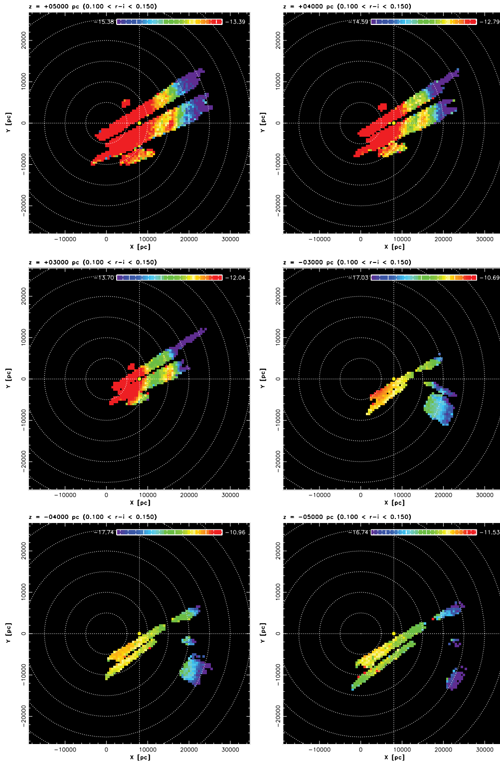
FIG. 13.— Same as Fig. 12, except that three symmetric slices at Z = 3, 4 , and 5 kpc above and below the plane are shown. The color stretch in panels for Z = 3, 4 , and 5 kpc is optimized to bring out the Monoceros overdensity at R \sim 16 kpc and Y \sim 0 .
