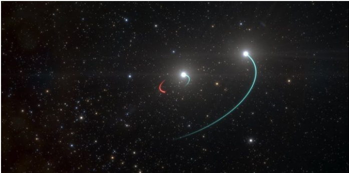
The Closest Black Hole We’ve Ever Discovered
