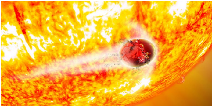
A Solar System Dies, and Necroplanetology Is Born
