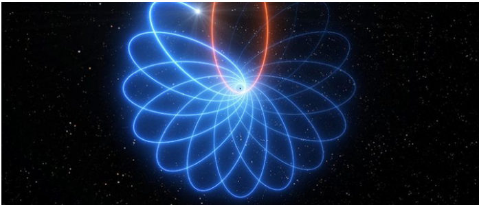
Black Hole-Orbiting Star Proves Einstein Right
