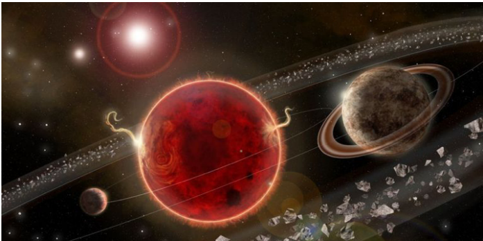
We Might Have an Image of the Exoplanet Proxima c
