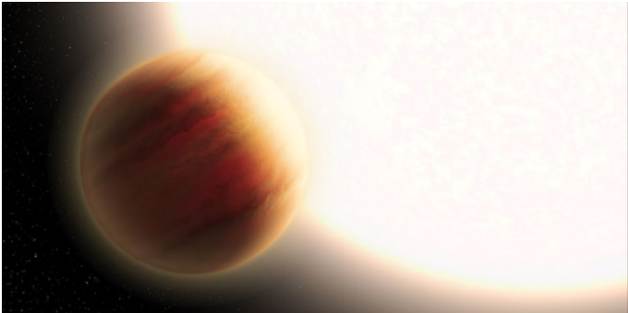
Why Does This Exoplanet Have a Bright Yellow Sky?
