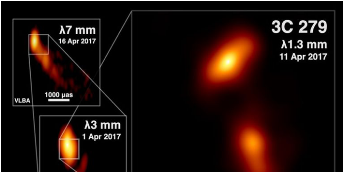
The First-Ever Image of a Black Hole-Powered Jet
