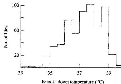
Fig. 2. A histogram of frequency of upper knock-down temperatures for a sample ( n=602 ) of male Drosophila melanogaster .
