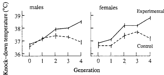
Fig. 3. Mean knock-down temperatures ( \pm 1 SE) of males from selected and control lines of Drosophila melanogaster at generations 0 through 4 of selection (top 25%) on knock-down resistance to heat. Knock-down temperatures ( T_{kd} ) responded rapidly to selection, such that T_{kd} of the selected line increased by about 1.5°C relative to that of the control line.
