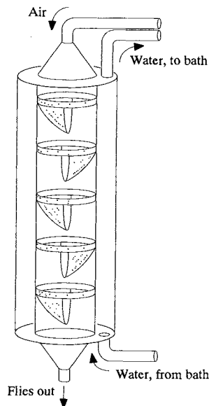
Fig. 1. Apparatus for measuring and 'fractionating' small arthropods by knock-down resistance to heat or cold. The study animals are first put into the top of the column, and the temperature within the column then warmed (or cooled) by pumping water (ethylene glycol) from a temperature-controlled bath through the surrounding water jacket. When the animals reach an incapacitating body temperature (knock-down temperature), they fall out of the column into collecting vials below. Knock-down temperatures of small insects are closely approximated (see Appendix) by measuring air temperature within the column.
