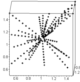
Fig A1: Inequality Constraint Function Level Sets i_h = -1 and i_h = 0 in price space \pi
