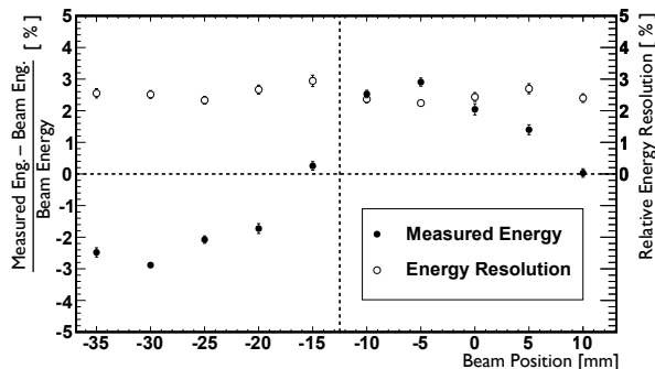
Figure 14: The measured energy and energy resolution in a 3 \times 4 array of white-wrapped crystals during a position scan with a 3.1-GeV beam. A vertical dotted line is drawn along a crystal boundary and a horizontal dotted line is drawn along the mean measured energy of 3.1 GeV.
