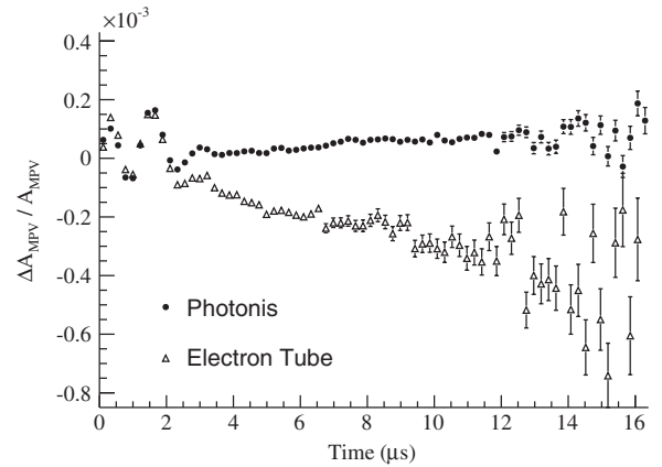
FIG. 14. Fractional MPV change versus the hit time in the measurement period. The solid circles correspond to the amplitude variation of tiles with Photinis PMTs and the open triangles correspond to the amplitude variation of tiles with Electron Tube PMTs.
