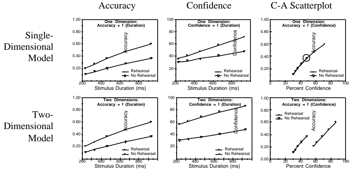
Figure 2: Predictions of the two Models
