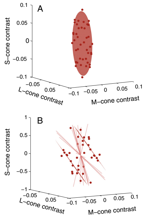
Fig. 2. Isoresponse surfaces from two V1 neurons. See (Horwitz and Hass, 2012) for methodological details. In each plot, the origin represents a blank gray screen, and distance from the origin represents contrast. Points represent stimuli that caused the neuron to discharge a criterion number of spikes. Points and surface fits are constrained to be symmetric about the origin because the stimuli used in the experiment were symmetric modulations through gray. (A) Isoresponse surface from a neuron that responded in every color direction tested. (B) Isoresponse surface from a neuron that responded to the sum of L- and M-cone contrasts. Radial lines in B represent directions in the stimulus space in which a criterion response could not be measured. Note the difference in y-axis scale between A and B.
