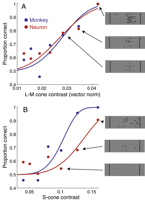
Fig. 1. Chromatic detection functions for a single V1 neuron (red) and a rhesus macaque (blue). See (Hass and Horwitz, 2013) for methodological details. In randomly interleaved trials, the stimulus was an antiphase modulation of the L- and M-cones (A) or a modulation of the S-cones alone (B). Neurometric sensitivity was quantified by an ideal observer analysis on the measured spike counts. Example rasters for the three highest contrast stimuli are shown (right).
