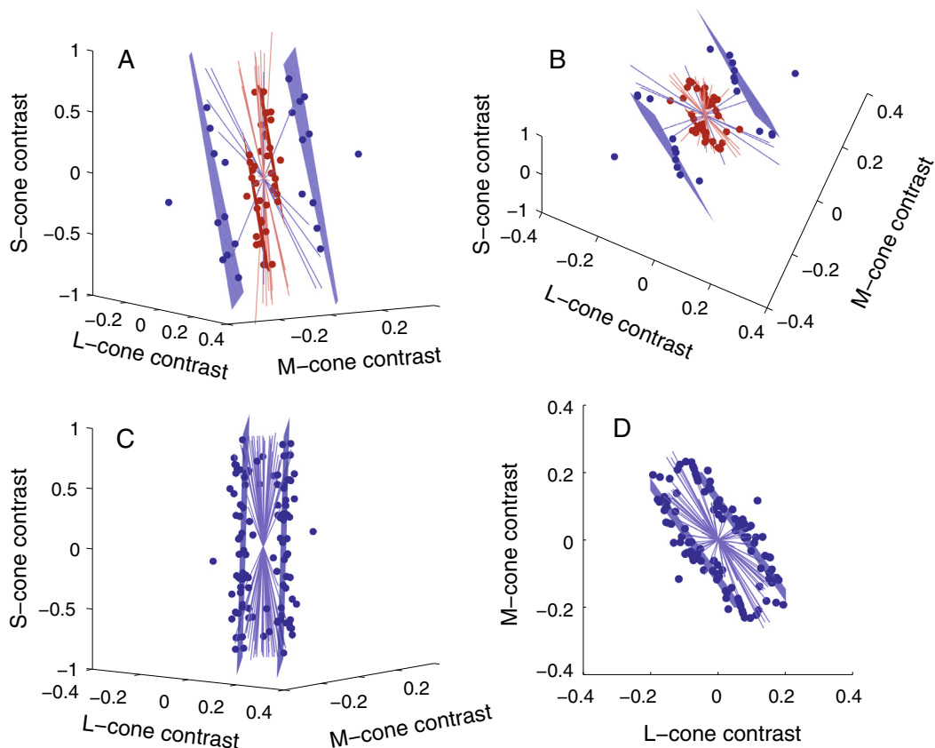
Fig. 3. Isodetectability planes for a macaque (A and B) and a human (C and D). Blue points represent stimuli at the observer's detection threshold, blue lines are color directions in which detection thresholds could not be measured, and planes are fits to these data. Red points and planes are redrawn from Fig. 2B to illustrate the similarity in orientation between neuronal isoresponse planes and macaque isodetectability planes. Data in A and B are identical but are shown from different viewing angles (and similarly, C and D). The stimulus used in the psychophysical experiments modulated at 25 Hz for the macaque and at 15 Hz for the human.
