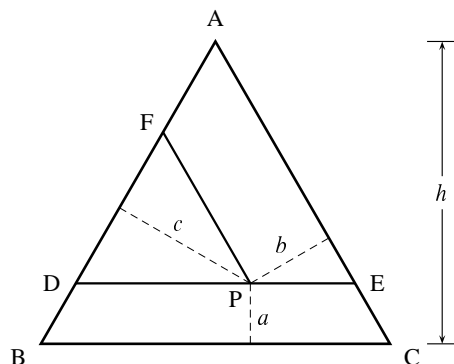
Figure 13.16 Proof that the sum of the lengths a , b , and c is equal to the height h of the large equilateral triangle ABC . ADE and FDP are two smaller equilateral triangles. The height of triangle ADE is equal to h - a . The height of triangle FDP is equal to the height of triangle ADE minus length b , and is also equal to length c : h - a - b = c . Therefore, a + b + c = h .
