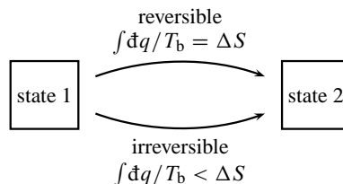
Figure 4.12 Reversible and irreversible paths between the same initial and final equilibrium states of a closed system. The value of \Delta S is the same for both paths, but the values of the integral \int (\dot{d}q/T_b) are different.
