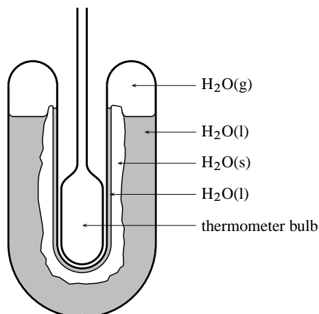
Figure 2.5 Cross-section of a water triple-point cell. The cell has cylindrical symmetry. Pure water of the same isotopic composition as \text{H}_2\text{O} in ocean water is distilled into the cell. The air is pumped out and the cell is sealed. A freezing mixture is placed in the inner well to cause a thin layer of ice to form next to the inner wall. The freezing mixture is removed, and some of the ice is allowed to melt to a film of very pure water between the ice and inner wall. The thermometer bulb is placed in the inner well as shown, together with ice water (not shown) for good thermal contact.
