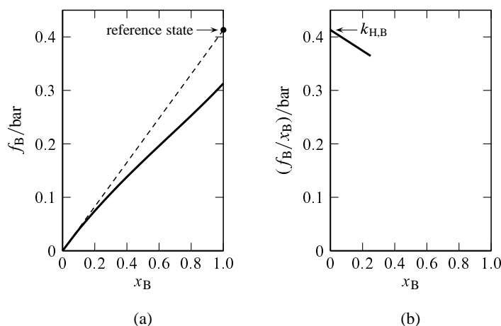
Figure 9.7 Liquid solutions of 2,3-dimethylbutane (B) in cyclooctane at 298.15 K and 1 bar. a
