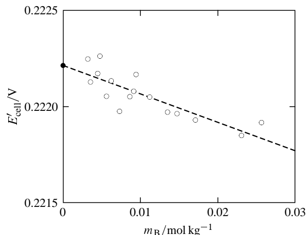
Figure 14.5 E'_{\text{cell}} (defined by Eq. 14.5.2) as a function of HCl molality for the cell of Fig. 14.1 at 298.15 K. a The dashed line is a least-squares fit to a linear relation.
