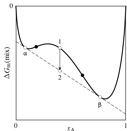
Figure 11.4 Molar Gibbs energy of mixing as a function of the composition of a binary liquid mixture with spontaneous phase separation. The inflection points are indicated by filled circles.
