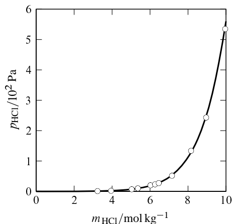
Figure 10.1 Partial pressure of HCl in a gas phase equilibrated with aqueous HCl at 25 °C and 1 bar. Open circles: experimental data from Ref. [5].
