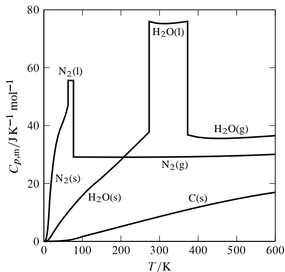
Figure 7.5 Temperature dependence of molar heat capacity at constant pressure ( p = 1 bar) of \text{H}_2\text{O} , \text{N}_2 , and \text{C}(\text{graphite}) .
