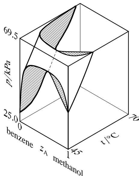
Figure 13.9 Liquidus and vaporus surfaces for the binary system of methanol (A) and benzene. a Cross-sections are hatched in the direction of the tie lines. The dashed curve is the azeotrope vapor-pressure curve.
