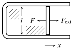
Figure 5.1 Device to measure the surface tension of a liquid film. The film is stretched between a bent wire and a sliding rod.
