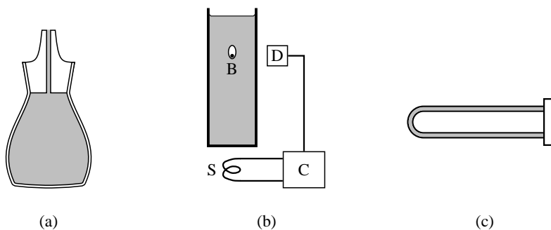
Figure 2.4 Three methods for measuring liquid density by comparison with samples of known density. The liquid is indicated by gray shading.
