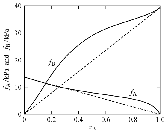
Figure 12.11 Fugacities in a gas phase equilibrated with a binary liquid mixture of chloroform (A) and ethanol (B) at 35 °C (Ref. [149]).
