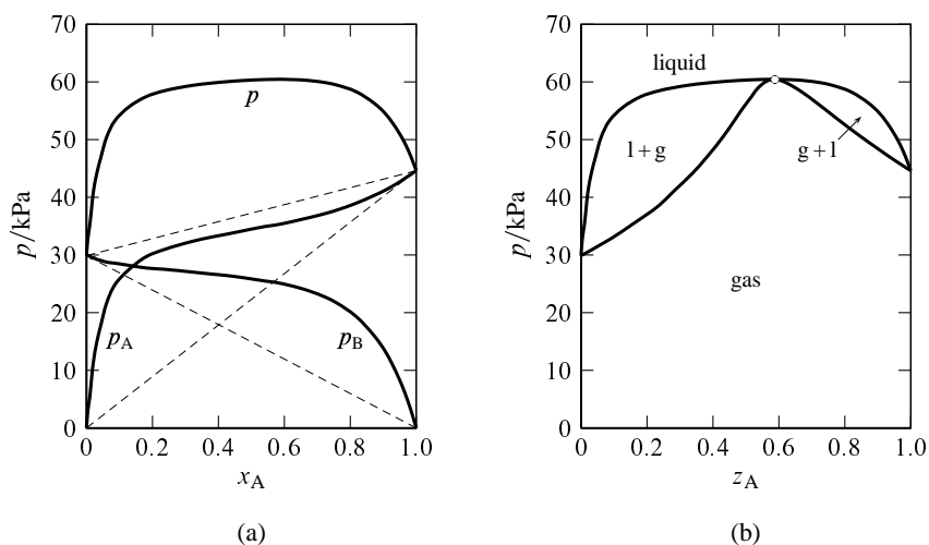
Figure 13.8 Binary system of methanol (A) and benzene at 45 °C. a
