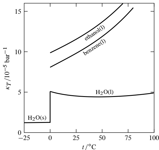
Figure 7.2 The isothermal compressibility of several substances as a function of temperature at p = 1 bar. (Based on data in Ref. [49]; Ref. [88]; and Ref. [167], p. 28.)
