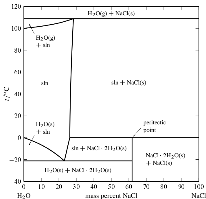
Figure 13.4 Temperature–composition phase diagram for the binary system of \text{H}_2\text{O} and \text{NaCl} at 1 bar. (Data from Refs. [37] and [167].)
