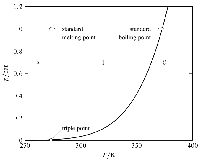
Figure 8.6 Pressure–temperature phase diagram of \text{H}_2\text{O} . (Based on data in Ref. [124].)
