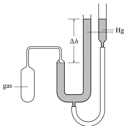
Figure 2.6 Simple version of a constant-volume gas thermometer.
