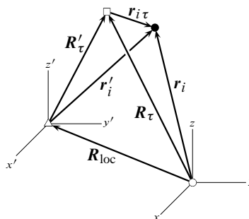
Figure G.3 Vectors in the lab and local reference frames. Open circle: origin of lab frame; open triangle: origin of local frame; open square: point fixed in system boundary at segment \tau ; filled circle: particle i . The thin lines are the Cartesian axes of the reference frames.
