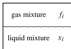
Figure 9.6 Equilibrated liquid and gas mixtures. Substance i is present in both phases.
