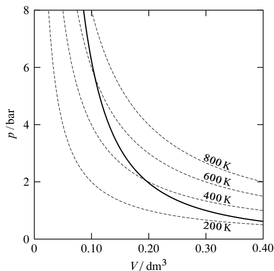
Figure 3.6 An adiabat (solid curve) and four isotherms (dashed curves) for an ideal gas ( n = 0.0120 mol, C_{V,m} = 1.5R ).
