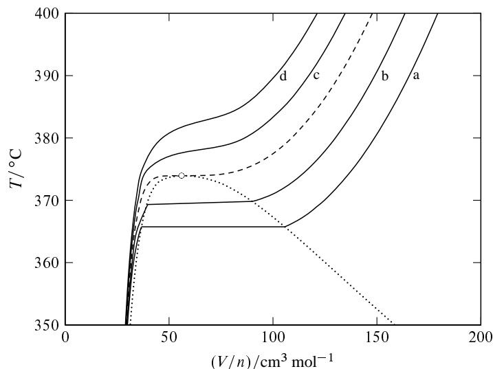
Figure 8.11 Isobars for the fluid phases of \text{H}_2\text{O} . a The open circle indicates the critical point, the dashed curve is the critical isobar at 220.64 bar, and the dotted curve encloses the two-phase area of the temperature–volume phase diagram.
