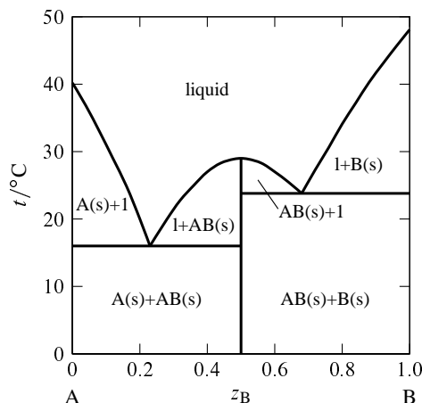
Figure 13.3 Temperature–composition phase diagram for the binary system of \alpha -naphthylamine (A) and phenol (B) at 1 bar (Ref. [128]).
