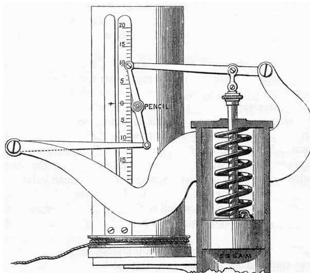
Figure 3.7 Indicator with paper-covered roll at left and pressure gauge at right. a
