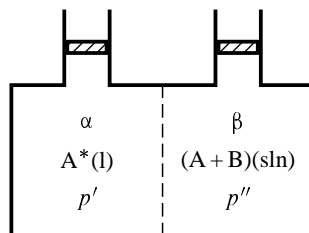
Figure 12.2 Apparatus to measure osmotic pressure (schematic). The dashed line represents a membrane permeable only to the solvent A. The cross-hatched rectangles represent moveable pistons.
