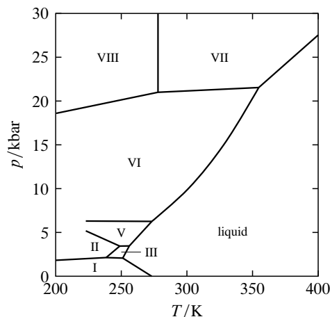
Figure 8.4 High-pressure pressure–temperature phase diagram of \text{H}_2\text{O} . a The roman numerals designate seven forms of ice.
