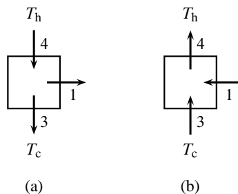
Figure 4.5 (a) One cycle of a Carnot engine that does work on the surroundings.
