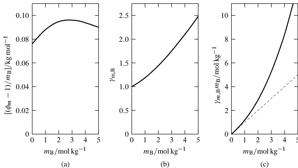
Figure 9.11 Aqueous sucrose solutions at 25 °C. a
