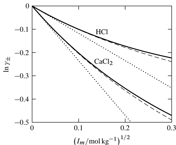
Figure 10.4 Dependence of \ln \gamma_{\pm} on \sqrt{I_m} for aqueous HCl (upper curves) and aqueous \text{CaCl}_2 (lower curves) at 25°C. a Solid curves: experimental; dashed curves: Debye–Hückel equation ( a = 5 \times 10^{-10} m for HCl, a = 4.5 \times 10^{-10} m for \text{CaCl}_2 ); dotted lines: Debye–Hückel limiting law.
