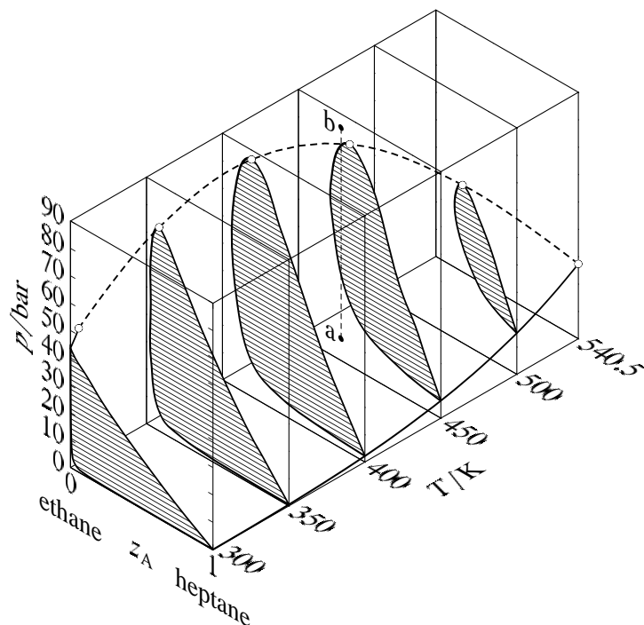
Figure 13.13 Pressure–temperature–composition behavior in the binary heptane–ethane system. a The open circles are critical points; the dashed curve is the critical curve. The dashed line a–b illustrates retrograde condensation at 450 K.
