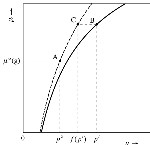
Figure 7.6 Chemical potential as a function of pressure at constant temperature, for a real gas (solid curve) and the same gas behaving ideally (dashed curve). Point A is the gas standard state. Point B is a state of the real gas at pressure p' . The fugacity f(p') of the real gas at pressure p' is equal to the pressure of the ideal gas having the same chemical potential as the real gas (point C).
