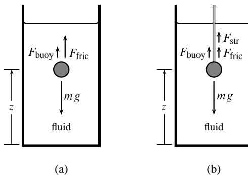
Figure 3.9 Spherical body (shaded) in a gravitational field. The arrows indicate the directions and magnitudes of contact and gravitational forces exerted on the body. (a) The body falls freely through a fluid in a vessel. (b) The body is lowered on a string through the fluid.
