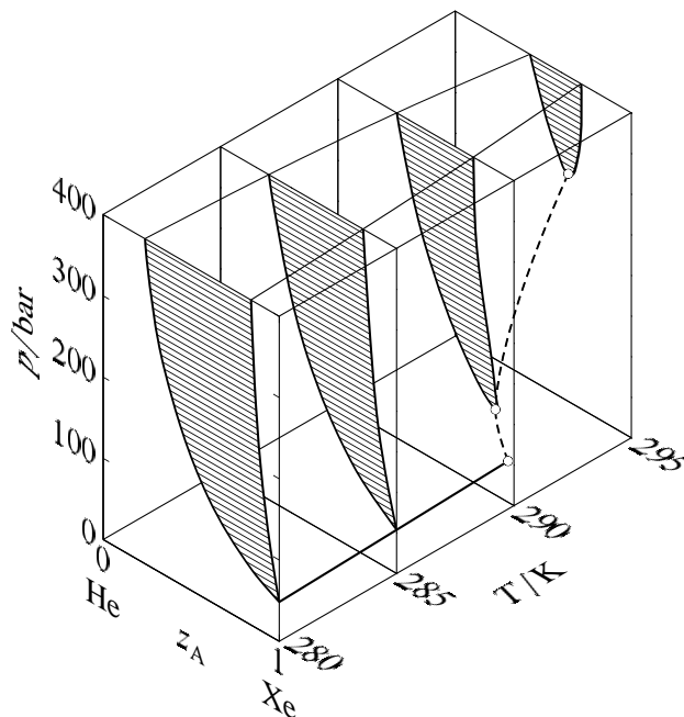
Figure 13.14 Pressure–temperature–composition behavior in the binary xenon–helium system. a The open circles are critical points; the dashed curve is the critical curve.
