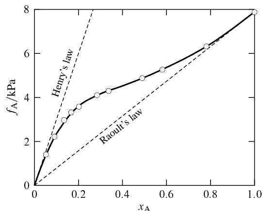
Figure 9.8 Fugacity of ethanol in a gas phase equilibrated with a binary liquid mixture of ethanol (A) and \text{H}_2\text{O} at 25^\circ\text{C} and 1 bar. Open circles: experimental measurements. a The dashed lines show Henry's law behavior and Raoult's law behavior.
