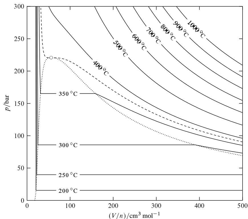
Figure 8.10 Isotherms for the fluid phases of \text{H}_2\text{O} . a The open circle indicates the critical point, the dashed curve is the critical isotherm at 373.95^\circ\text{C} , and the dotted curve encloses the two-phase area of the pressure–volume phase diagram. The triple line lies too close to the bottom of the diagram to be visible on this scale.
