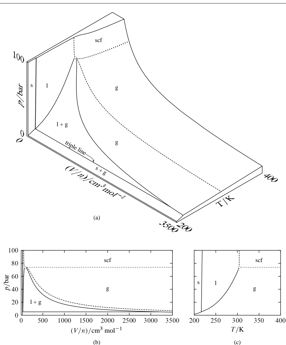
Figure 8.2 Relations among p , V/n , and T for carbon dioxide. a Areas are labeled with the stable phase or phases (scf stands for supercritical fluid). The open circle indicates the critical point.
