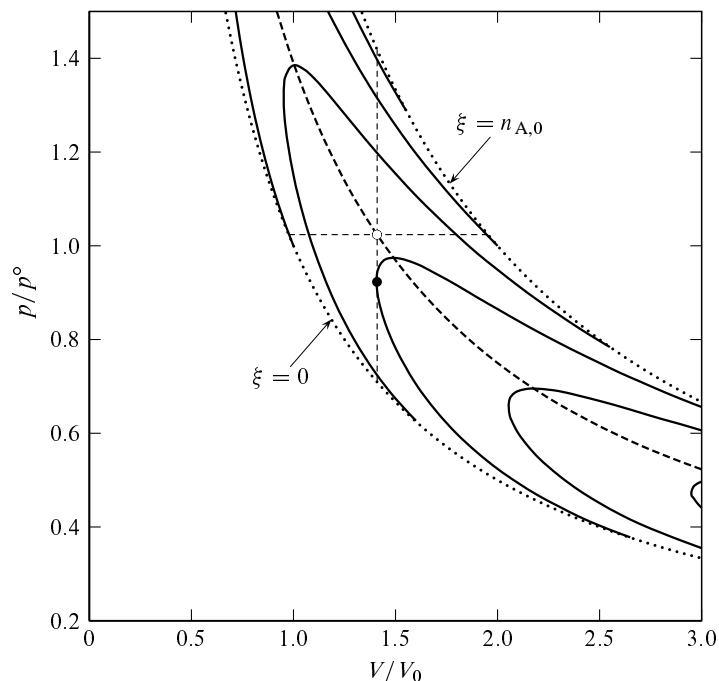
Figure 11.17 Dependence of Gibbs energy on volume and pressure, at constant temperature, in a closed system containing an ideal gas mixture of A and B. The reaction is A \rightarrow 2B with \Delta_r G^\circ = 0 . Solid curves: contours of constant G plotted at an interval of 0.5n_{A,0}RT . Dashed curve: states of reaction equilibrium ( \Delta_r G = 0 ). Dotted curves: limits of possible values of the advancement. Open circle: position of minimum G (and an equilibrium state) at the constant pressure p = 1.02p^\circ . Filled circle: position of minimum G for a constant volume of 1.41V_0 , where V_0 is the initial volume at pressure p^\circ .
