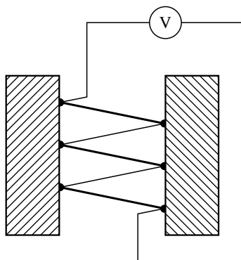
Figure 2.7 A thermopile used to measure the difference in the temperatures of two bodies.
