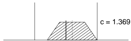
shifted trapezoidal density: a = .5
