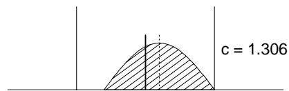
shifted half cosine wave density
