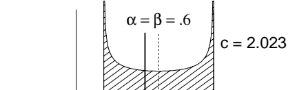
shifted beta density
