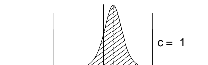
shifted Student t density: df = 4
