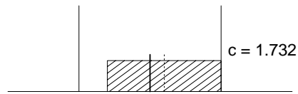
shifted uniform density
