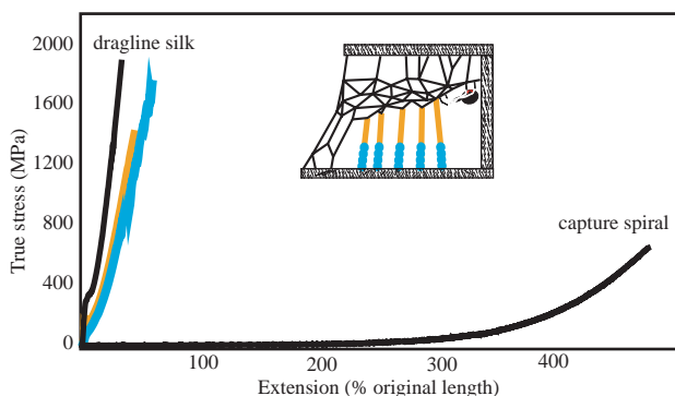
Fig. 3. Plasticization of black widow dragline silk by aqueous glue does not alter the mechanical performance of dragline silk to resemble the mechanical performance of orb-weaver capture spiral. Black curves show the mechanical characteristics of dry dragline and glue-coated capture spiral silks from an orb-web. Representative curves for both dry (orange) and wet (blue) sticky gumfooted silk are shown.
