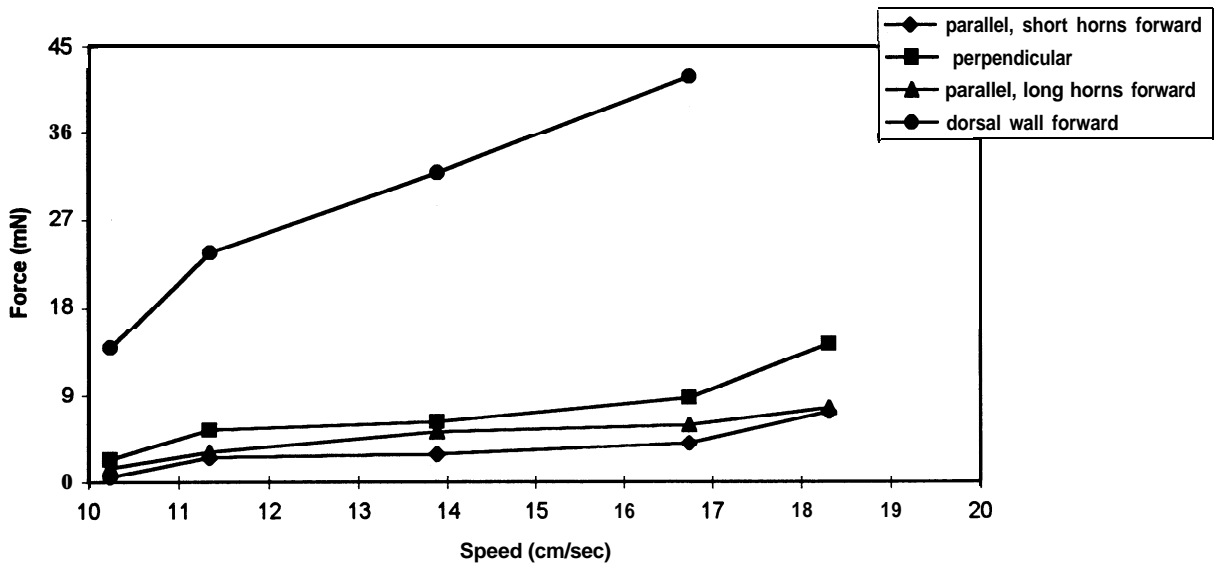
Figure 2. Relative drag measurements on capsules oriented as indicated at various flow speeds. Values presented are means for five capsules. Standard deviations are not shown because the values of the three curves at the bottom are not statistically different.
