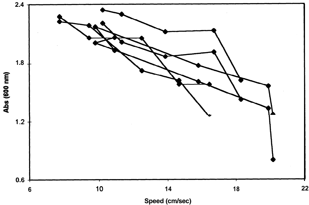
Figure 3. Scatter diagram of the optical absorbance of the methylthymol blue solutions remaining in six capsules after one hour at the indicated speeds. The lines connect the five values for individual capsules.
