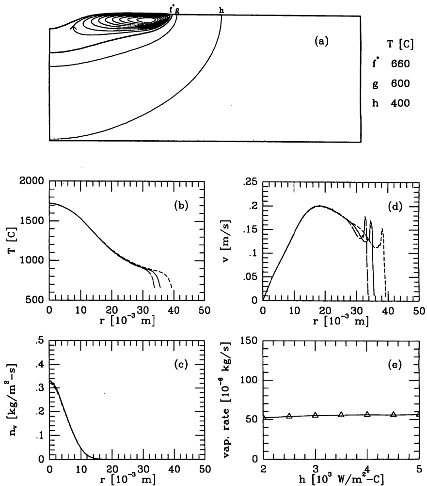
Figure 5. Effects of variations in the platform heat transfer coefficient, h_{pi} . (a) Streamfunction and temperature contours for h_{pi} = 3 \text{ kW m}^{-2} \text{ K}^{-1} . Surface variables in pool area: (b) temperature; (c) vapor flux; (d) velocity for h_{pi} = 3 \text{ kW m}^{-2} \text{ K}^{-1} and M2 mesh (---), h_{pi} = 4 \text{ kW m}^{-2} \text{ K}^{-1} and M2 mesh (—), and h_{pi} = 5 \text{ kW m}^{-2} \text{ K}^{-1} and M2 mesh (- -); (e) vaporization rate versus platform heat transfer coefficient for M1 and M2 meshes (curves coincide to resolution of plot).
