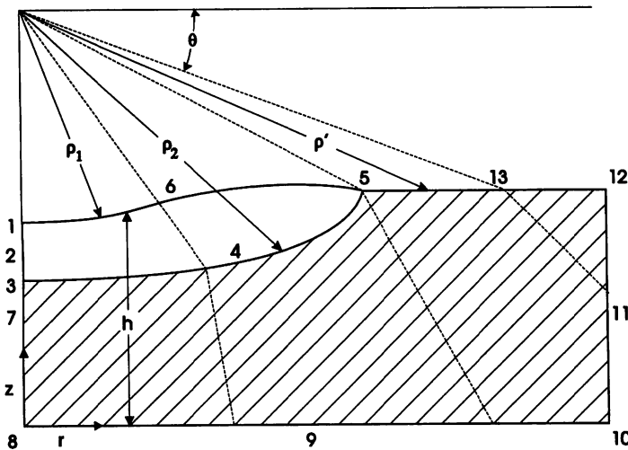
Figure 2. Mesh variables, spines (---) and interfacial segments and endpoints. The interfacial variables and associated conditions are given in Table I.
