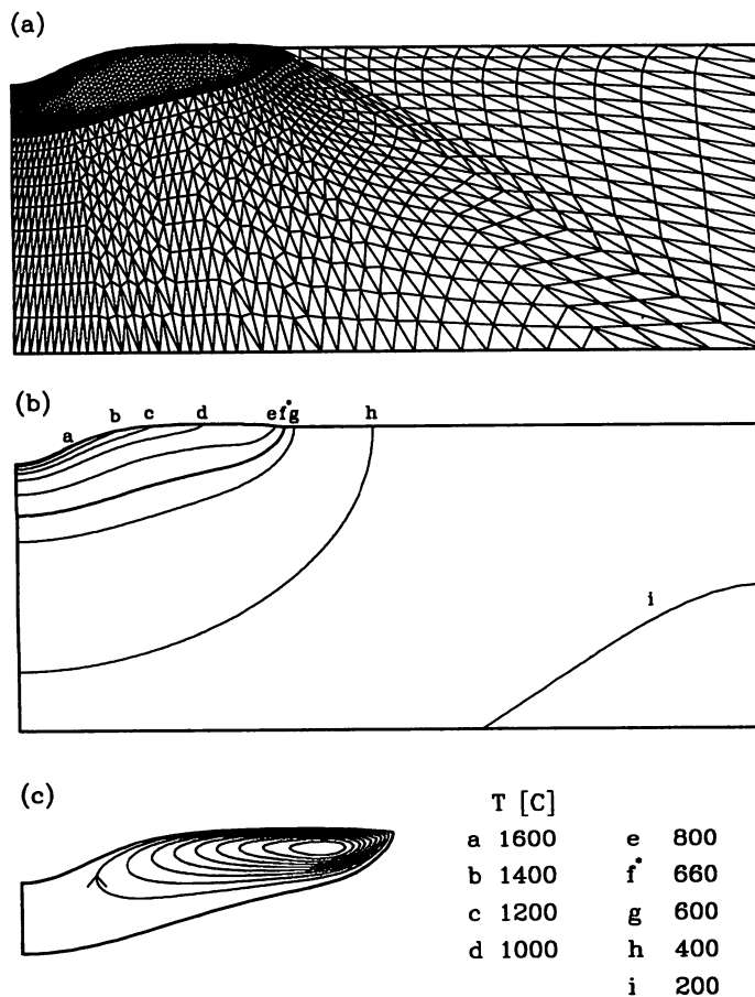
Figure 3. Results for base case (material properties and operating parameters listed in Appendix I and Table II) on mesh M2. (a) Deformed mesh, (b) temperature contours, (c) streamfunction contours.
