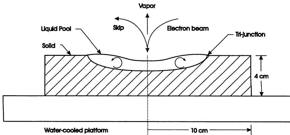
Figure 1. Evaporation of aluminum from a plate on a water-cooled platform.
