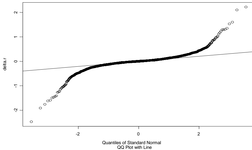
First order change of Weekly 3 Month U.S. T-Bill Rate
