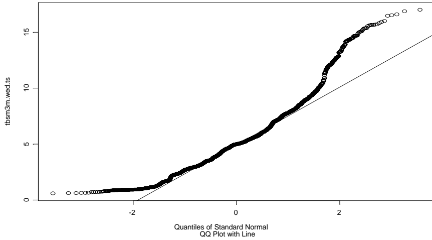
Weekly 3 Month U.S. T-Bill Rate
