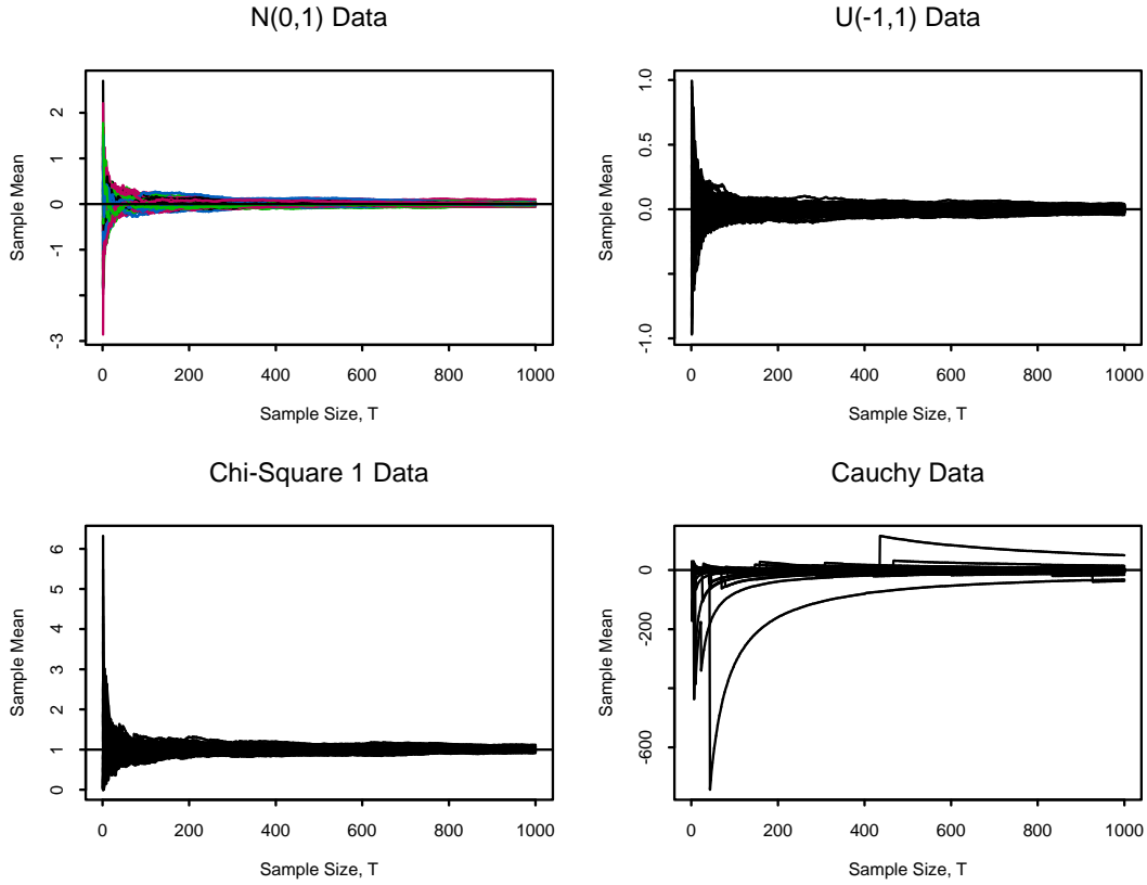
Figure 2: 100 realizations of Y_n = \bar{X} for n = 1, \dots, 1000 .
