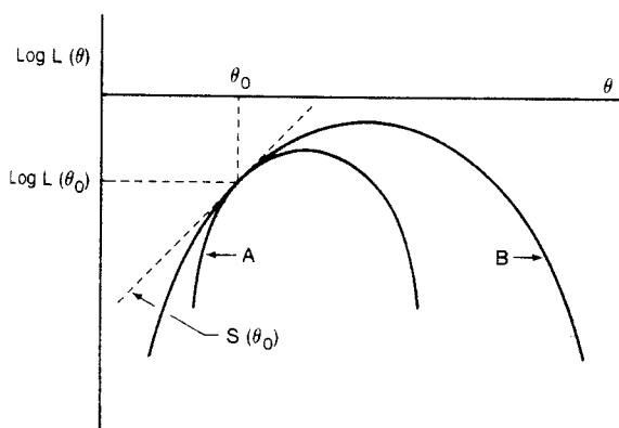
Figure 3. The Lagrange Multiplier Test
