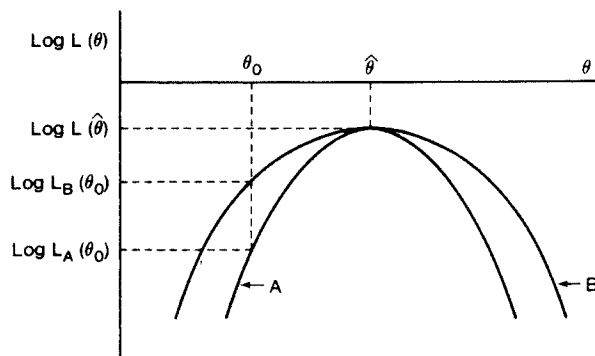
Figure 2. The Wald Test
