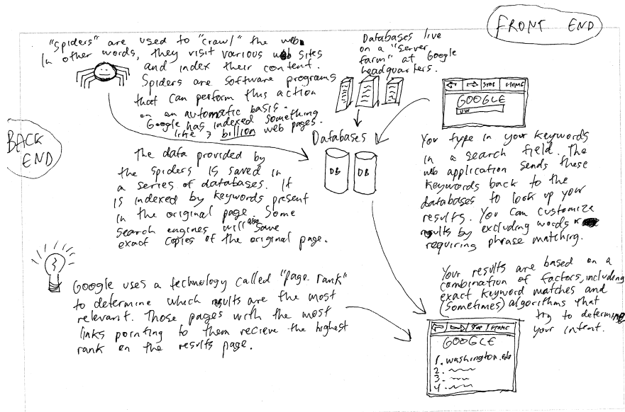
Fig. 15.3. Sketch of search engine that reveals a significant technical maturity, including an explanation of PageRank, approximate size of the WWW, and the complexity of determining a ranking of pages. The sketch segments the process into the front-end and back-end components. The use of visual symbols and user interface representations is noteworthy because to a large degree this visual language supports the written annotations – the reverse of many sketches. Finally, the light bulb, suggesting innovation and intelligence, draws attention to PageRank, a distinguishing characteristic of Google’s matching algorithm.
