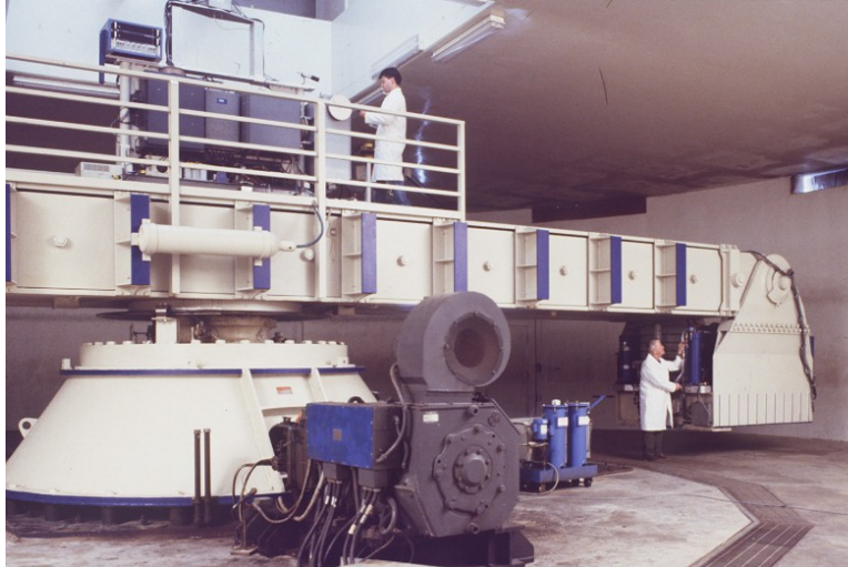
Figure 7. Geotechnical Centrifuge at the University of California, Davis
