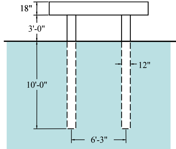
Figure 4. Field Specimen
