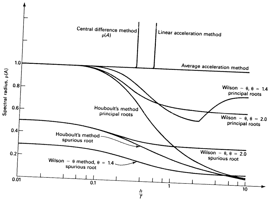
Figure 8.13 Roots of the difference equation.
