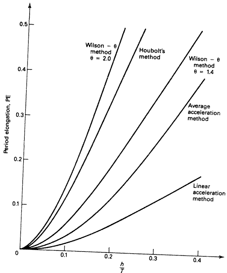
Figure 8.14 Period elongation versus h/T .
