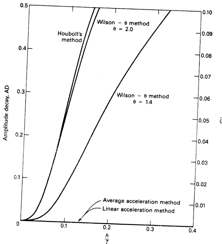
Figure 8.15 Amplitude decay versus h/T .
