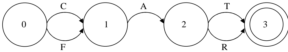
Figure 4: disjunction
