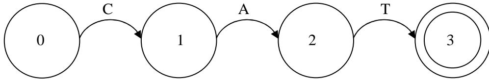
Figure 3: concatenation
