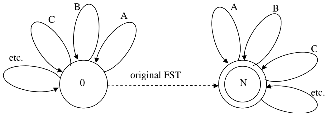
Figure 2: Extending an FSA for use in search
