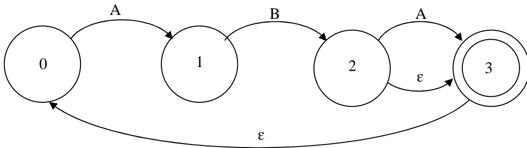
Figure 7: an equivalent NFA
