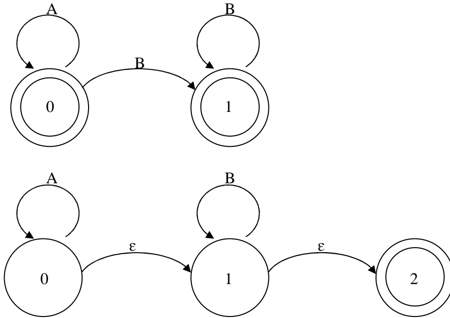
Figure 1: Two ways of doing /A*B*/
