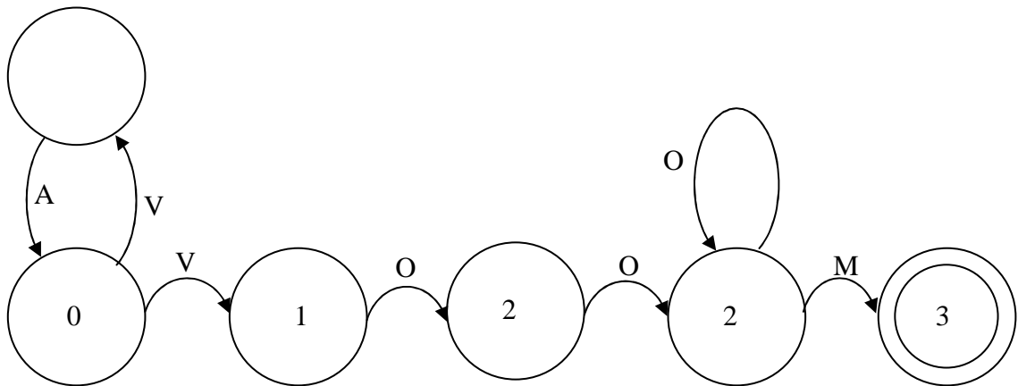
Figure 5: iteration
