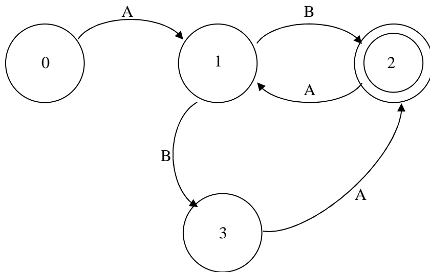
Figure 6: Exercise 2.8
