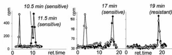
FIGURE 6. Synthesis of complex N-glycans in vitro by incubating E. histolytica membranes with UDP-[ 3 H]Glc and UDP[ 3 H]Gal. A , a Bio-Gel P-4 filtration chromatogram of N-glycans is shown. B , isomer separation by HPAEC in PA100 is shown. ret. , retention. C , identification of the transferred monosaccharide after total hydrolysis by HPAEC in MA1 is shown. The presence of Gal in the Hex 4 isomers and in Hex 5 eluting at 17 min is consistent with the \alpha -galactosidase digests in F . In D – F , untreated glycans are marked with closed circles , and the products of glycosylhydrolases are marked with open circles . D , one Gal 1 Man 3 GlcNAc 2 isomer (H4.3, at 10.5 min) is digested with jack bean \alpha -mannosidase (JBAM), whereas the other isomer (H4.2, at 11.5 min) is not. E , Glc 1 Man 5 GlcNAc 2 (H6.1, at 22 min) is digested to a disaccharide ( asterisk ) by endomannosidase. F , both Gal 1 Man 3 GlcNAc 2 isomers (H4.2 and H4.3 at 10.5 and 11.5 min), as well as Gal 1 Man 4 GlcNAc 2 (H5.2 at 17 min), digest with \alpha -galactosidase. In contrast, Glc 1 Gal 1 Man 3 GlcNAc 2 (H5.6 at 19 min) is not digested by \alpha -galactosidase. G , the table summarizes these results. Isomer H5.2 was fully characterized using complementary data acquired in a separate [ 2 H]Man-labeling experiment (Fig. 2). frct. , fraction; Endomann. , endomannosidase; comp. , composition; ident. , identity.
