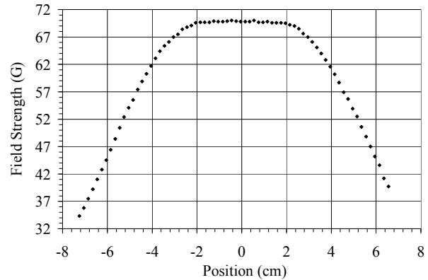
FIG. 3. Helmholtz coils with 16 Amperes of current.
