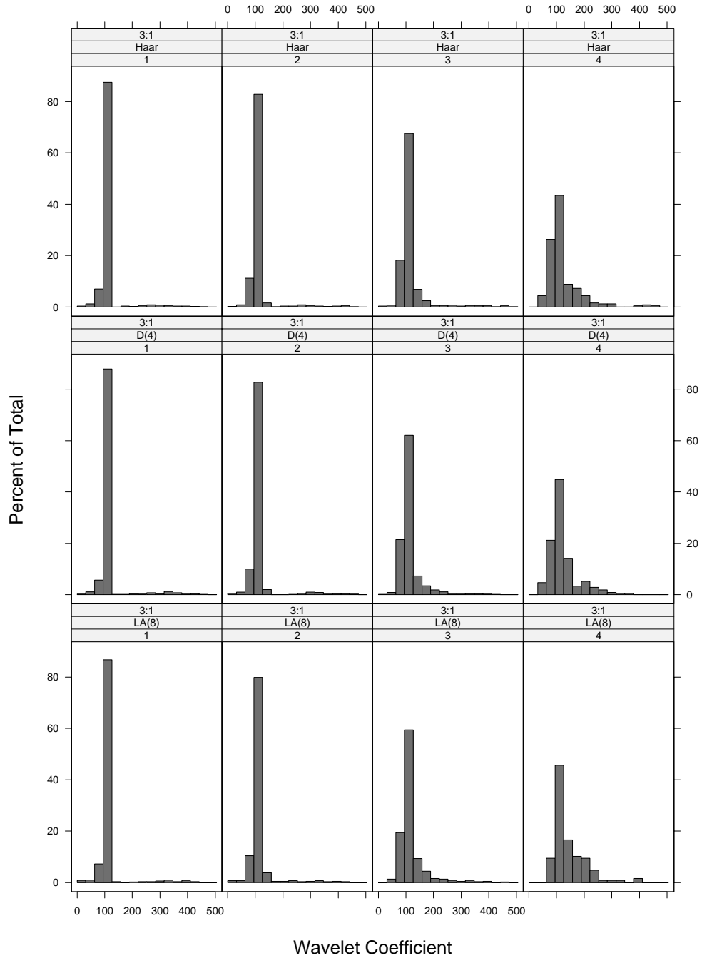
Figure 3: Same as Figure 1 with variance ratio \Delta = 3 .
