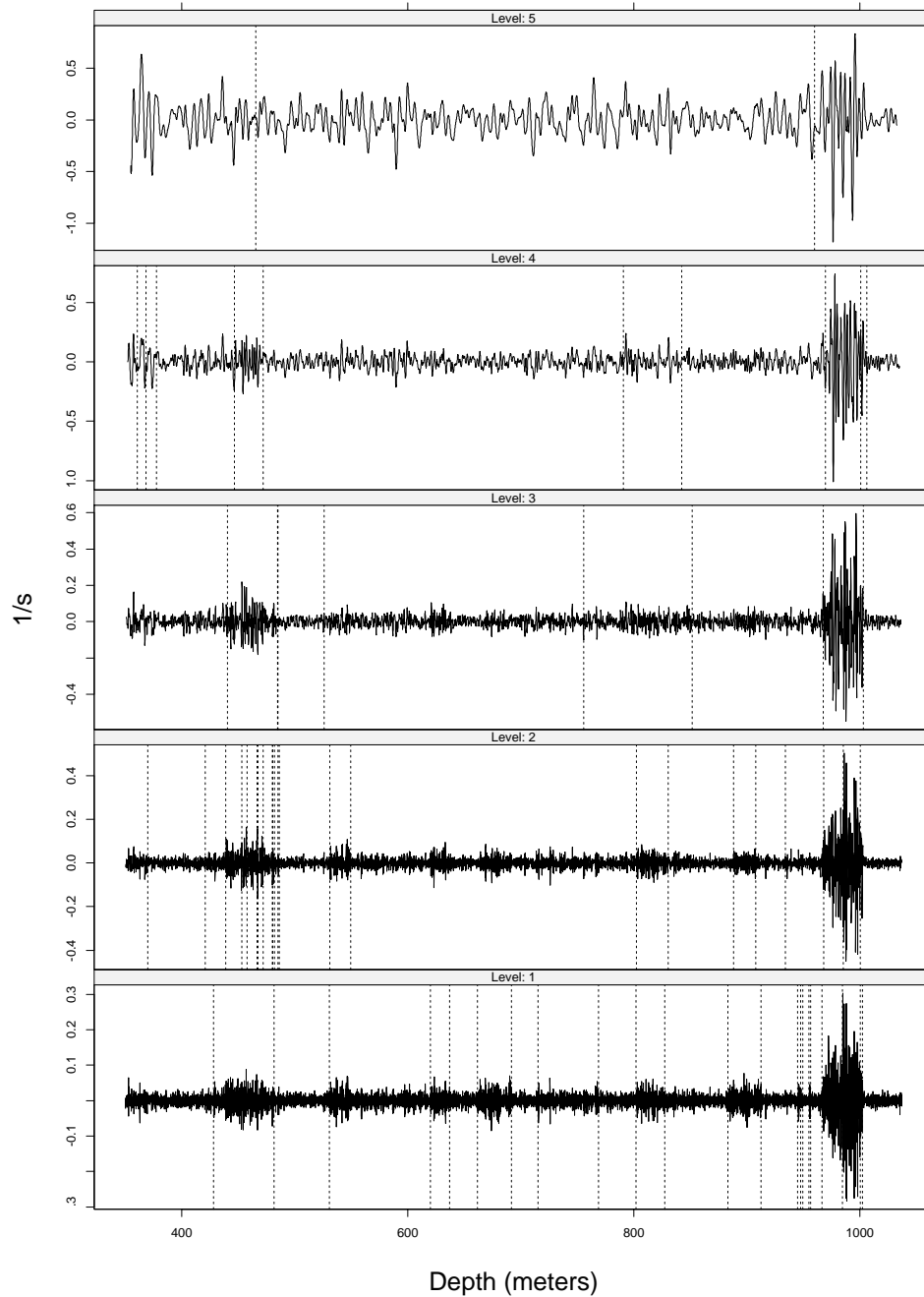
Figure 11: Estimated locations of variance change for the vertical ocean shear measurements using the D(4) wavelet filter displayed on the MODWT wavelet coefficients. Only the first five scales were found to have significant changes of variance. Asymptotic critical values were used for the hypothesis testing at the \alpha = 0.05 level of significance.
