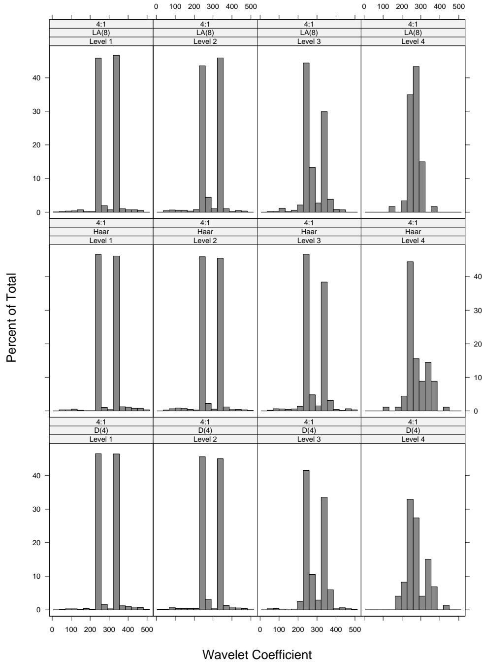
Figure 8: Same as Figure 5 with variance ratio \Delta = 4 .
