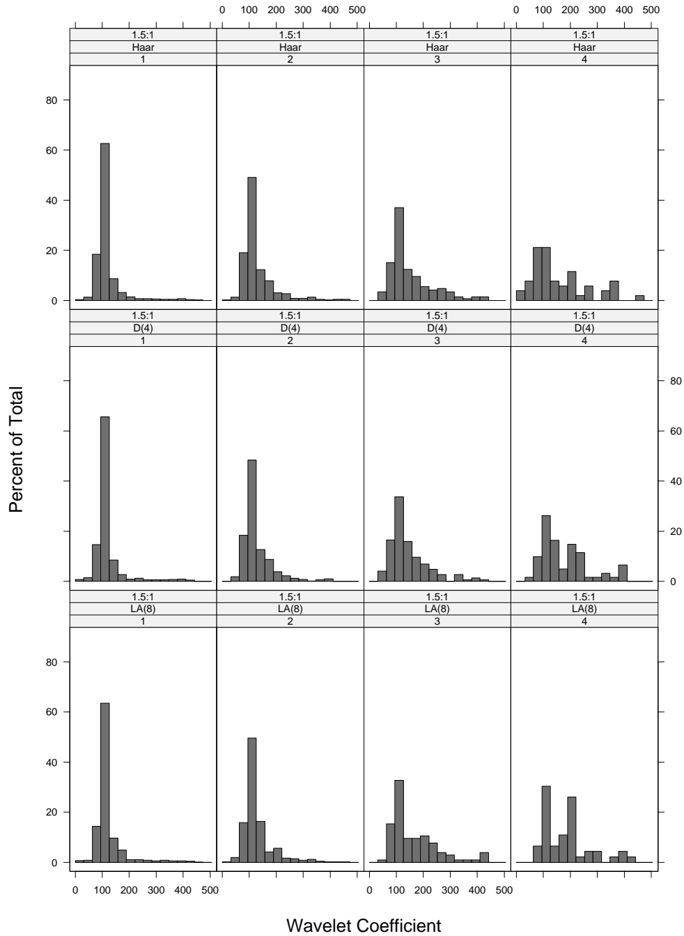
Figure 1: Estimated locations of a single variance change ( k = 100 ) for FD processes ( N = 656, d = 0.4 ) using the iterated CSS procedure and MODWT. The rows denote the various wavelet filters, the columns denote the levels of the MODWT and the variance ratio is \Delta = 1.5 .
