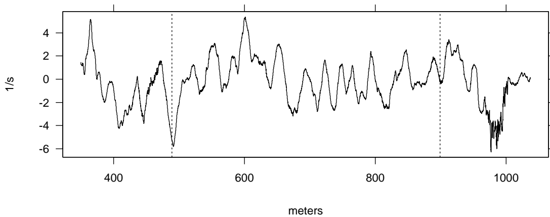
Figure 9: Plot of vertical shear measurements (inverse seconds) versus depth (meters). The two vertical lines are at 489.5m and 899.0m, and denote the roughly stationary series used by Percival and Guttorp (1994). This series can be obtained via the World Wide Web at http://lib.stat.cmu.edu/datasets/ under the title 'lmpavw'.
