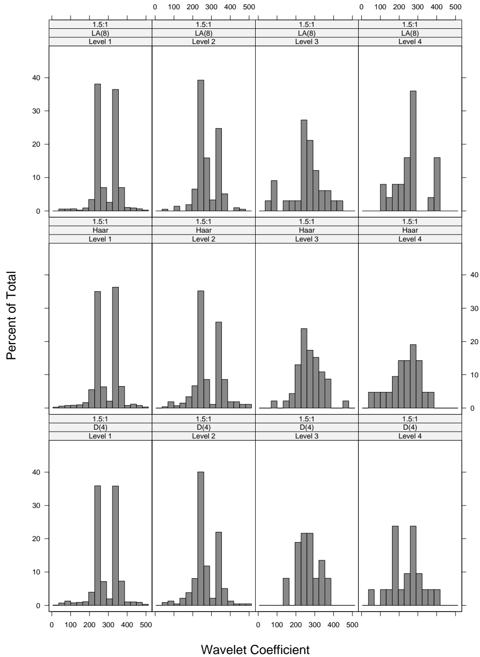
Figure 5: Estimated locations of two variance changes ( k_1 = 251, k_2 = 350 ) for FD processes ( N = 656, d = 0.4 ) using the iterated CSS procedure and MODWT. The rows denote the various wavelet filters, the columns denote the levels of the MODWT and the variance ratio is \Delta = 1.5 .
