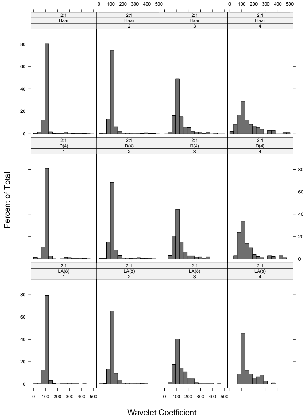
Figure 2: Same as Figure 1 with variance ratio \Delta = 2 .
