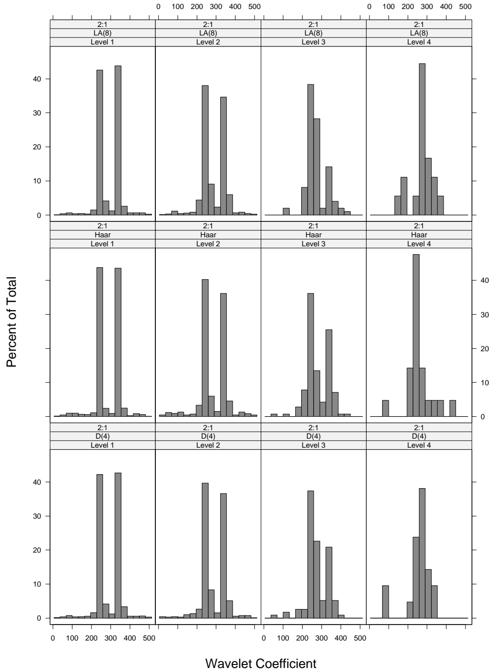
Figure 6: Same as Figure 5 with variance ratio \Delta = 2 .
