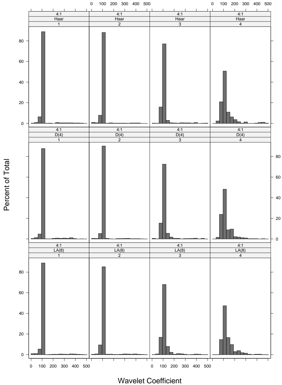
Figure 4: Same as Figure 1 with variance ratio \Delta = 4 .
