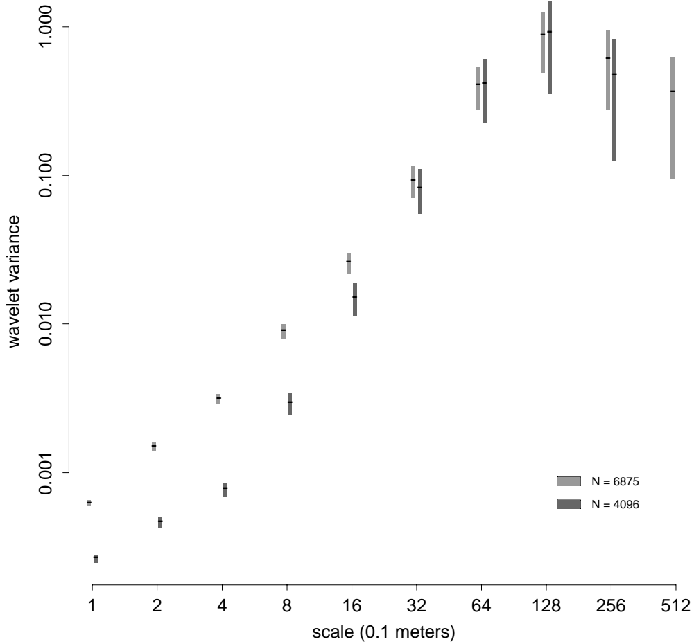
Figure 10: Estimated wavelet variance of the vertical ocean shear measurements using the D(4) wavelet filter and MODWT. The light grey confidence intervals correspond to all 6875 observations, while the dark grey confidence intervals correspond to the middle 4096 observations as analyzed in Percival and Guttrop (1994).
