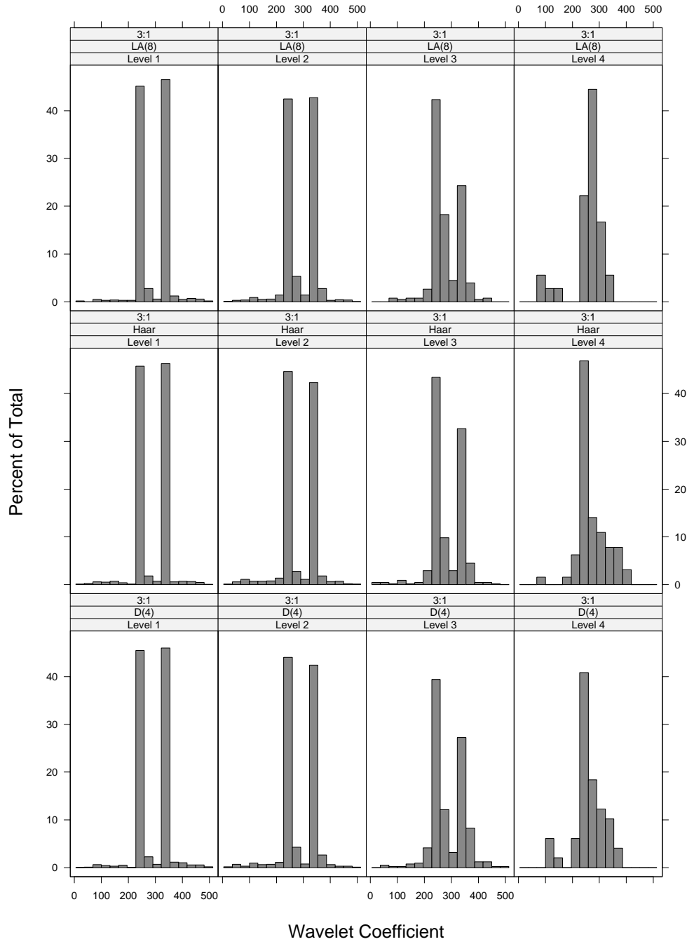
Figure 7: Same as Figure 5 with variance ratio \Delta = 3 .
